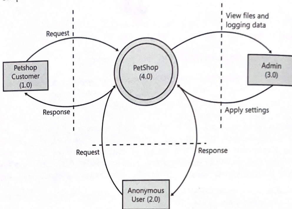
Figure 9-3 Context diagram for Pet Shop 4.0.
