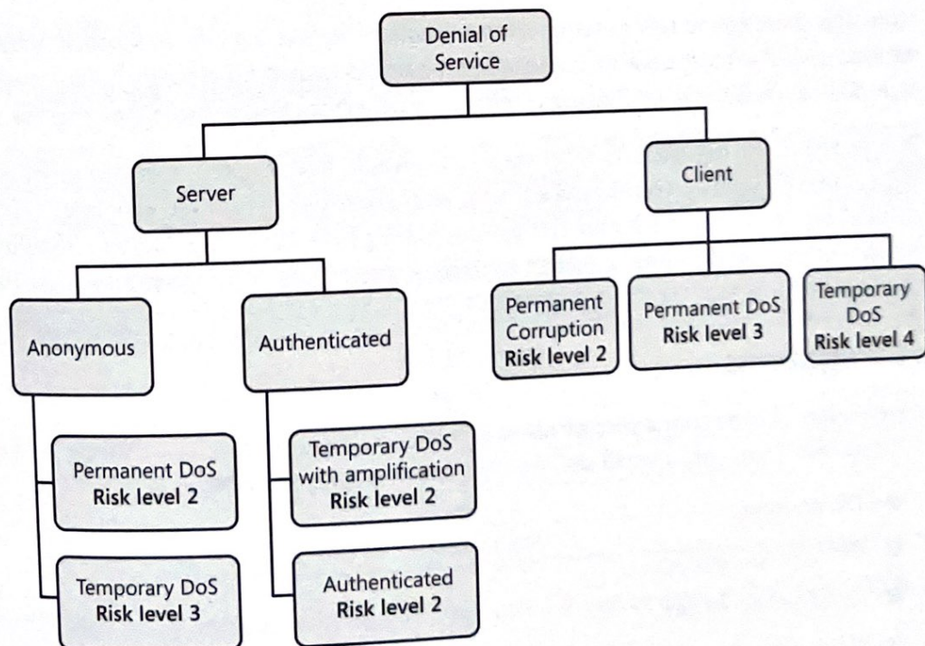
Figure 9-9 DoS threats risk ranking.
