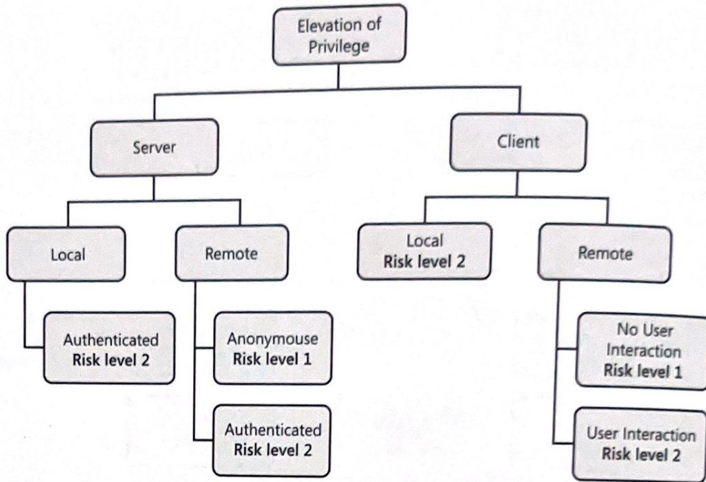
Figure 9-10 EoP threats risk ranking.
