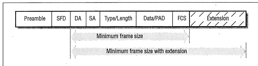
Figure 3-2. Carrier extension
