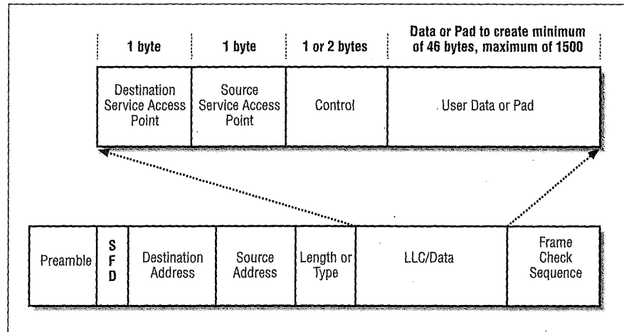
Figure 3-7. LLC PDU carried in an Ethernet frame
