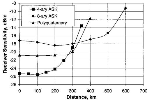
Fig. 11. Receiver sensitivity versus distance for 4-ary ASK, 8-ary ASK, and polyquaternary (seven levels) signals.
