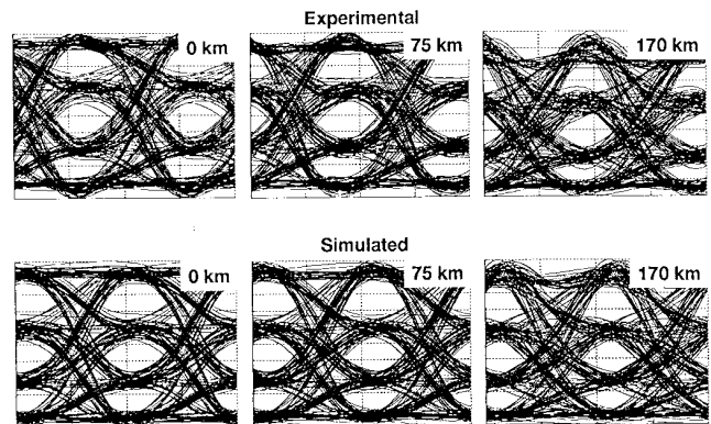
Fig. 21. Experimental and simulated eye diagrams for 10 Gb/s 4-ary ASK experiments using a III-V MZ module.
