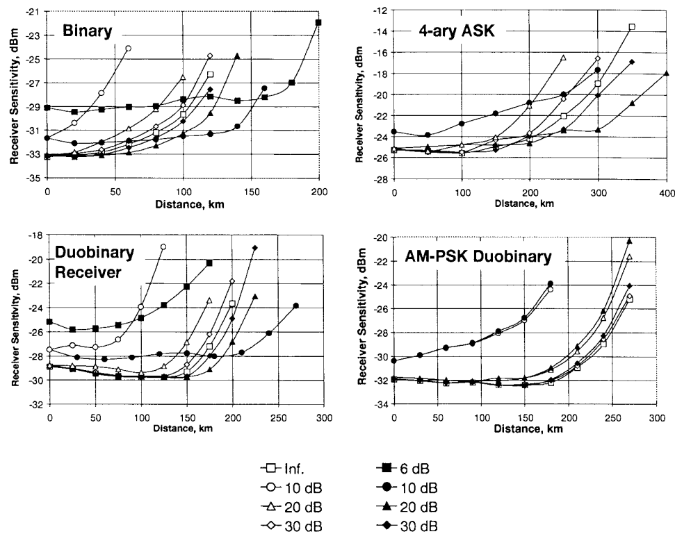
Fig. 12. Effect of residual chirp from a finite dc optical extinction ratio on various signaling schemes. Hollow markers with finite extinction ratio denote positive residual chirp. Solid markers denote negative residual chirp.
