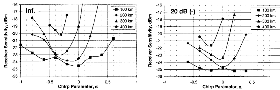
Fig. 14. Receiver sensitivity versus chirp parameter for a 4-ary ASK system using an external modulator with an ideal and 20 dB dc extinction ratio.
