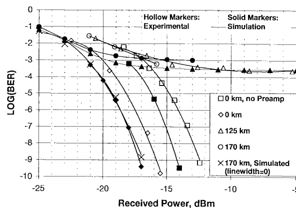
Fig. 18. BER versus received optical power for 4-ary ASK experiments using a III-V MZ module.
