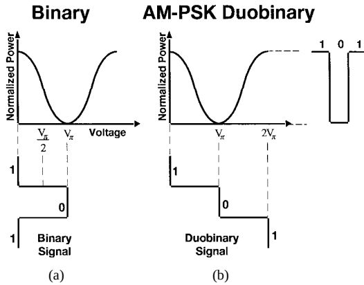
Fig. 2. (a) MZ bias and drive condition for generating a conventional binary, intensity-modulated signal and (b) an optical AM-PSK duobinary signal.
