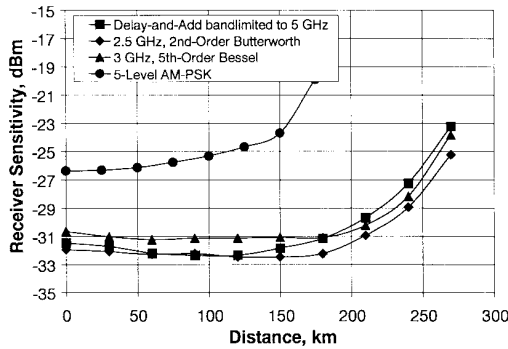
Fig. 9. Receiver sensitivity versus distance for AM-PSK polybinary signals using various duobinary filters at the transmitter. The delay-and-add filter was bandlimited by a 5-GHz, twelfth-order Butterworth low-pass filter.
