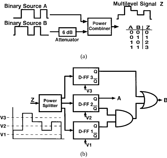
Fig. 3. (a) Multilevel symbol generator and (b) multilevel decoder.
