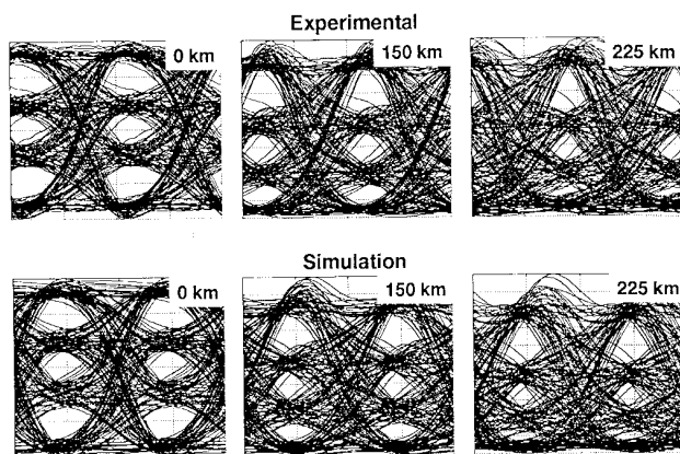
Fig. 23. Experimental and simulated eye diagrams for 10 Gb/s 4-ary ASK experiments using a LiNbO 3 MZ modulator.
