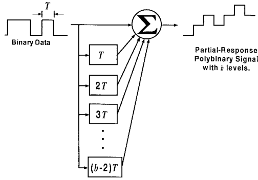
Fig. 1. Filter for generating a polybinary signal.
