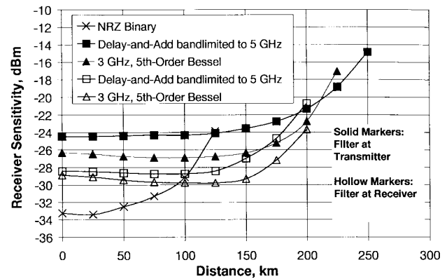
Fig. 7. Receiver sensitivity versus distance for an NRZ binary signal and for systems employing a duobinary filter at the transmitter or receiver. Delay-and-add filters were bandlimited using a 5-GHz, twelfth-order Butterworth low-pass filter.
