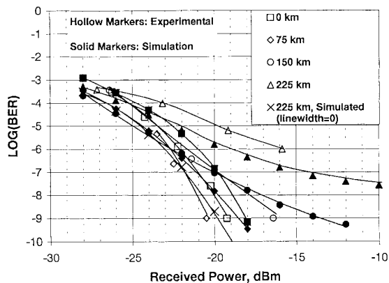
Fig. 22. BER versus received optical power for experiments using a dual-drive LiNbO 3 MZ and a narrow-linewidth laser.
