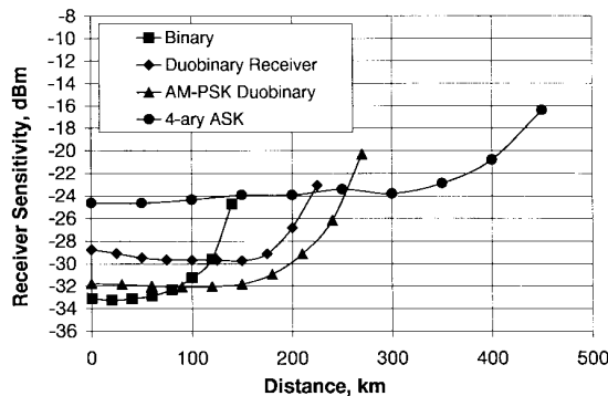
Fig. 15. Receiver sensitivity versus distance for various signaling schemes.
