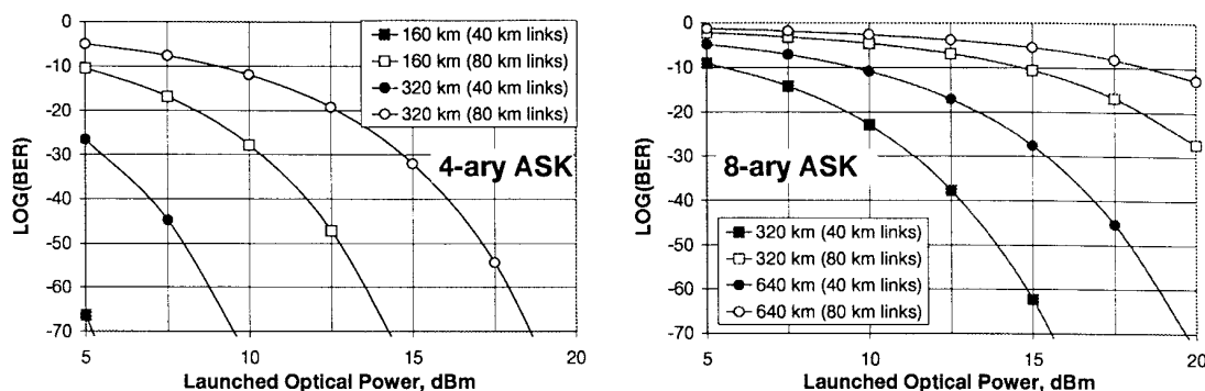
Fig. 17. BER versus launched optical power for 4-ary ASK and 8-ary ASK signals.
