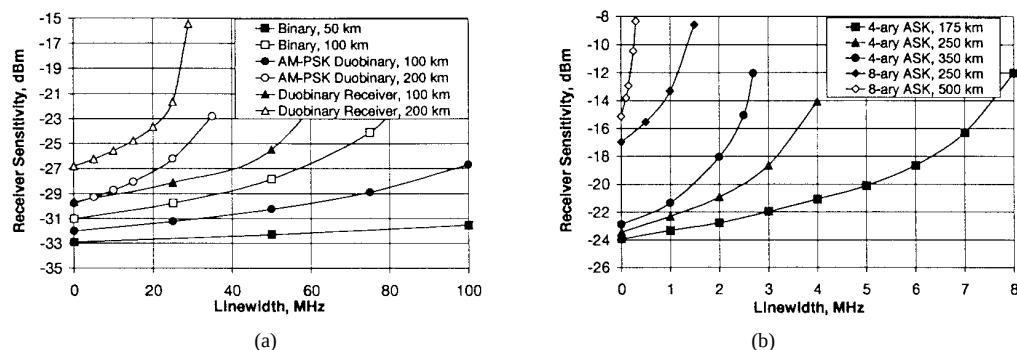
Fig. 16. Receiver sensitivity versus source linewidth: (a) binary and duobinary systems and (b) M -ary ASK systems.
