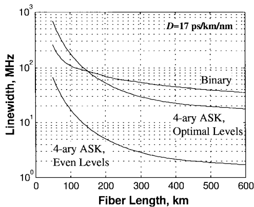
Fig. 6. Linewidth that will produce a 10^{-14} BER floor due to PM-AM RIN noise for 10 Gb/s transmission.
