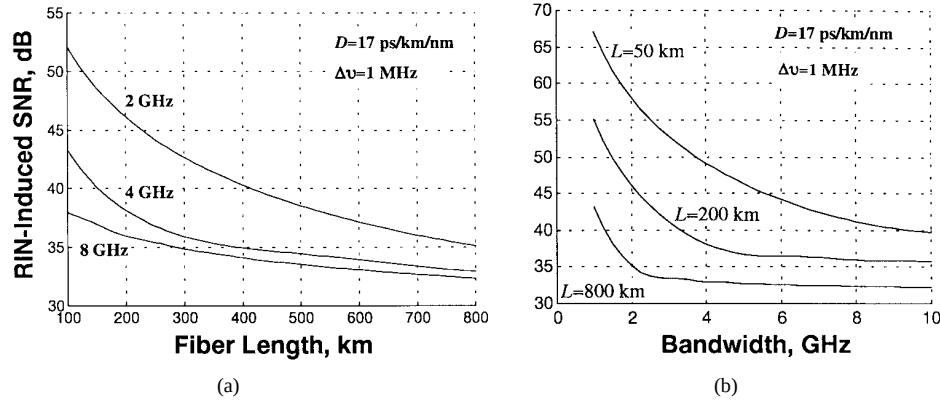
Fig. 5. (a) PM-AM RIN-induced SNR for various receiver bandwidths versus fiber length and (b) for various fiber lengths versus receiver bandwidth.
