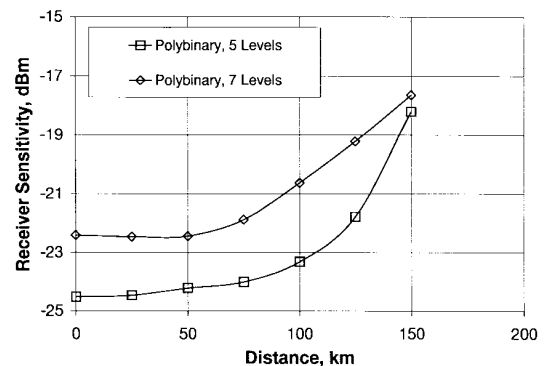
Fig. 8. Receiver sensitivity versus distance for five- and seven-level polybinary signals.
