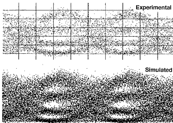
Fig. 20. Experimental and simulated eye diagrams for a 4-ary ASK signal transmitted over 170 km.
