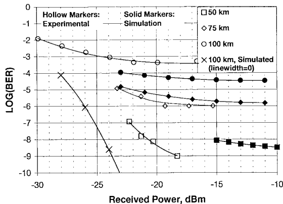
Fig. 19. BER versus received optical power for 4-ary ASK experiments using a III-V MZ module, and two EDFA's in cascade as an optical preamplifier.
