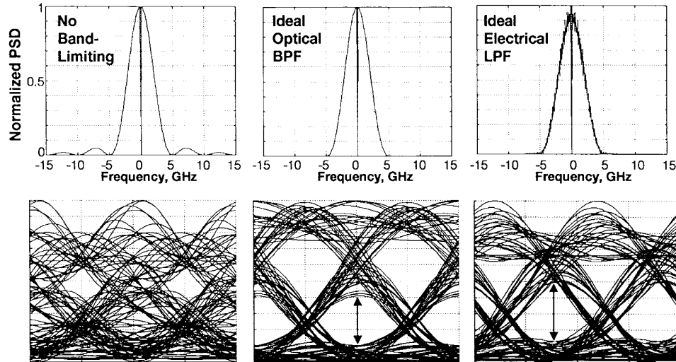
Fig. 10. PSD of the optical electric field (top) and corresponding filtered receiver eye diagrams (bottom) after transmission over 200 km for an optical AM-PSK duobinary signal.
