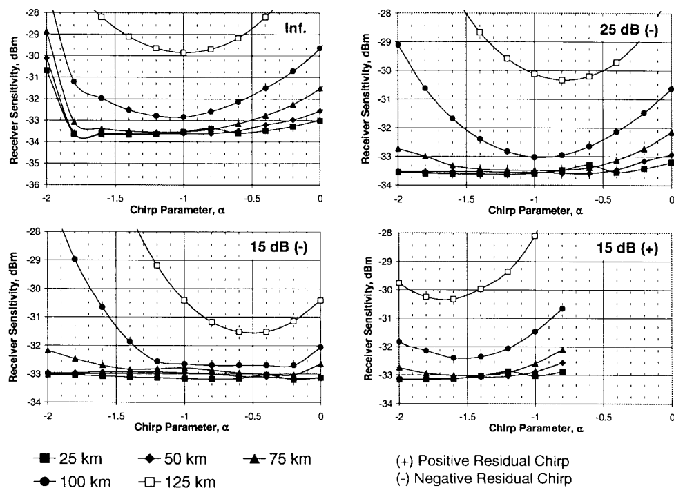
Fig. 13. Receiver sensitivity versus chirp parameter for a binary system using an external modulator with various dc extinction ratios and residual chirp polarity.
