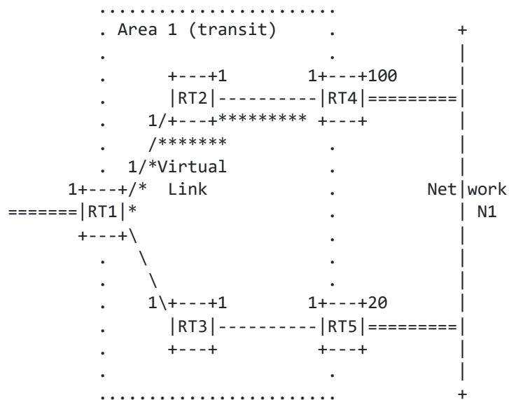
Figure 17: Routing through transit areas
