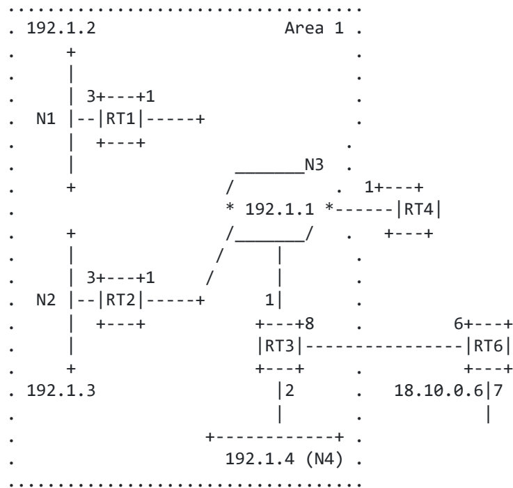
Figure 15: Area 1 with IP addresses shown
