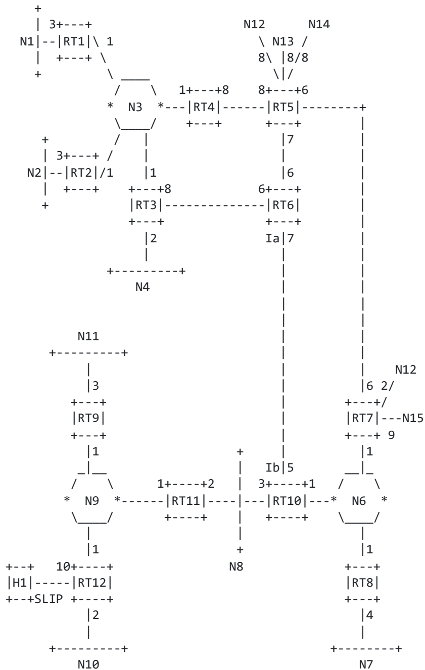
Figure 2: A sample Autonomous System
