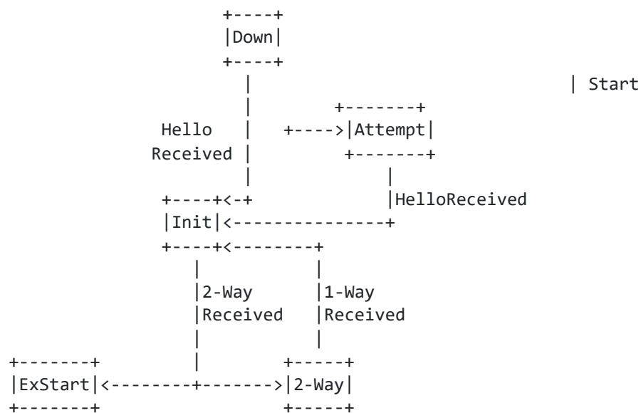
Figure 12: Neighbor state changes (Hello Protocol)
