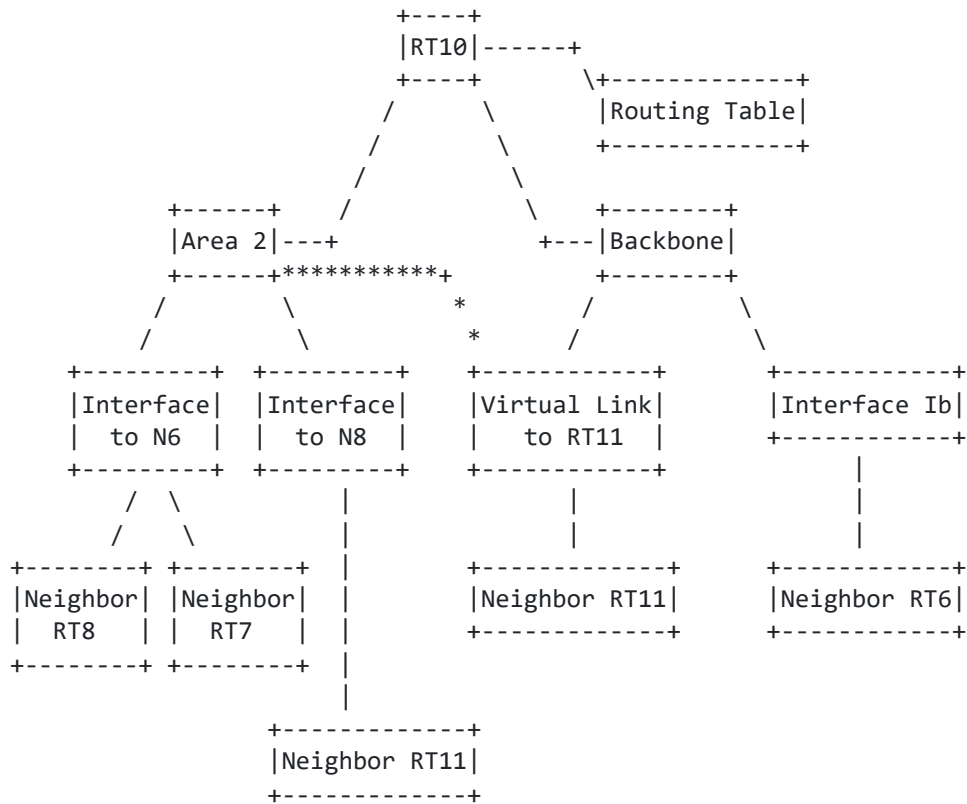
Figure 9: Router RT10's Data structures
