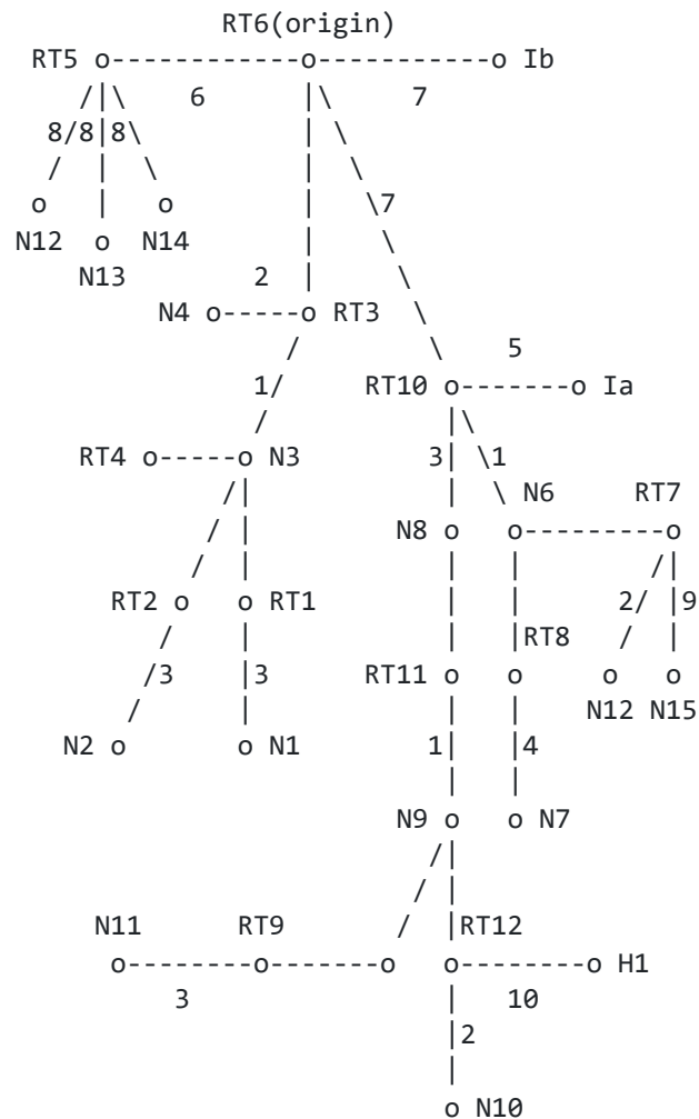
Figure 5: The SPF tree for Router RT6
