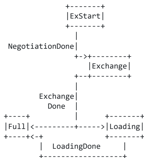
Figure 13: Neighbor state changes (Database Exchange)
