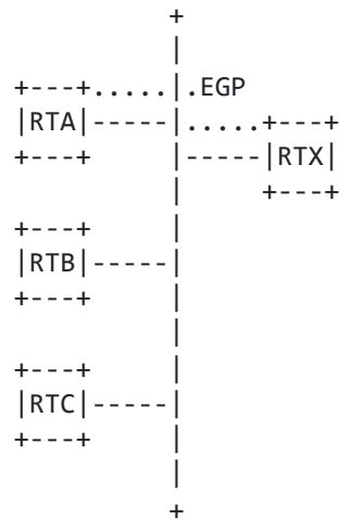
Figure 16: Forwarding address example
