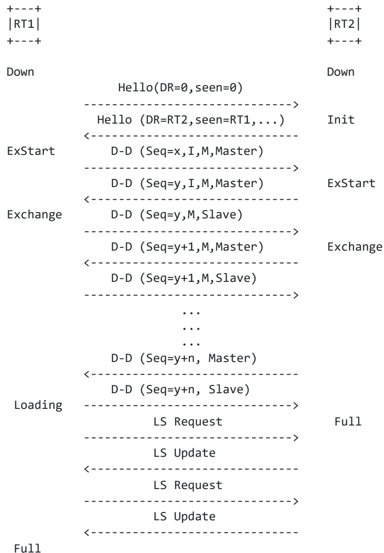
Figure 14: An adjacency bring-up example
