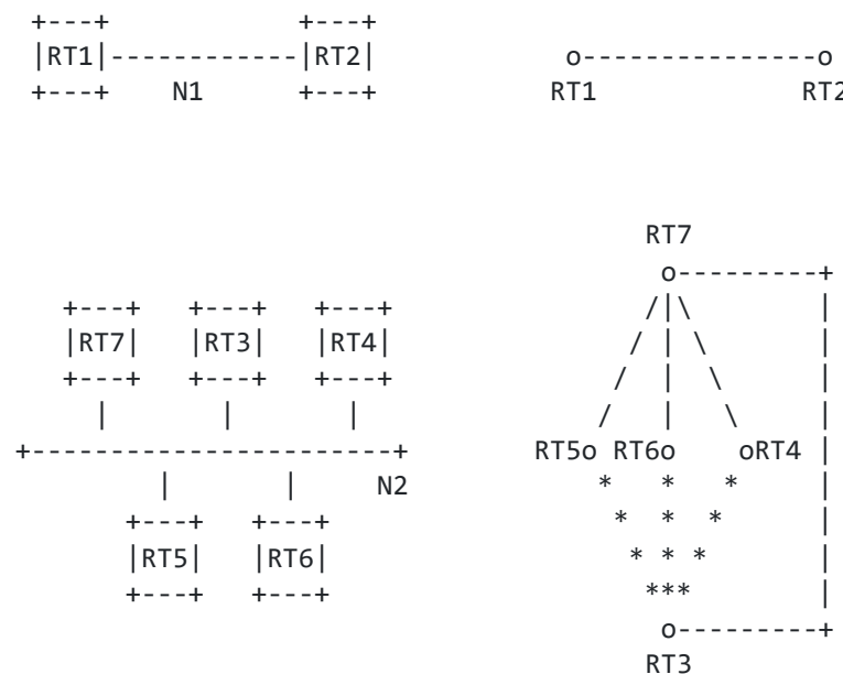
Figure 10: The graph of adjacencies
