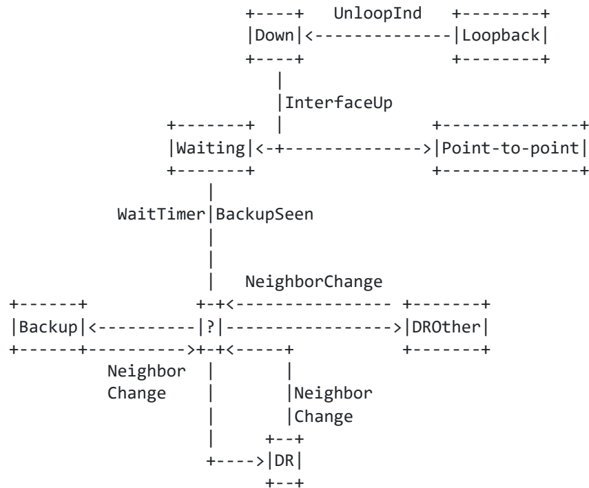
Figure 11: Interface State changes
