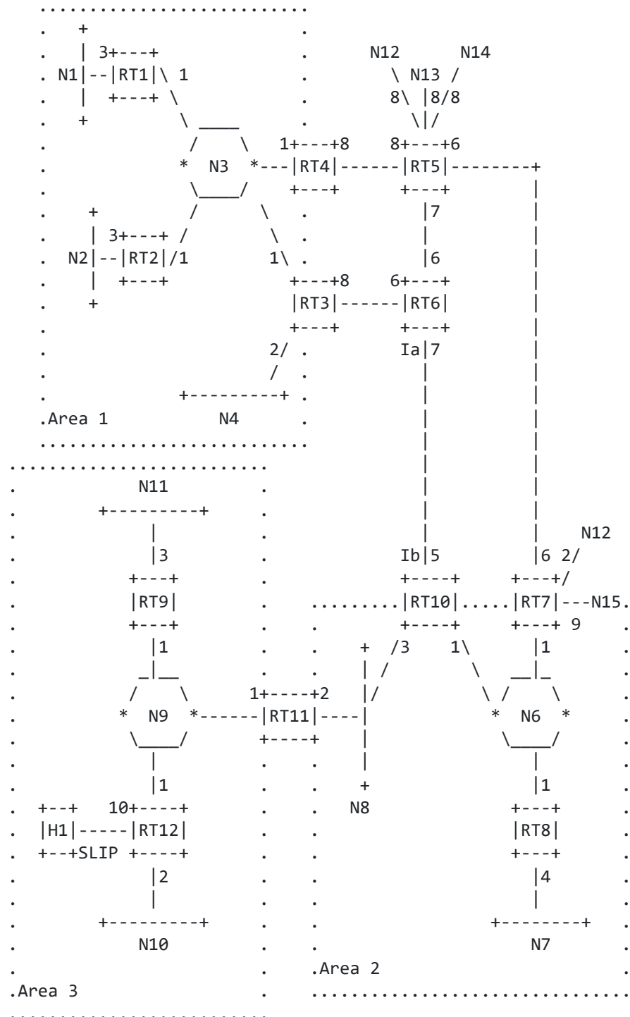
Figure 6: A sample OSPF area configuration
