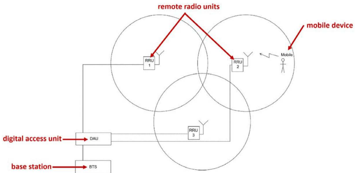
Figure 4 Indoor Localization System of GSM and LTE
