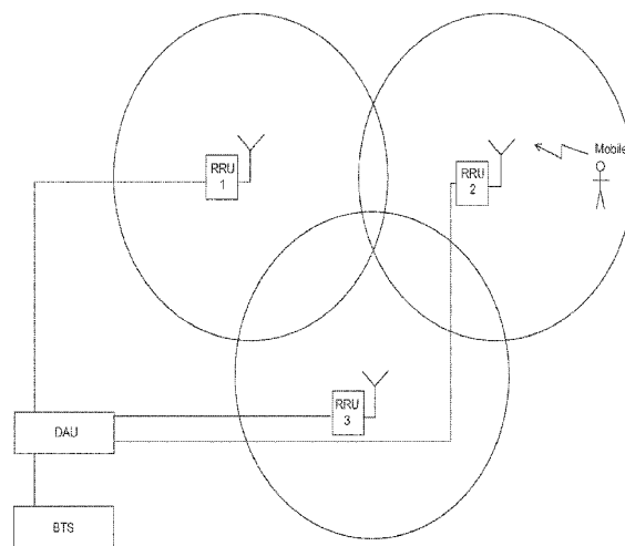
Indoor Localization System of GSM and LTE
