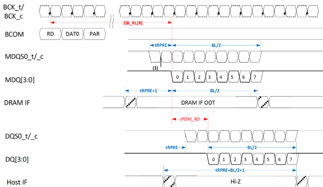
Figure 3 — READ Timing
