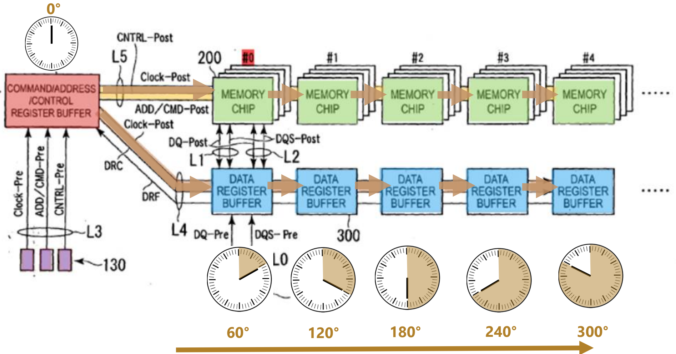
Control/Clock (Horizontal) Flight Time Delays (slower clock speed)
