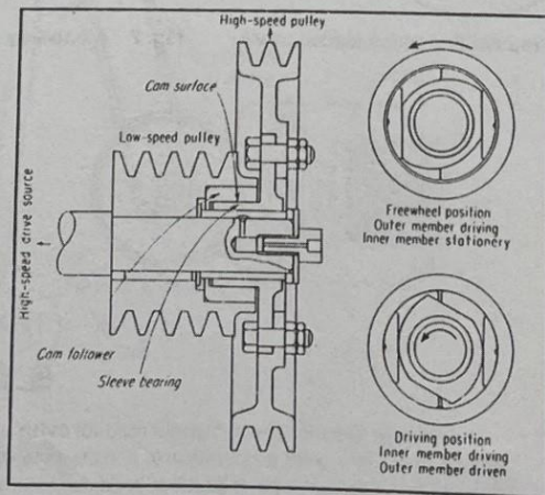
Two-speed operation is provided by the new cam clutch
