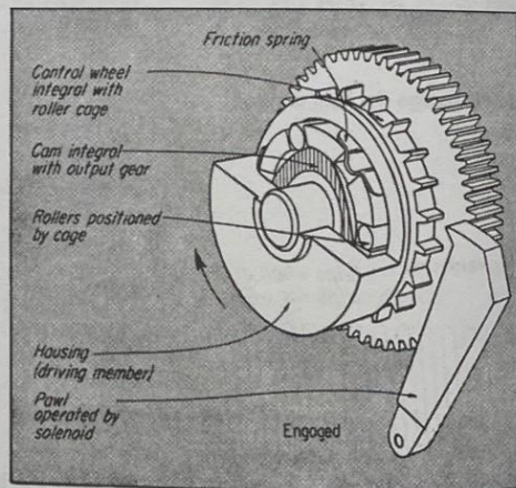
A positive drive is provided by this British roller clutch.
