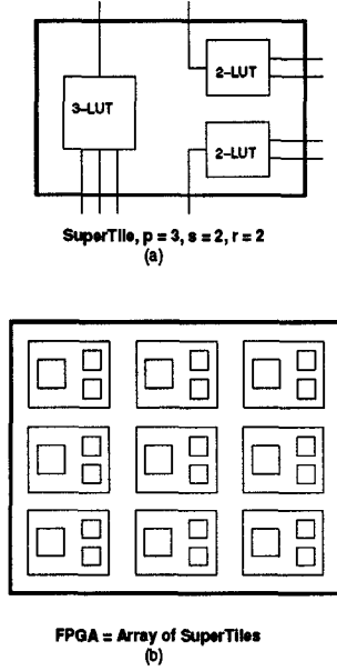
Figure 2: Example Supertile and Heterogeneous FPGA
