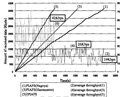
Figure 11: Results of PHS experiments.
