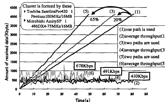
Figure 9: Results of Wireless LAN experiments.
