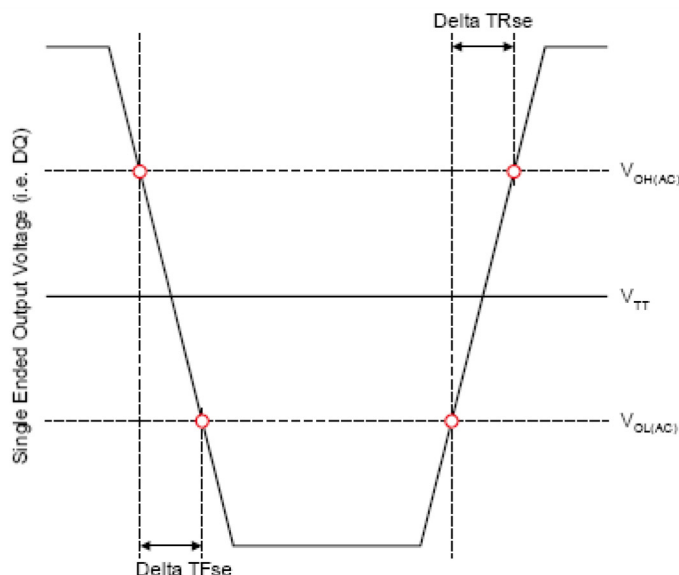
Figure 95 — Single Ended Output Slew Rate Definition
