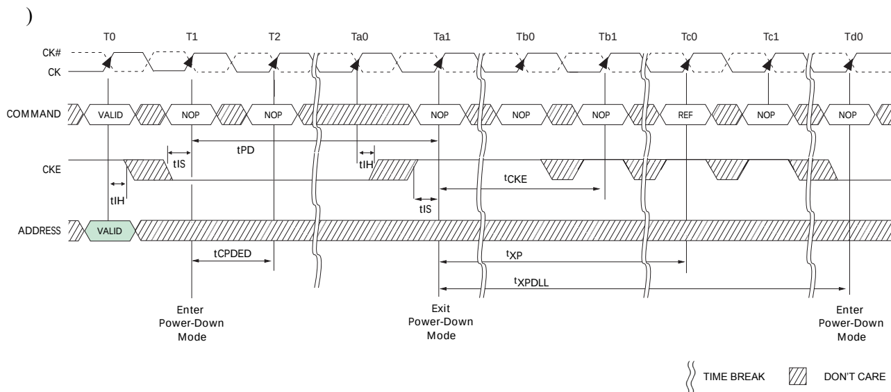
Figure 73 — Power-Down Entry/Exit Clarifications - Case 2
