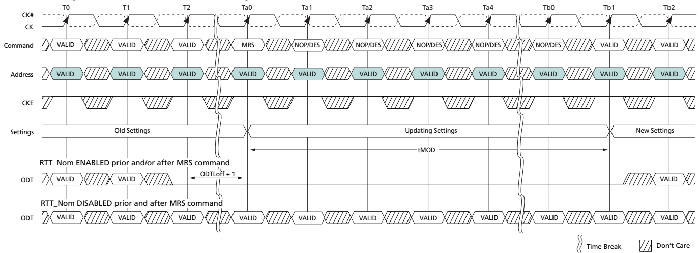
Figure 8 — t_{MOD} Timing
