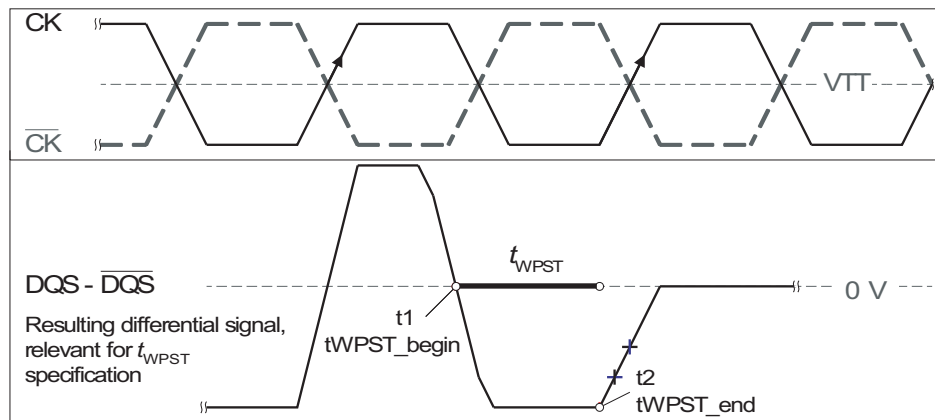
Figure 45 — Method for calculating tWPST transitions and endpoints
