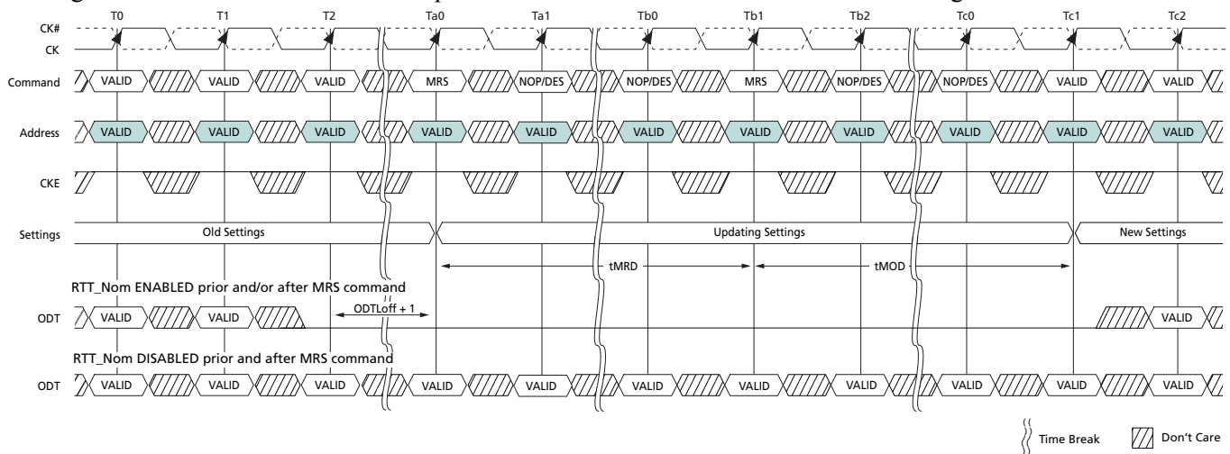
Figure 7 — t_{MRD} Timing
