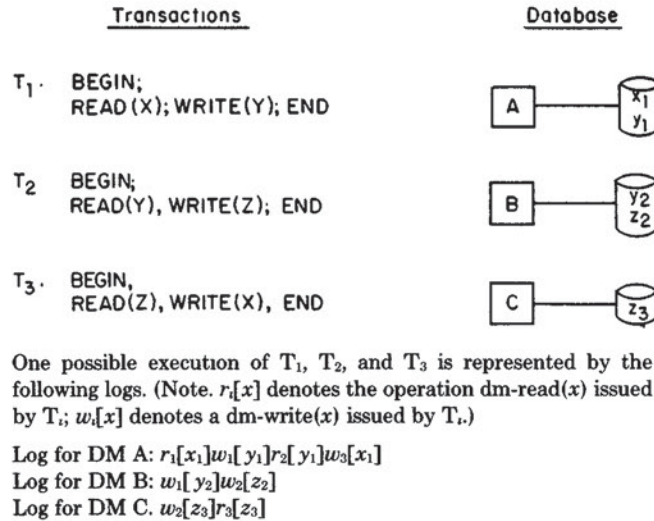
Figure 4. Modeling executions as logs.
