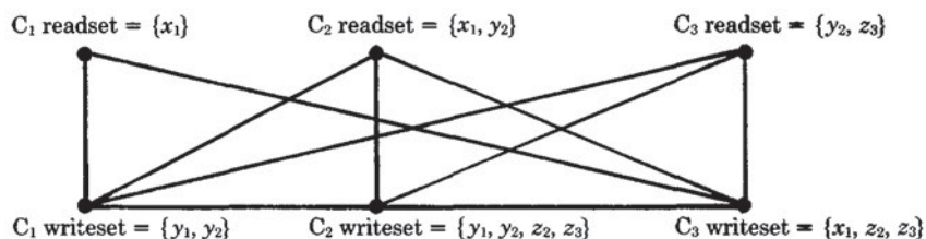
Figure 14. Conflict graph.
