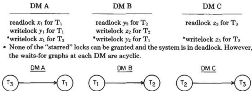
Figure 8. Multisite deadlock.
