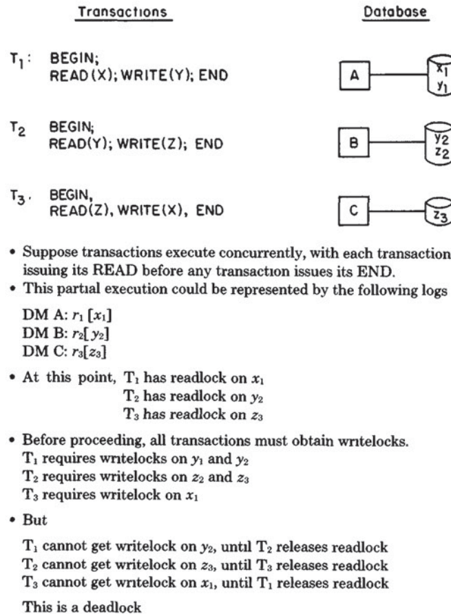
Figure 6. Deadlock.
