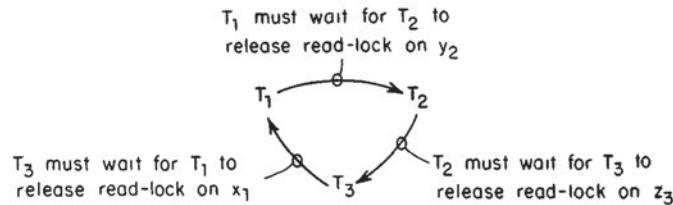
Figure 7. Waits-for graph for Figure 6.
