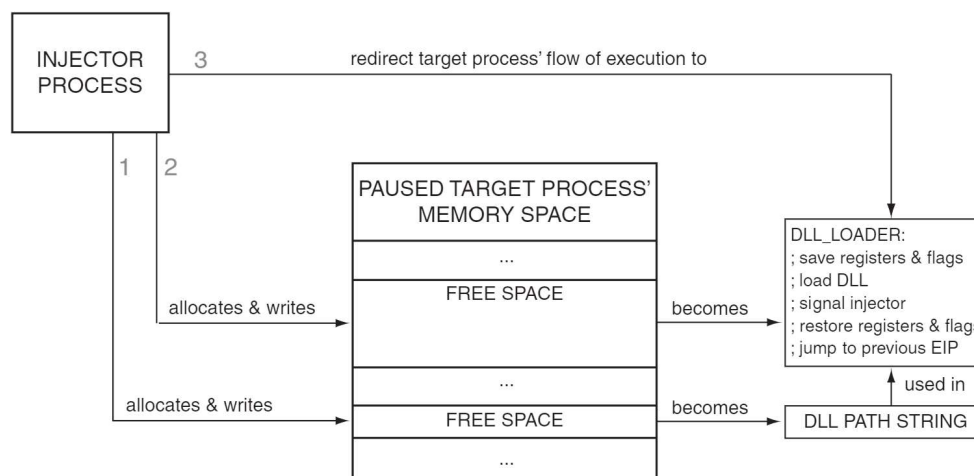
Figure 3. Debugger-aided DLL injection : An illustration of the first two steps of Debugger-aided DLL injection . First, the injector process writes a string with the path of the DLL to be injected into the target process' memory. Second, the injector process writes short low-level DLL loading code into the target process' memory, which uses the string written in the previous step. Last, the target process' flow of execution is redirected to the DLL loading code. After the DLL has been loaded, the part of the DLL loading code is overwritten so that the injector process can determine that the DLL had been loaded.
