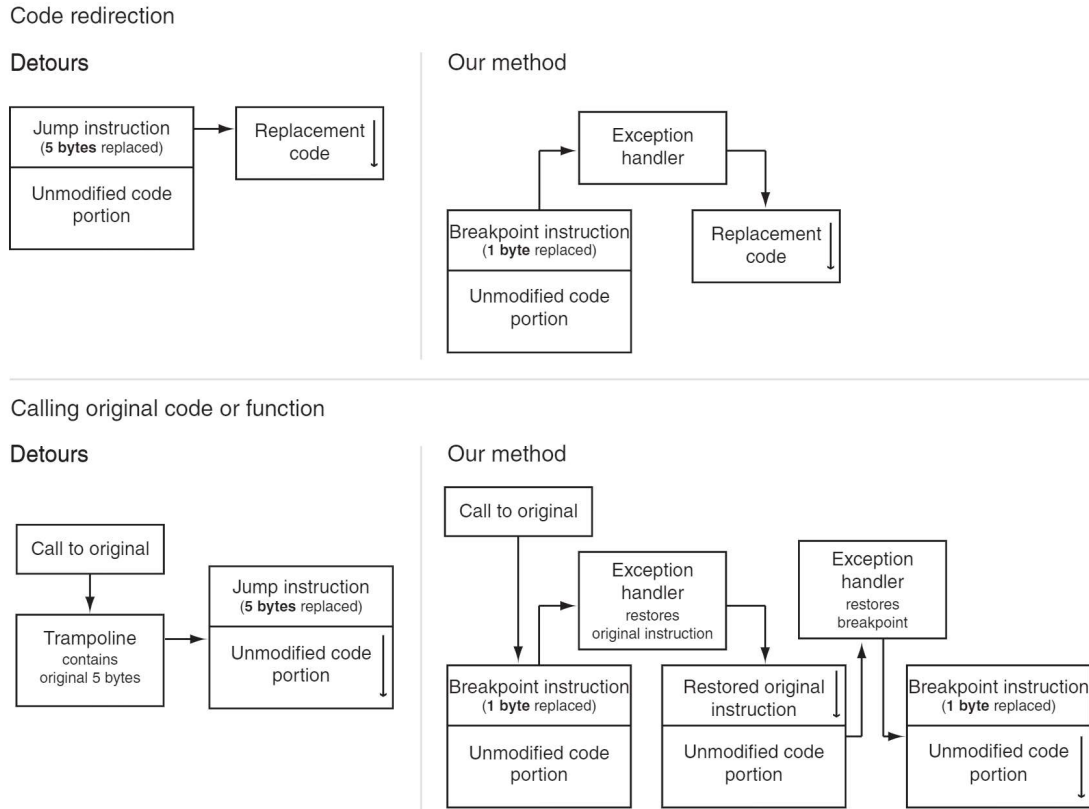
Figure 5. Comparison of Detours and SIH. Above: Comparison of how code redirection is performed. Below: Comparison of how original code is called.
