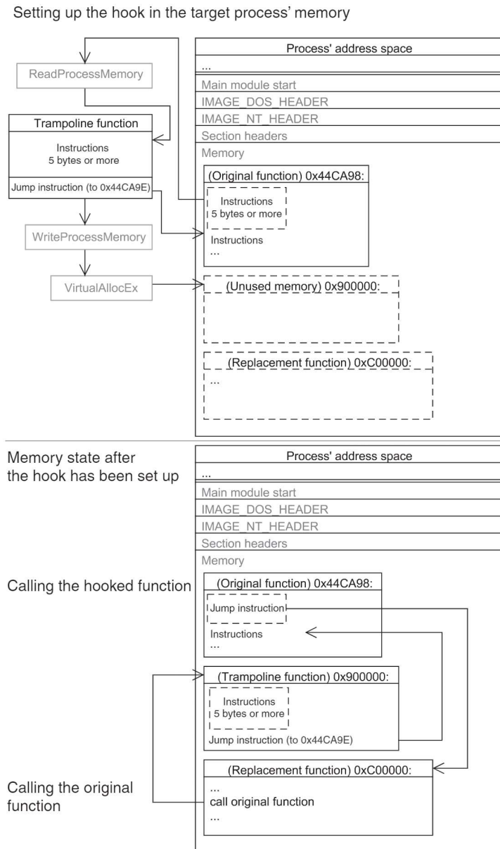
Figure 1. Detours hooking method with some technical details. Above: Creation of the trampoline function, which is created in the process' address-space. Below: The process after the applied change, and a call of the hooked function as follows. The original function contains an unconditional jump to the replacement function. The replacement function invokes the original function through the trampoline. The last instruction in the trampoline jumps to the unchanged part of the original function and proceeds with the execution of original code.
