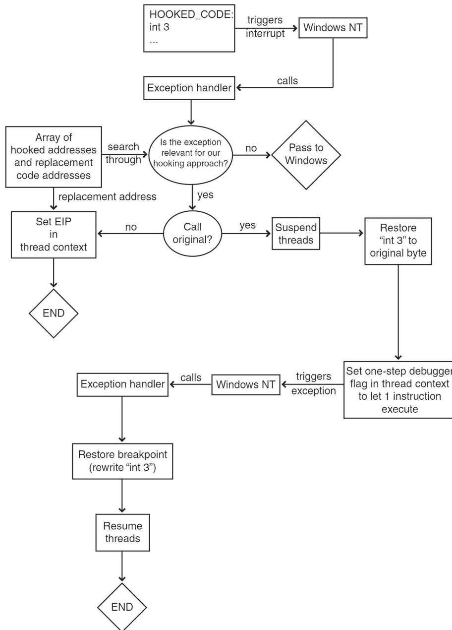
Figure 4. Single instruction hooking.
