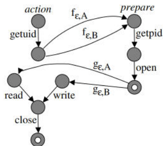
Figure 7. Dyck model.
