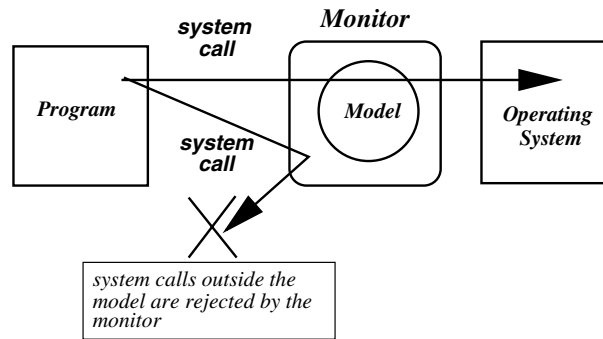
Figure 1. Architecture of a host-based intrusion detection system.
