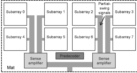
Fig. 10. Example of mat using external sensing and bus-like routing.
