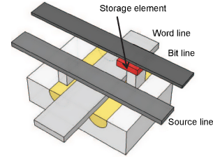
Fig. 14. Conceptual view of a MOS-accessed cell (1T1R) and its connected word line, bit line, and source line.
