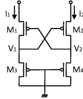
Fig. 22. Current–voltage converter modeled in NVSim.
