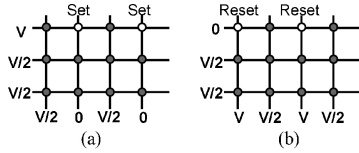
Fig. 12. Sequential write method: SET-before-RESET. (a) SET step. (b) RESET step.
