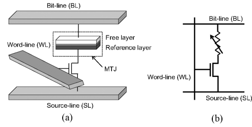
Fig. 2. Demonstration of a MRAM cell. (a) Structural view. (b) Schematic view (BL = bitline, WL = wordline, SL = sourceline).
