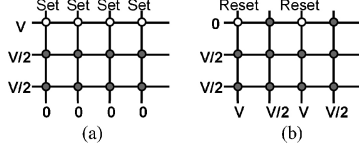
Fig. 13. Sequential write method: ERASE-before-RESET. (a) ERASE step. (b) RESET step.
