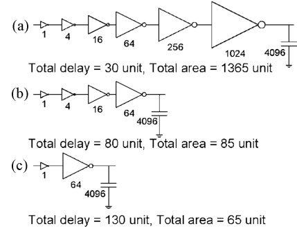
Fig. 17. Buffer designs with different transistor sizing. (a) Latency-optimized. (b) Balanced. (c) Area-optimized.
