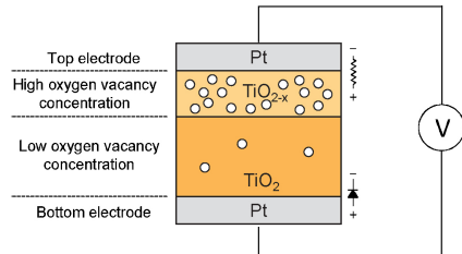
Fig. 5. Working mechanism of ReRAM cells.
