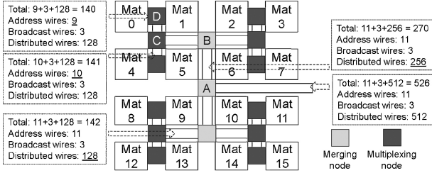
Fig. 7. Example of the wire routing in a 4 \times 4 mat organization for the data array of a 8-way 1 MB cache with 64 B cache lines.
