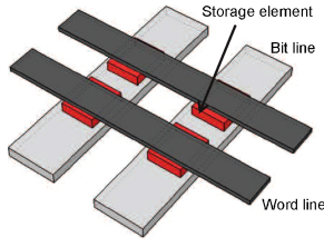
Fig. 15. Conceptual view of a cross-point cell array without diode (0T1R) and its connected word lines and bit lines.
