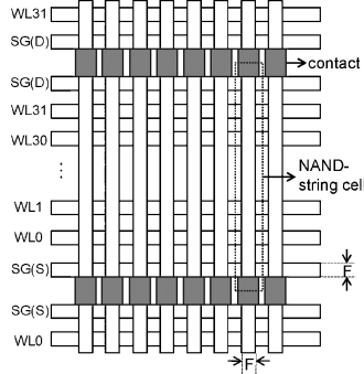
Fig. 16. Layout of the NAND-string cell modeled in NVSim.
