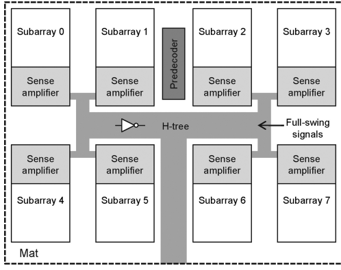
Fig. 9. Example of mat using internal sensing and H-tree routing.
