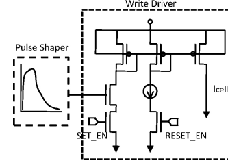
Fig. 23. Circuit schematic of the slow quench pulse shaper used in [10].
