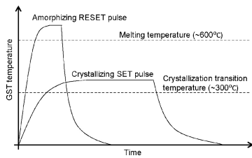
Fig. 4. Temperature–time relationship during SET and RESET operations.
