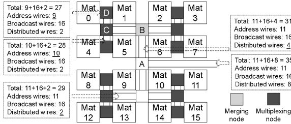
Fig. 8. Example of the wire routing in a 4 \times 4 mat organization for the tag array of a 8-way 1 MB cache with 64 B cache lines.
