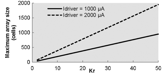
Fig. 11. Maximum subarray size versus nonlinearity and driving current.
