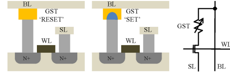
Fig. 3. Schematic view of a PCRAM cell with a MOSFET selector transistor (BL = bitline, WL = wordline, SL = sourceline).
