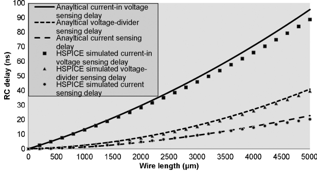
Fig. 21. Delay model verification of three sensing schemes comparing to HSPICE simulations.
