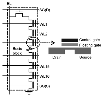
Fig. 1. Basic string block of NAND Flash, and the conceptual view of floating gate Flash memory cell (BL = bitline, WL = wordline, SG = select gate).
