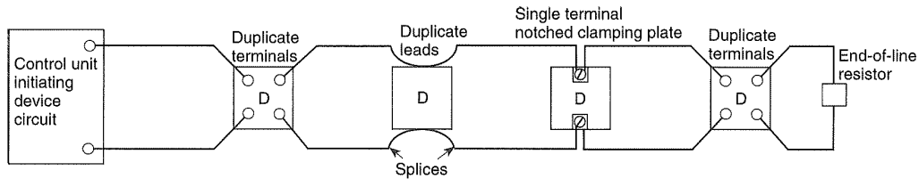
Correct wiring method — two-wire detectors
