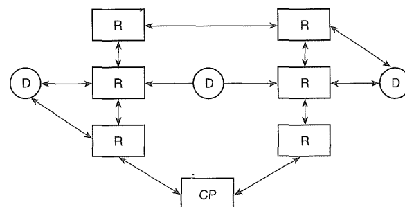
Figure A-7-2.2(b)(14)(b) Low-power radio (wireless) fire alarm system.
