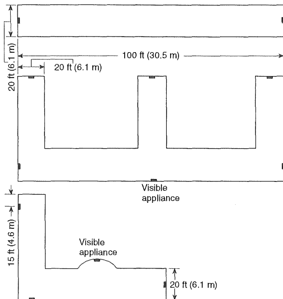
Figure A-4.4.4.2 Corridor and elevator area spacing allocation.
