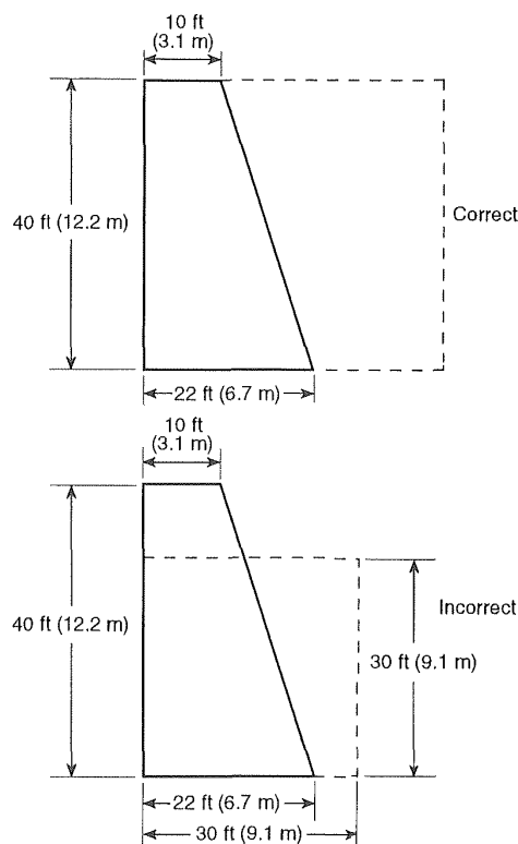
Figure A-4.4.4.1(a) Irregular area spacing.
