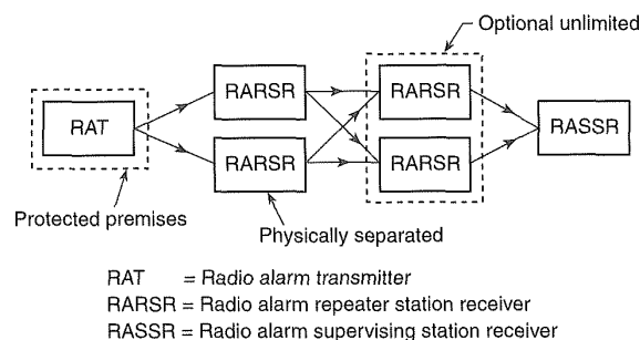
Figure A-7-2.2(b)(14)(d) One-way radio alarm system.
