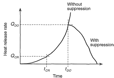
Figure B-2.3.2.2 Critical and design objective heat release rates vs. time.
