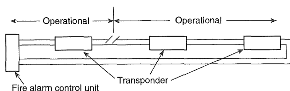
Figure A-7-2.2(b)(14)(a) Style 7.0 (Class A).
