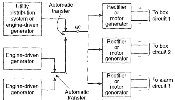
Figure A-6-7.1.8.1(c) Form 4C.
