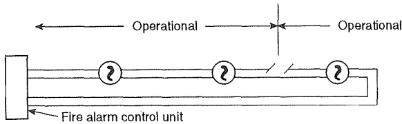
Figure A-7-2.2(a)(4) Circuit-powered (two-wire) smoke detectors for Styles D or E initiating device circuits.
