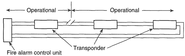
Figure A-7-2.2(b)(11) Style 5.0 (Class A).
