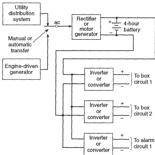
Figure A-6-7.1.8.1(b) Form 4B.
