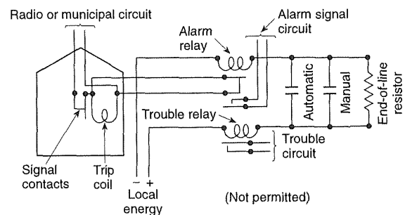
Figure A-6-16.4.1(b)(8) Shunt-type auxiliary fire alarm system.
