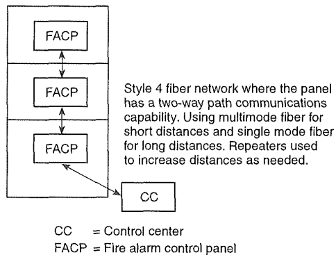
Figure A-7-2.2(b)(14)(f) Style 4 fiber network.
