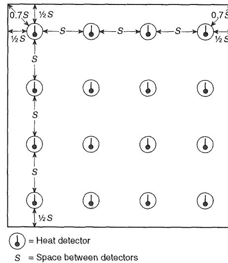
Figure A-2-2.4.1(a) Spot-type heat detectors.
