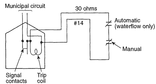
Figure A-6-16.4.1(b) Shunt-type auxiliary fire alarm system.
