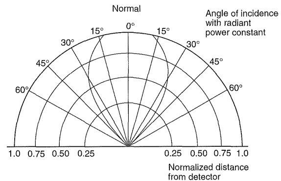
Figure A-2.4.3.2.3 Normalized sensitivity vs. angular displacement.
