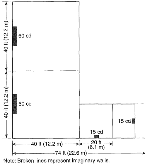
Figure A-4.4.1(c) Room spacing allocation — correct.
