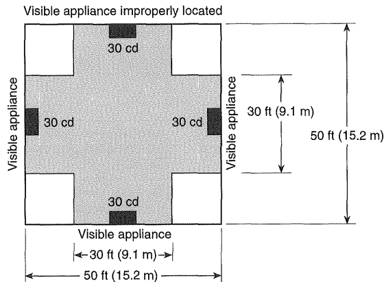
Figure A-4.4.1(d) Room spacing allocation — incorrect.
