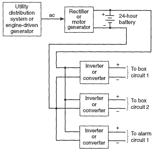
Figure A-6-7.1.8.1(a) Form 4A.
