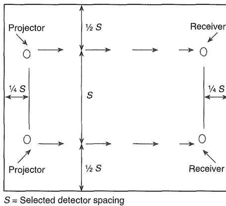
Figure A-2-3.4.5.2 Maximum distance at which ceiling-suspended light projector and receiver can be positioned from end wall is one-quarter selected spacing (S).
