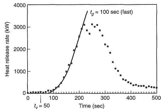
Figure B-2.3.2.1.2.8 Test 38, foam sofa.
