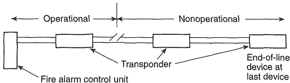
Figure A-7-2.2(b)(8) Style 3.5 (Class B).
