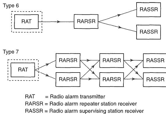
Figure A-7-2.2(b)(14)(e) One-way radio alarm system.
