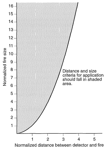
Figure A-2.4.3.1.1 Normalized fire size vs. distance.
