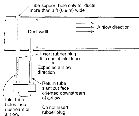
Figure A-2-10.5.2(c) Inlet tube orientation.
