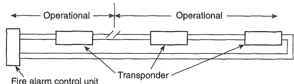
Figure A-7-2.2(b)(10) Style 4.5 (Class B).
