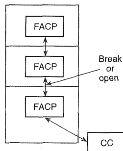
Figure A-7-2.2(b)(14)(g) Style 4 fiber network.
