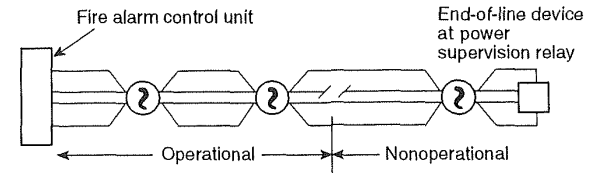
Figure A-7-2.2(a)(7) Style A, B, or C circuits with four-wire smoke detectors and an end-of-line power supervision relay.
