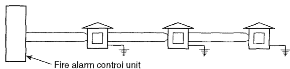
Figure A-7-2.2(a)(16) System connected to a municipal fire alarm master box circuit.
