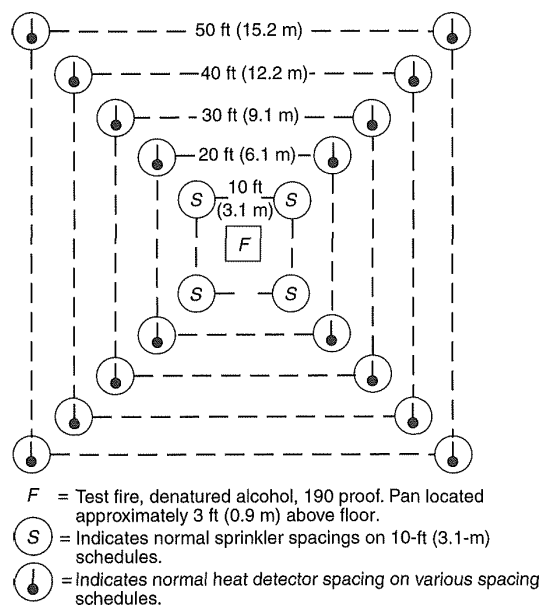
Figure A-2.2.4.1(c) Fire test layout.
