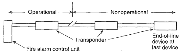
Figure A-7-2.2(b)(9) Style 4.0 (Class B).
