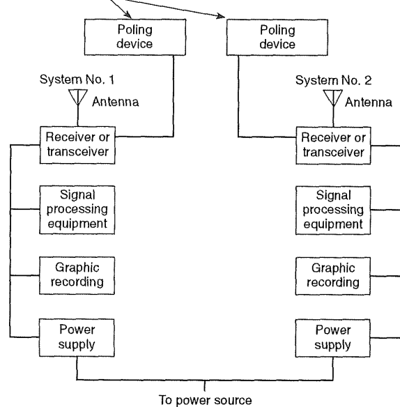
Figure A-6-14.3.1.1 Type A system receiving networks.
