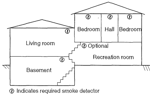
Figure A-8-1.4.1 Split level arrangement.
