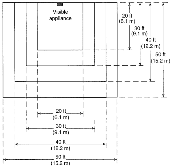
Figure 4-4.4.1.1 Room spacing for wall-mounted visible appliances.
