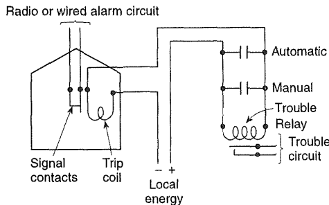
Figure A-6-16.4.1(a)(1) Local energy-type auxiliary fire alarm system.
