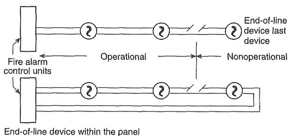
Figure A-7-2.2(a)(3) Circuit-powered (two-wire) smoke detectors for Style A, B, or C initiating device circuits.
