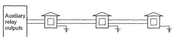
Figure A-7-2.2(a)(17) Auxiliary circuit connected to a municipal fire alarm master box.
