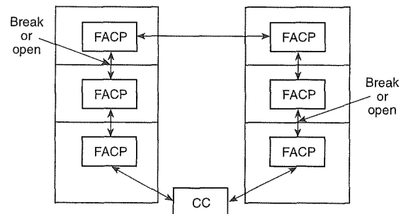
Figure A-7-2.2(b)(14)(i) Style 7 fiber network.
