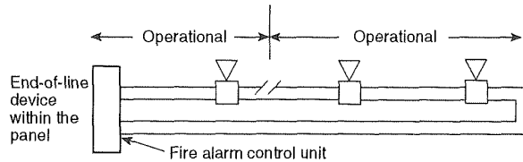
Figure A-7-2.2(a)(10) Alarm indicating appliances connected to Styles X and Z (four-wire) circuits.
