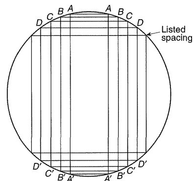
Figure A-2.2.4.1(f) Detector spacing, rectangular areas.
