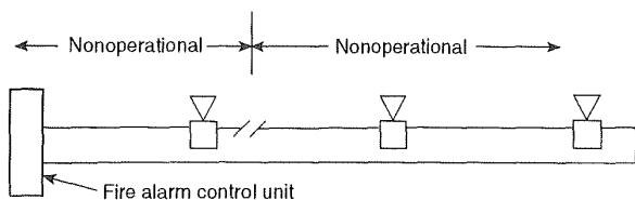
Figure A-7-2.2(a)(13) Series indicating appliance circuit.
