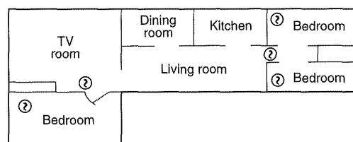
Figure A-8-1.2.1(c) A smoke detector should be located on each story.
