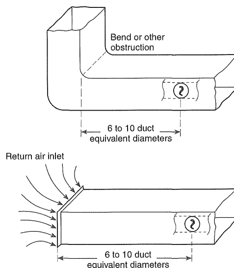
Figure A-2-10.5.2(b) Typical duct detector placement.
