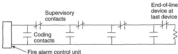
Figure A-7-2.2(b)(2) Style 0.5(a) (Class B) series.
