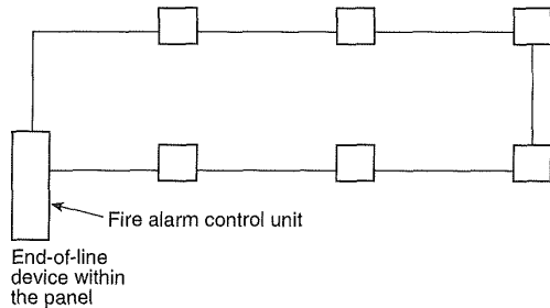
Figure A-7-2.2(b)(6) Typical McCulloh loop.
