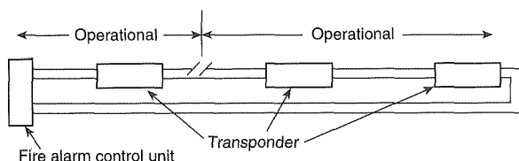
Figure A-7-2.2(b)(12) Style 6.0 (Class A).
