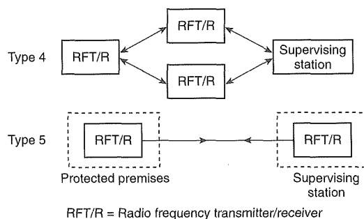
Figure A-7-2.2(b)(14)(c) Two-way RF multiplex systems.
