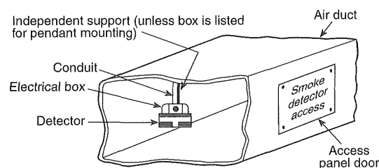
Figure A-2-10.5.2(a) Pendant-mounted air duct installation.
