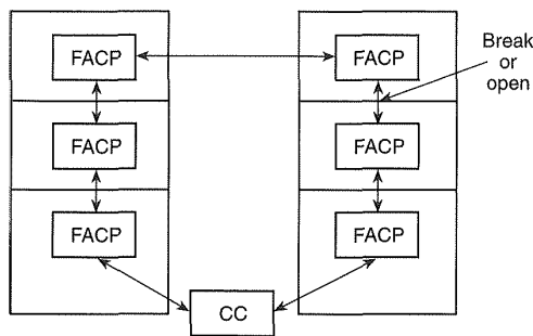
Figure A-7.2.2(b)(14)(j) Style 7 fiber network.
