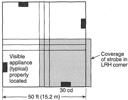
Figure A-4.4.1(d) Room spacing allocation — incorrect.
