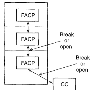
Figure A-7-2.2(b)(14)(h) Style 4 fiber network.
