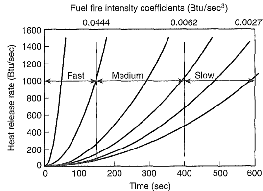
Figure B-2.3.2.3.1 Power law heat release rates.
