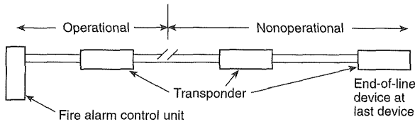
Figure A-7-2.2(b)(7) Style 3.0 (Class B).
