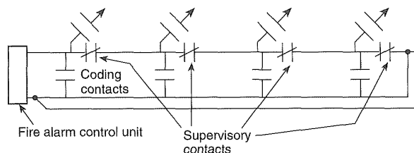
Figure A-7-2.2(b)(3) Style 0.5(b) (Class B) shunt.
