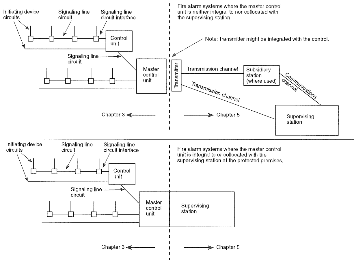
Figure 5-5.1 Division of scope.
