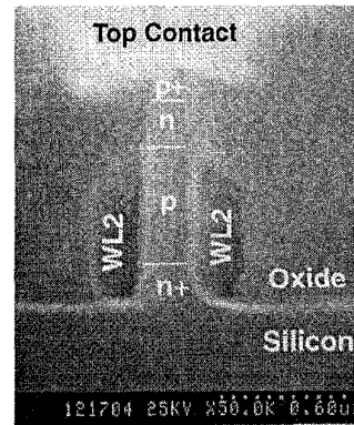
Fig. 7: Cross-sectional SEM image of a 0.2\mu\text{m} thick NDR device.
