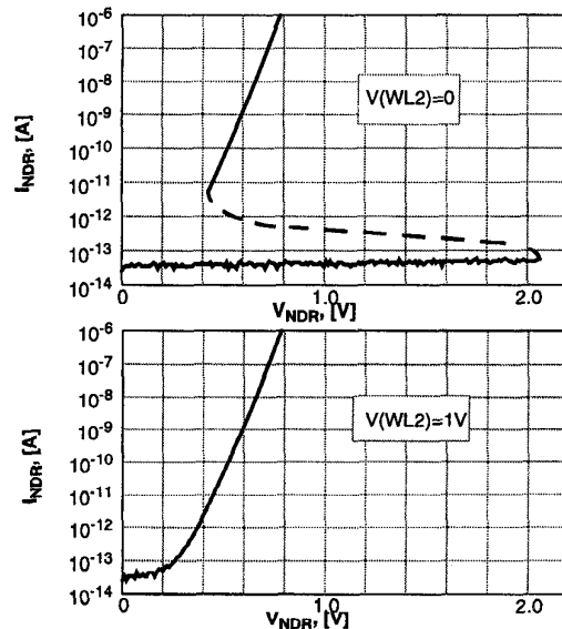
Fig. 8: Measured I-V characteristics of a typical NDR Device for various gate voltages. The holding current of the device in the standby on state is less than 10\text{pA} . The area of the device is 0.2\mu\text{m} \times 5\mu\text{m} .
