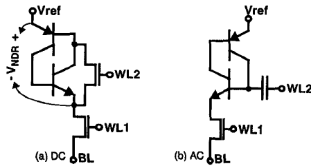
Fig. 3: DC and AC equivalent circuit models of the SRAM cell. The capacitive coupling between WL2 and the P region is used for the fast switching of the NDR device.
