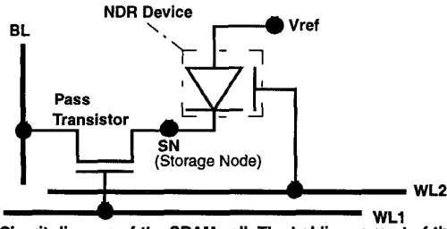
Fig. 2: Circuit diagram of the SRAM cell. The holding current of the NDR device, in the standby on state, is provided by the sub-threshold current of the pass transistor at V_{GS}=0 .
