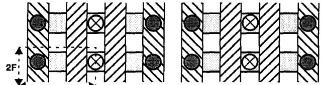
Fig. 6: Layout of the 8F^2 SRAM cell in an open bit-line architecture. WL2 is not defined in the actual layout and is formed by poly spacer etch.
