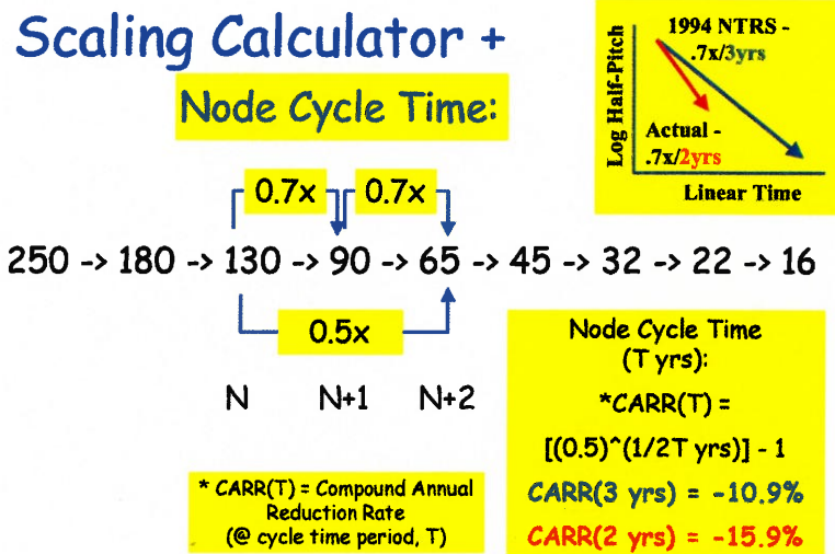
Figure 6 Scaling Calculator
