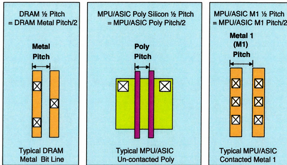
Figure 4 Definition of Metal Half Pitch
