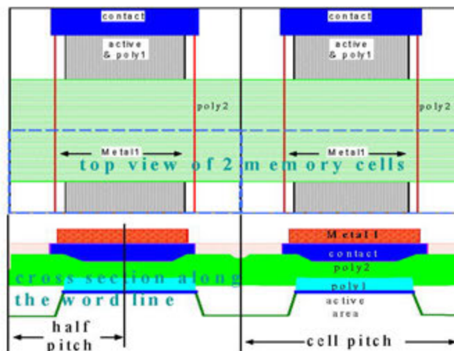
Figure 51 Minimum Feature Size of NOR Flash Memory
