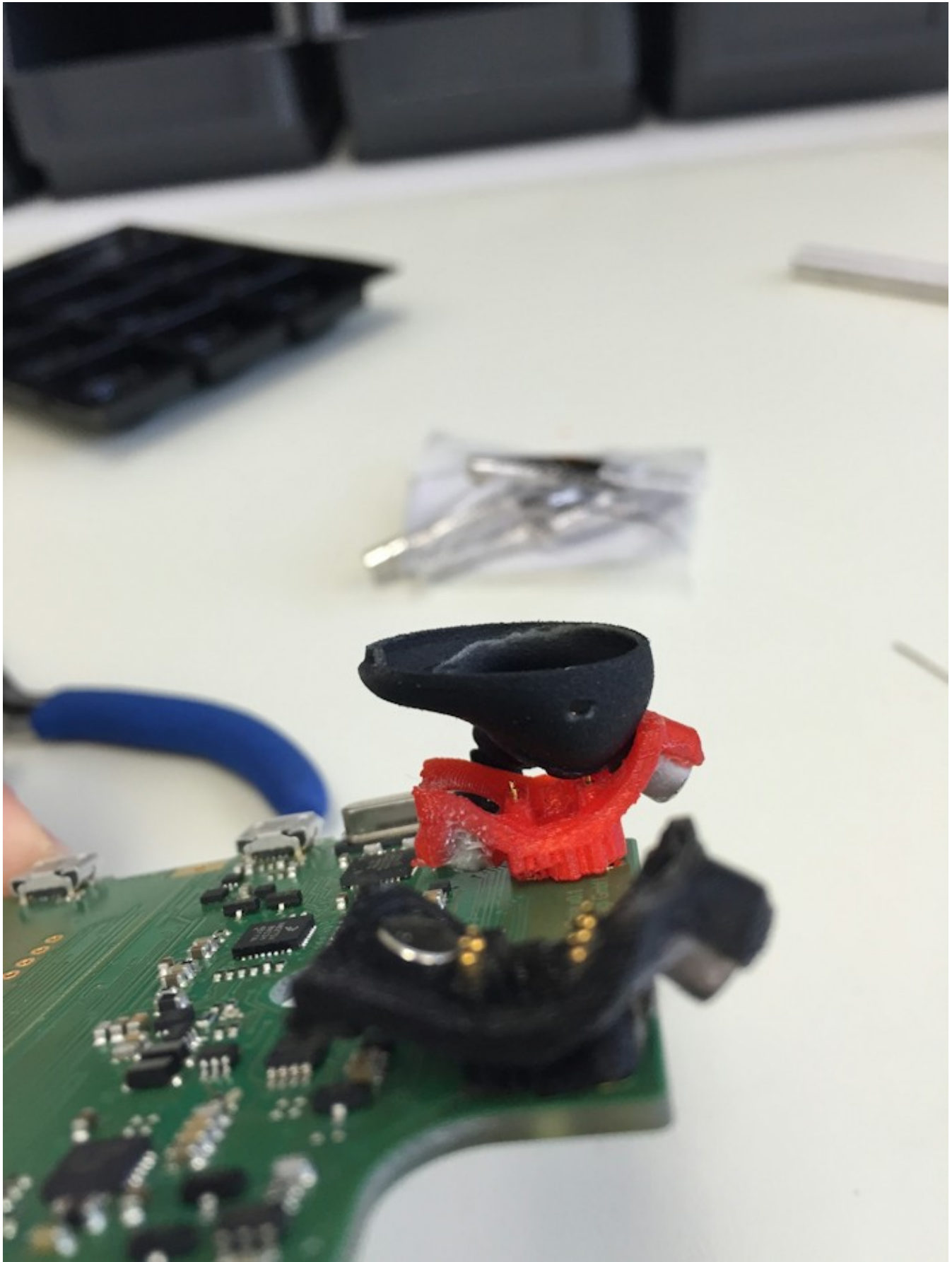
Charger electronics development board. Pogo pins are the gold plated pins.
