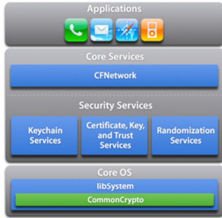
Fig. 3. iOS Architecture [27]
