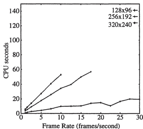
Figure 7. CPU consumption
