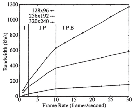
Figure 8. Network bandwidth
