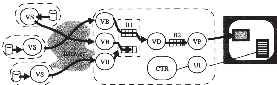
Figure 6. Concatenation
