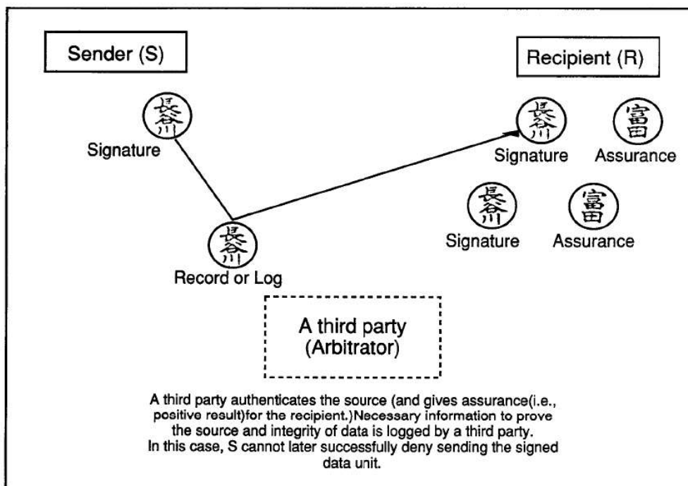
Figure 2 — Arbitrated Signature Scheme
