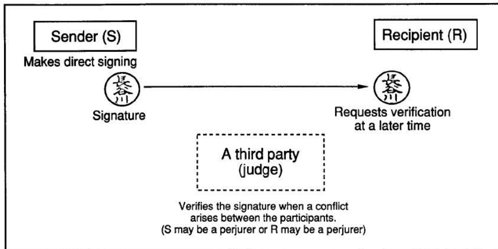
Figure 1 — Direct Signature Scheme
