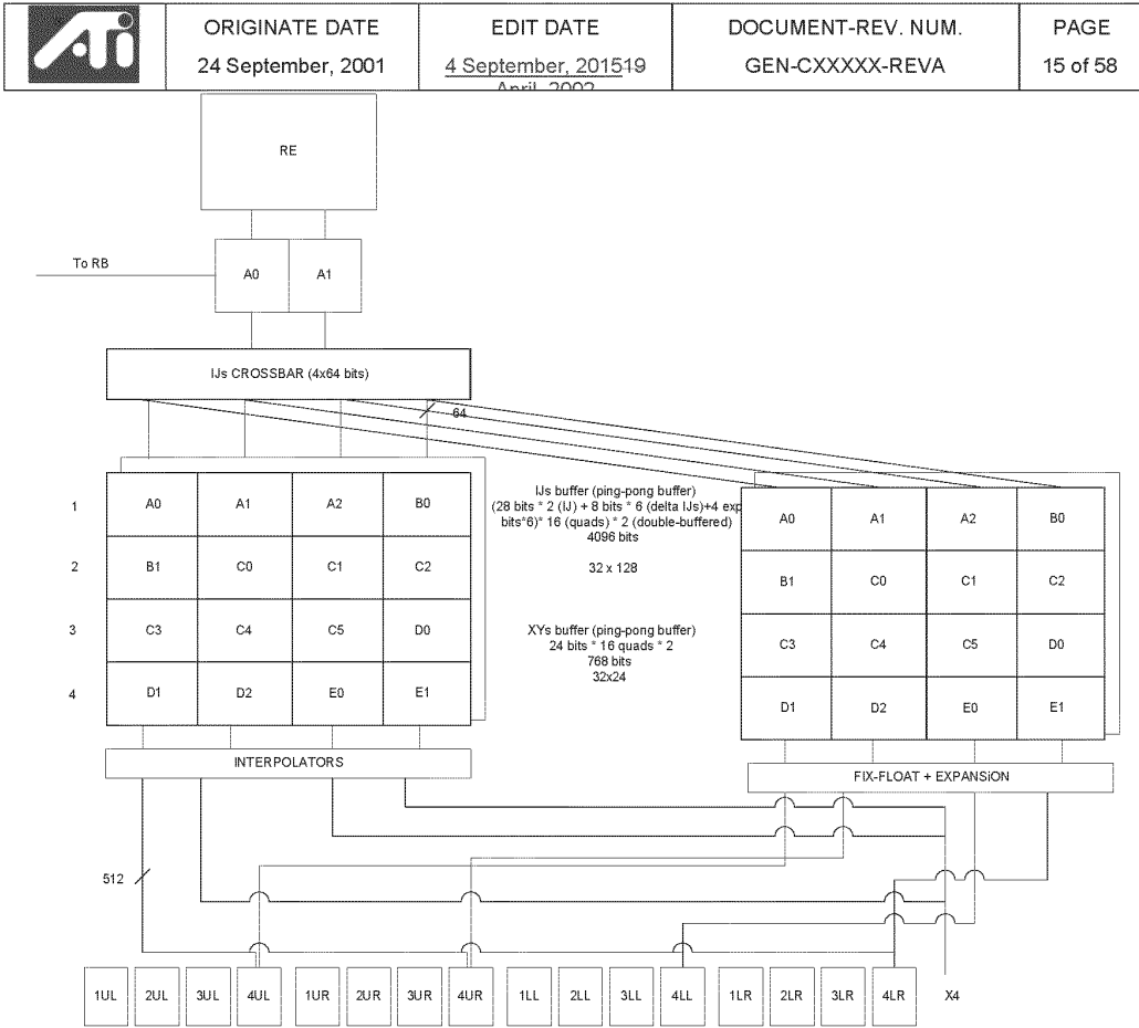
Figure 5: Interpolation buffers
