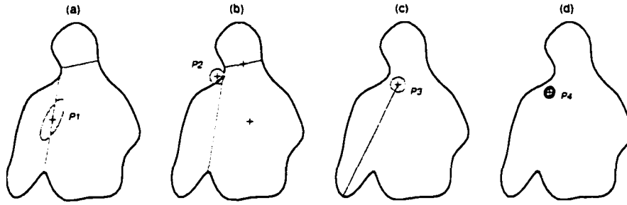
Figure 4.1: Updating the location of the joint between the arm and the torso: (a) the initial estimate based on body part identification, (b) the estimate based on the locations of the torso and head, (c) the estimate based on the major axis of the arm, and (d) the weighted least squares estimate integrating estimates P_1 , P_2 , and P_3 .
