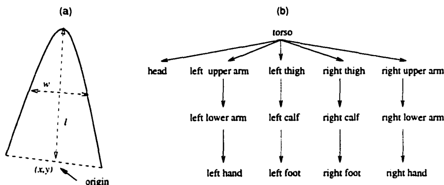
Figure 2.6: (a) Body part model (b) "connect-to" hierarchy
