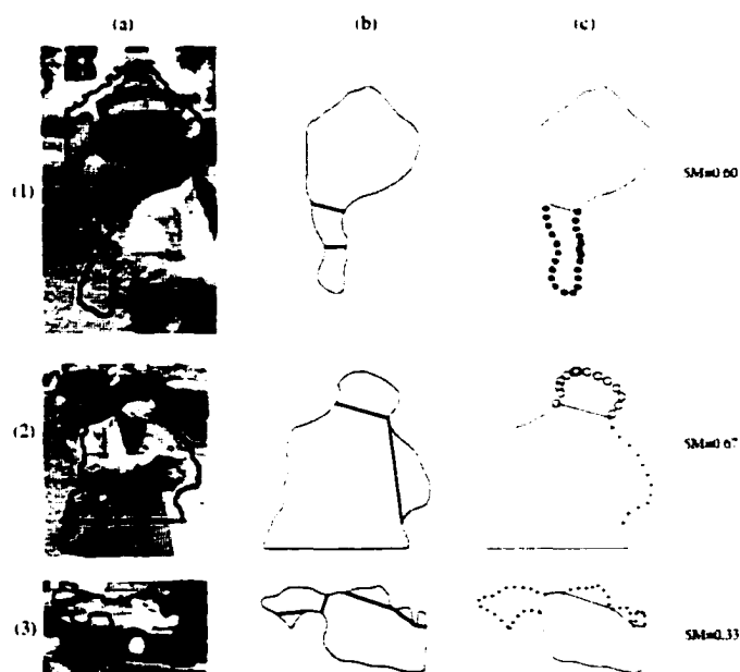
Figure 4.6: The first iteration of the RCR algorithm
