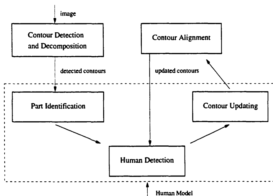
Figure 1.9: Flow chart of the RCR algorithm
