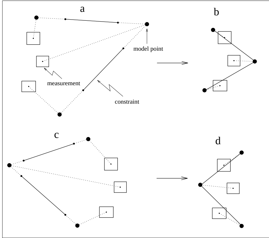
Figure 7: Two examples of a priori estimates (a and c) and their corresponding solutions (b and d). Model points are represented by black circles, measurements and their uncertainty by rectangles and distance constraints by bold lines. The dotted lines connect between a measurement and its associated model point.
