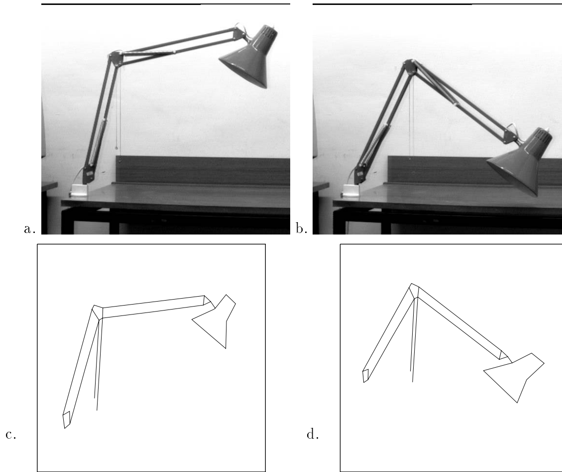
Figure 12: a-b) Images of a desk lamp at different positions. c-d) The corresponding result shown as a synthetic image created from the estimated location vector.
