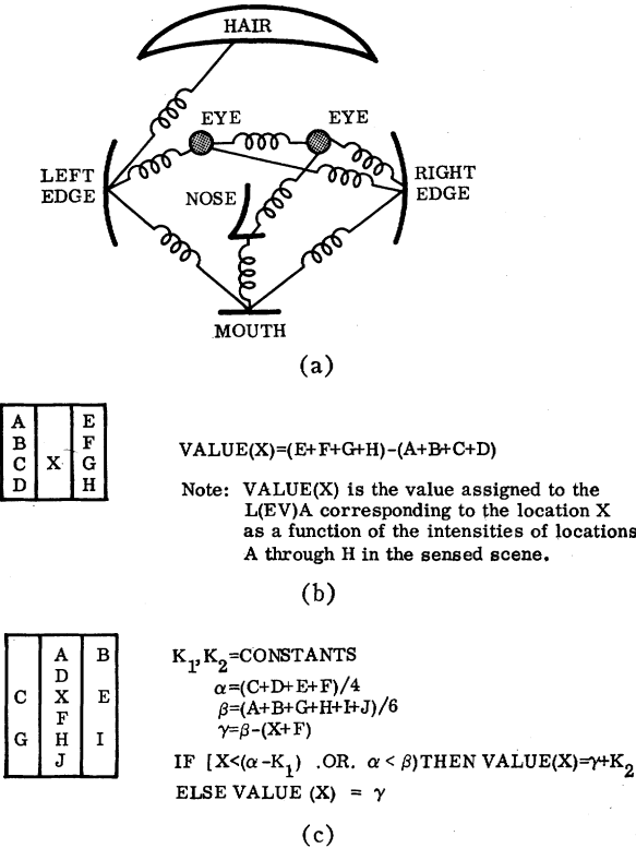
Fig. 3. Reference description of a face. (a) Schematic representation of face reference, indicating components and their linkages. (b) Reference description for left edge of face. (c) Reference description for eye.
