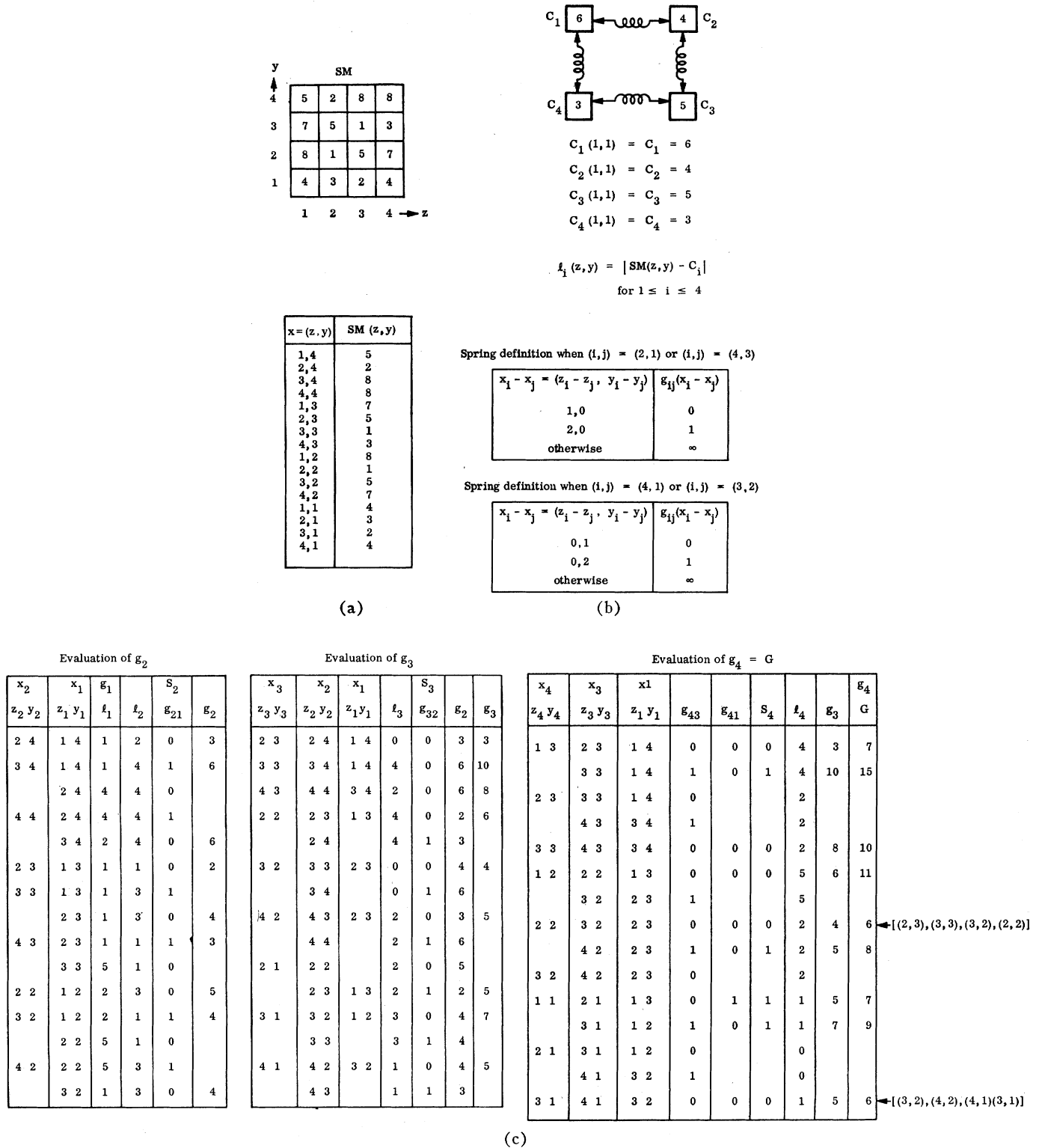
Fig. 1. An example illustrating the operation of the linear embedding algorithm. The definitions of x , g_{ij} , l_i are given on pages 69 and 71. z and y are the components of x ; that is, x = (z, y) . (a) The sensed image. (b) The reference description. (c) Linear embedding algorithm.
