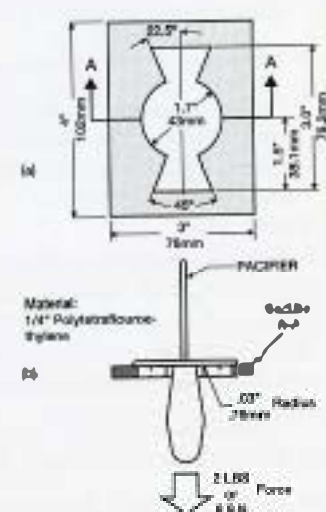
PACIFIER TEST FIXTURE
