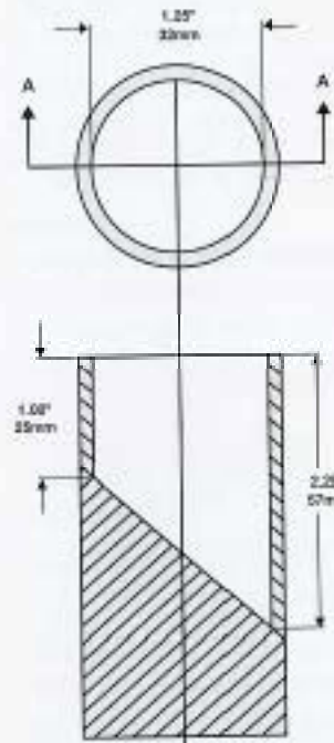
SMALL PARTS GAUGE Section A-A
