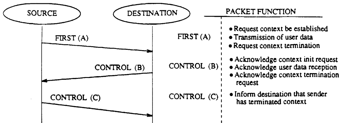
Figure 2. Three Packet Connection-Mode Handshake
