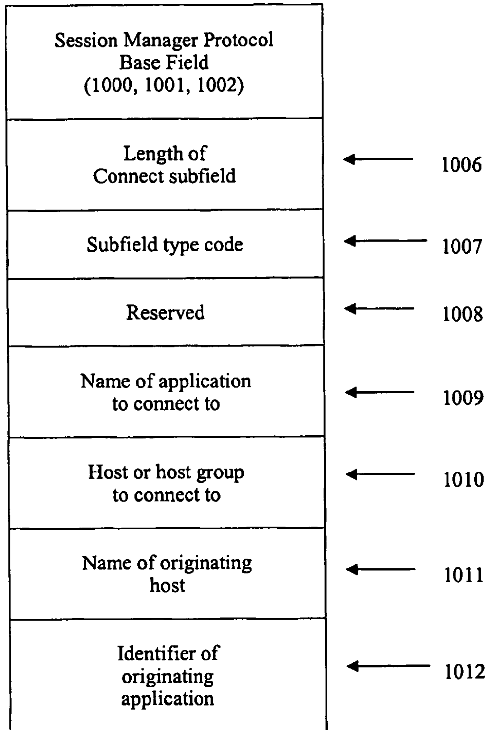
Data Mover Session Manager Protocol Connect Subfield
