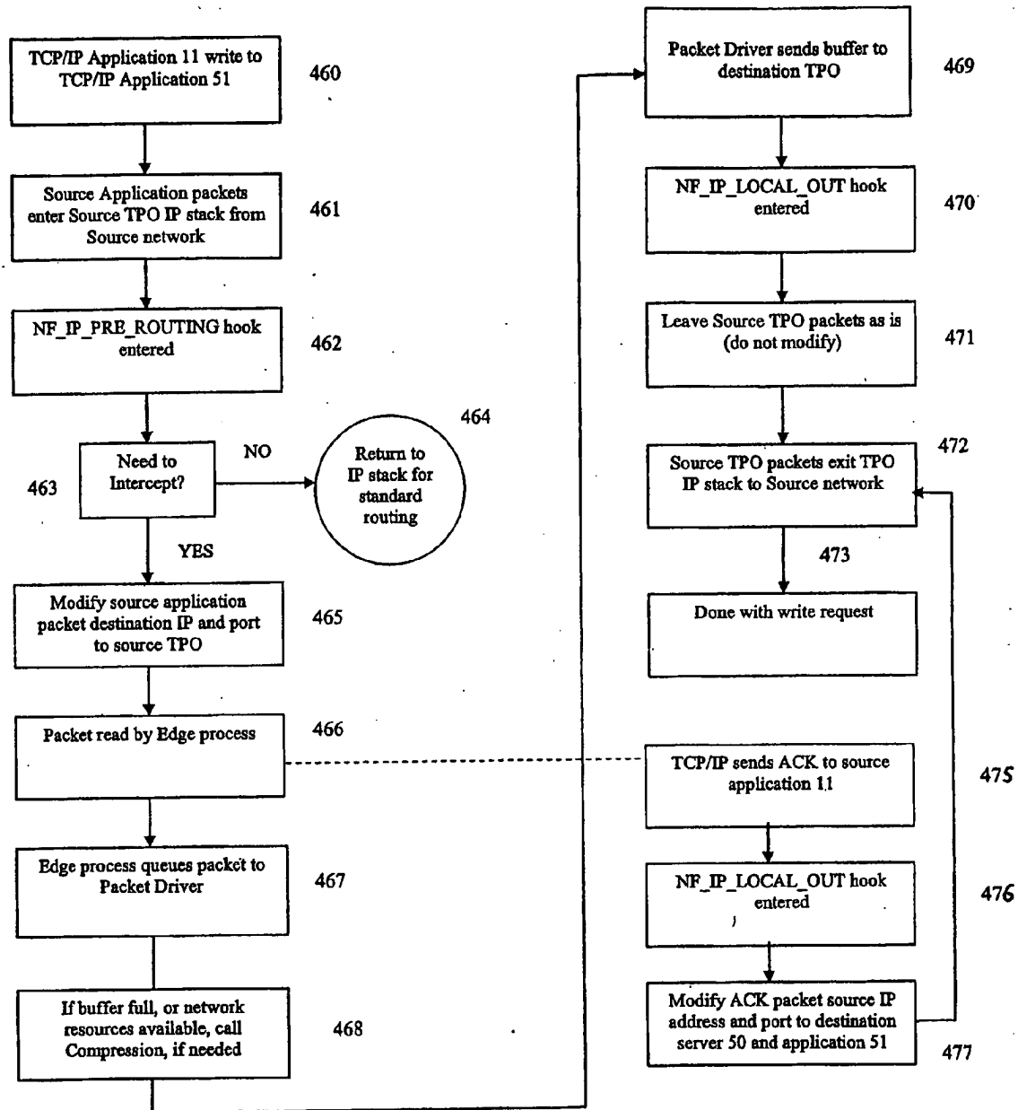
TCP/IP Application Write Process
