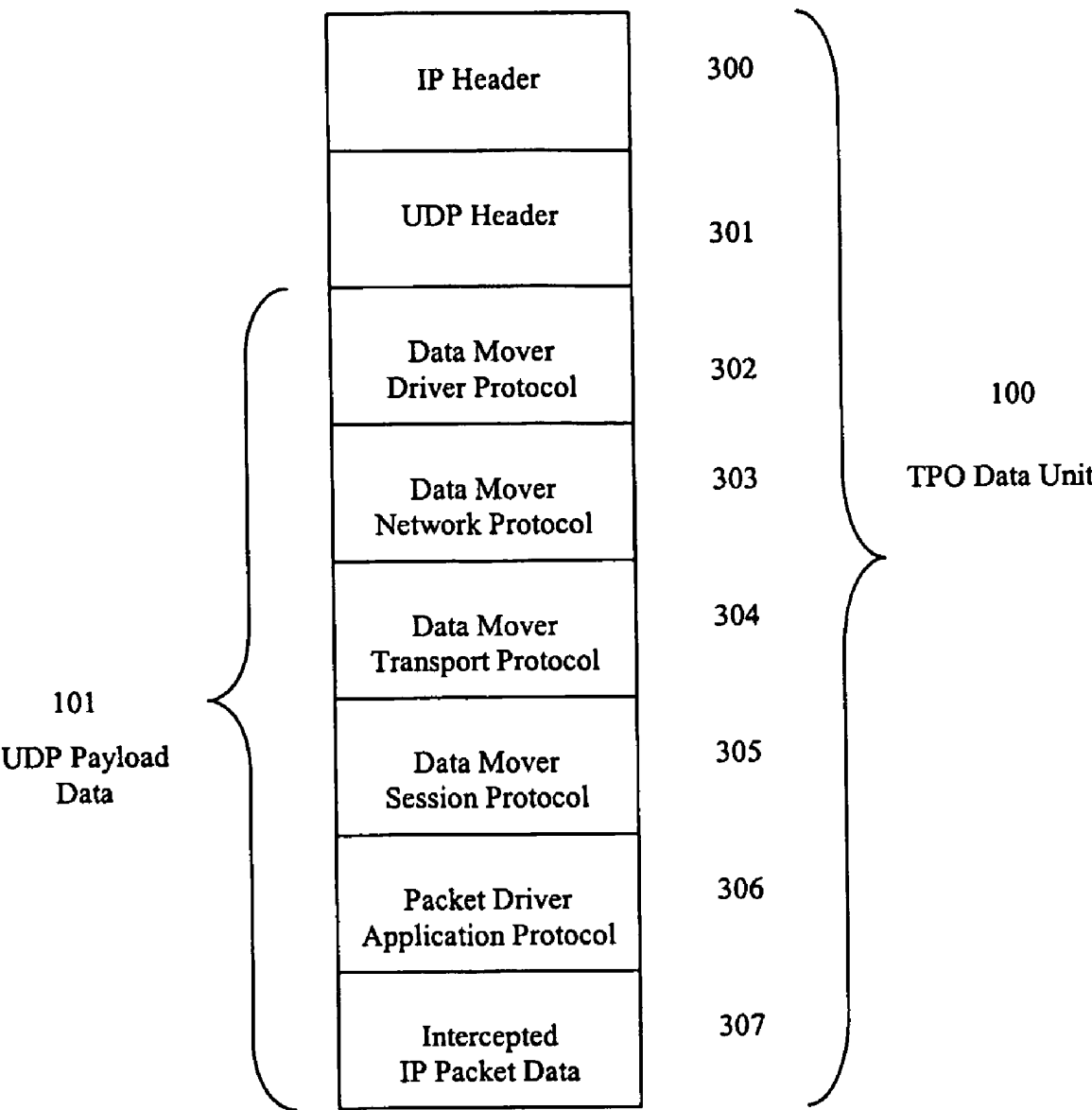
Transport Protocol Optimizer Data Unit
