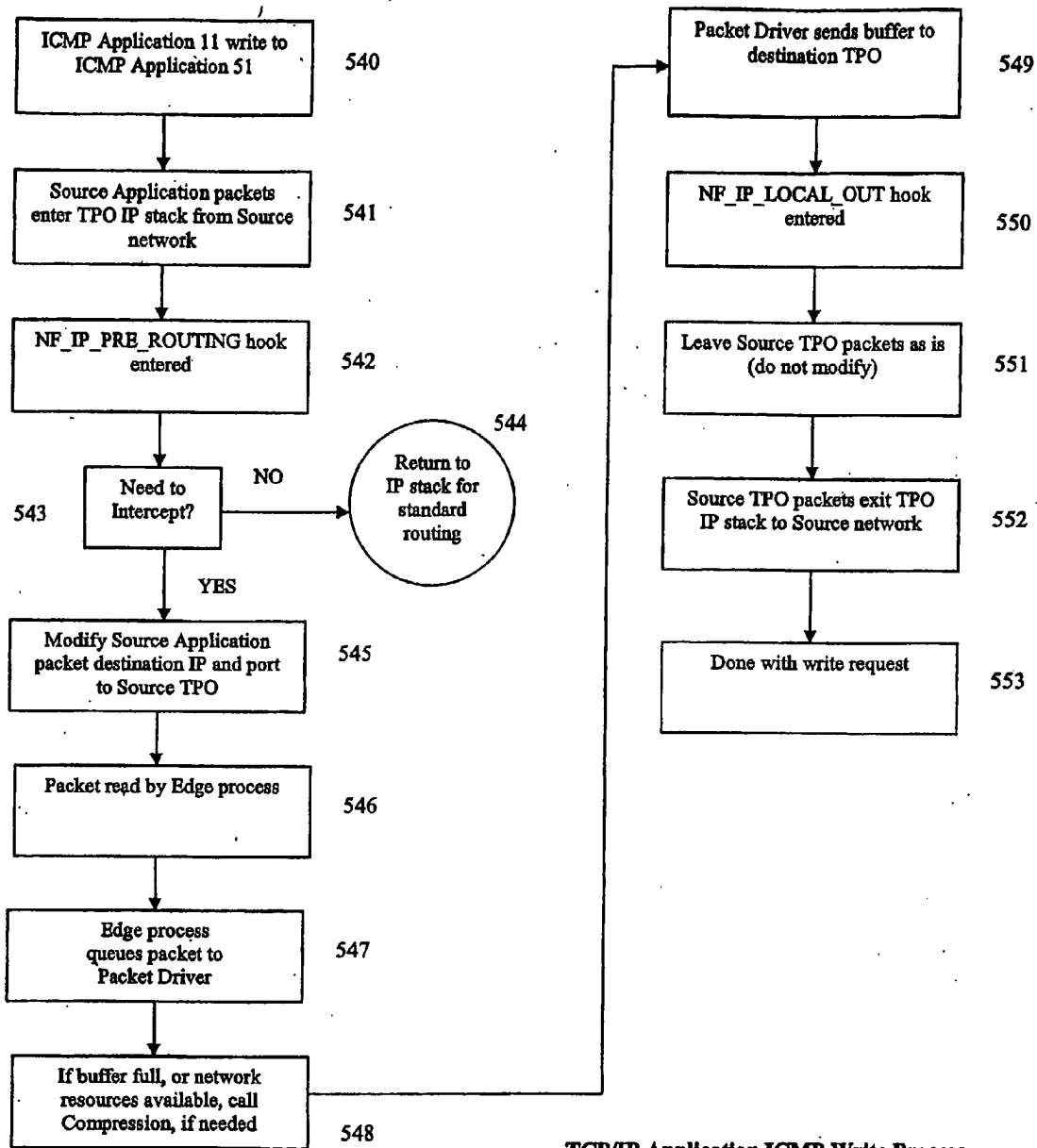
TCP/IP Application ICMP Write Process (Source Side)
