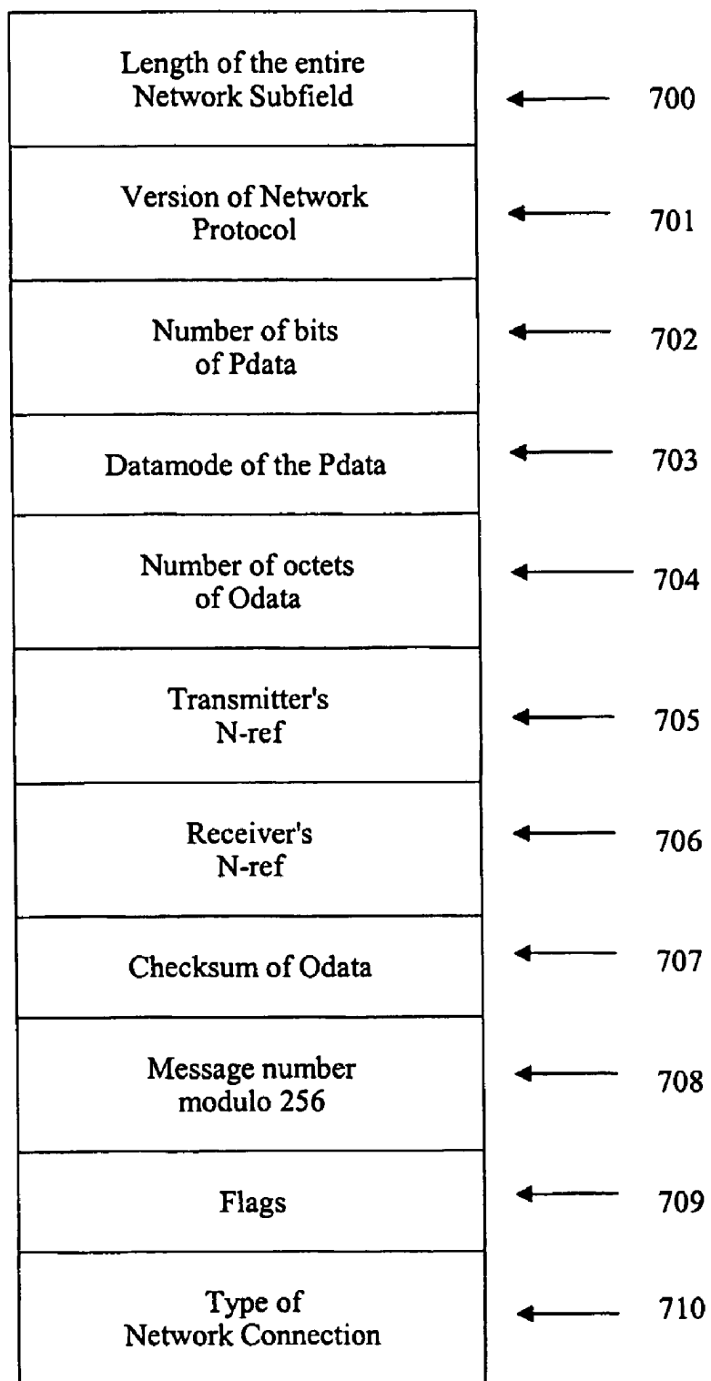
Data Mover Network Message Header
