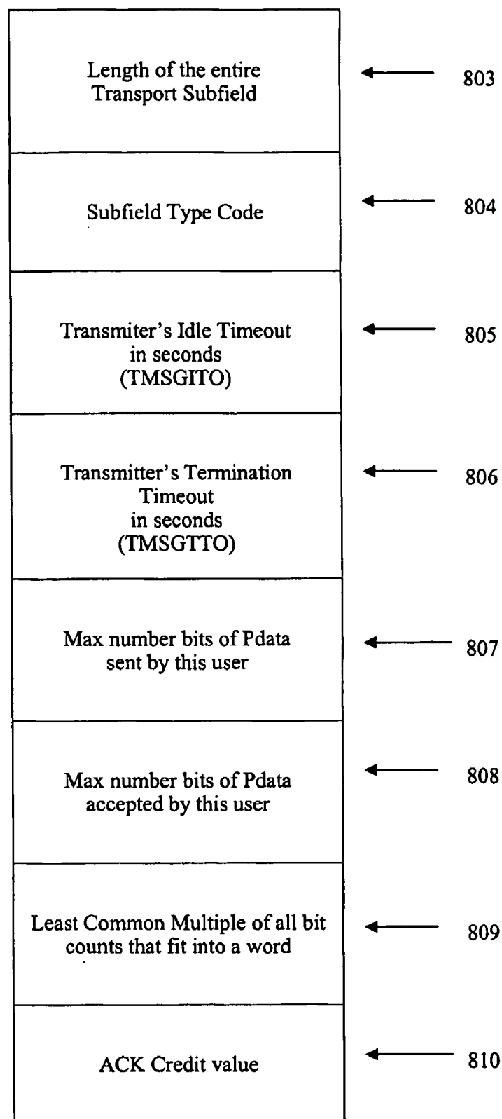
Data Mover Transport Protocol Connect Subfield
