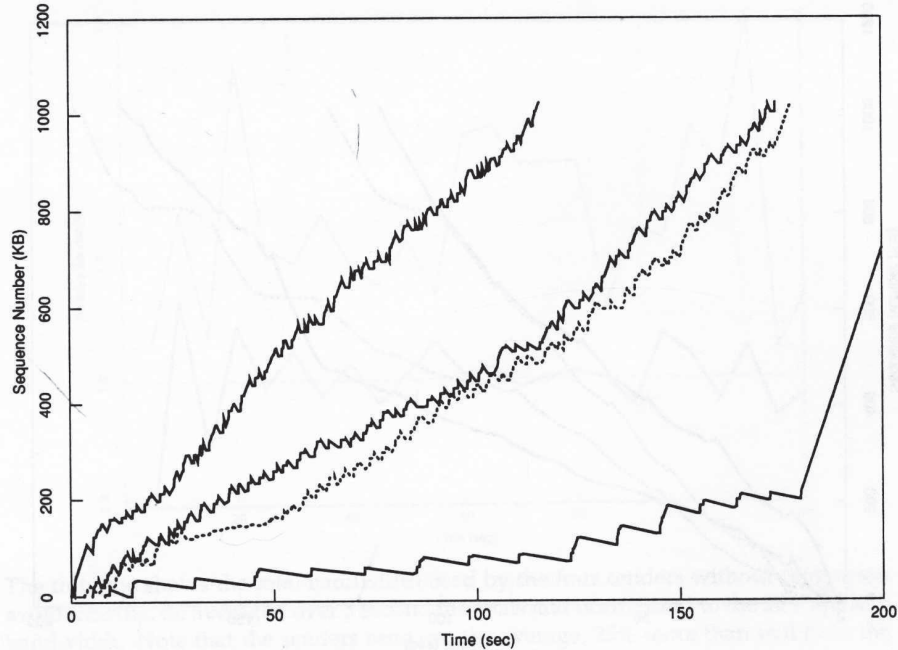
Trace data from four simultaneous TCP conversations without congestion avoidance over the paths shown in figure 7.
