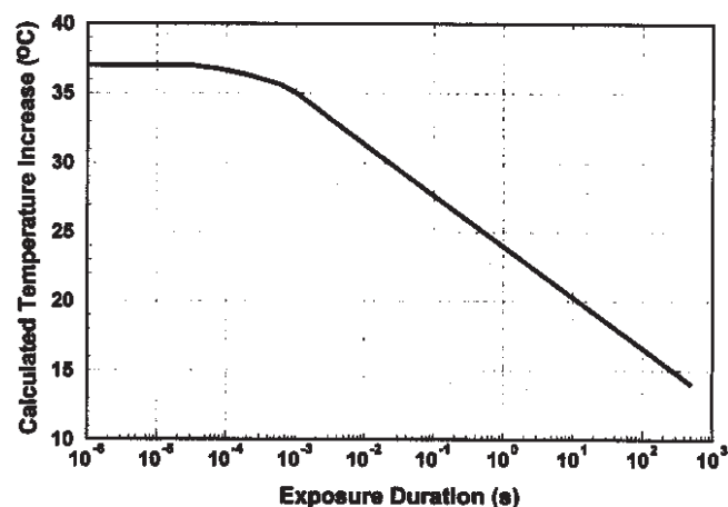
Fig. 2. The calculated peak temperature rise (at the image radius) necessary to result in retinal thermal injury in a 50 \mu m retinal image as a function of duration of light exposure (Priebe and Welch 1978; Allen and Polhamus 1989). Because of longer cooling times for larger images, smaller peak temperatures would be required for significantly larger retinal images, but the general trend will be similar.
