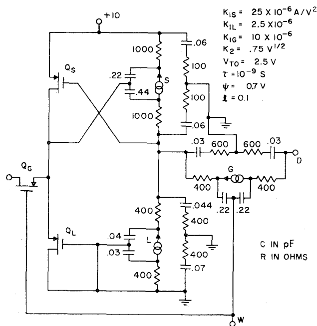
Fig. 10. IGFET memory cell circuit.
