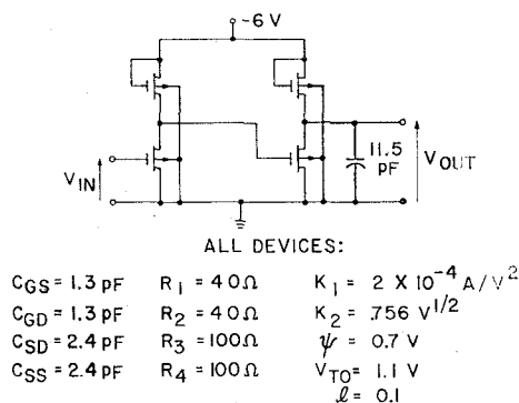
Fig. 7. Cascade of two IGFET inverter stages.
