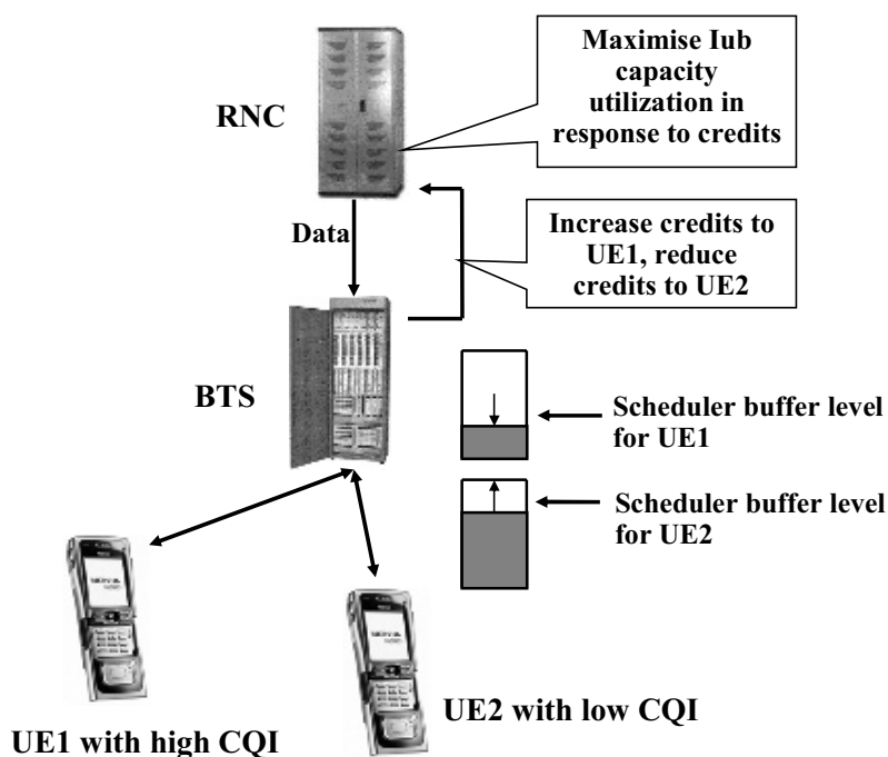
Figure 3.8 HSDPA flow control on the Iub interface.
