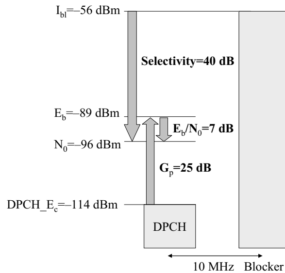
Figure 11.6 In-band blocking with a 10-MHz offset.
