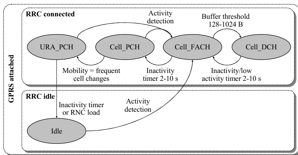
Figure 9.6 RRC states for packet-switched services.
