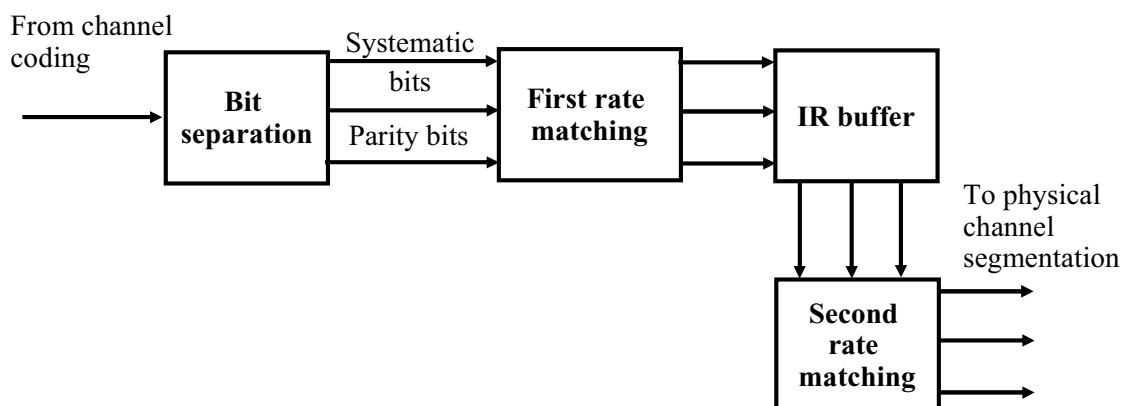
Figure 4.6 HARQ functionality.
