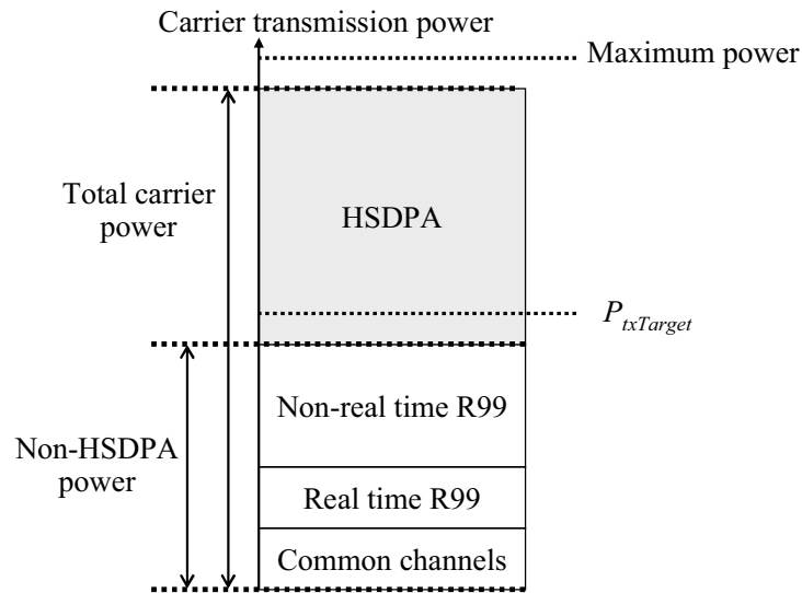
Figure 6.3 Illustration of downlink power budget.
