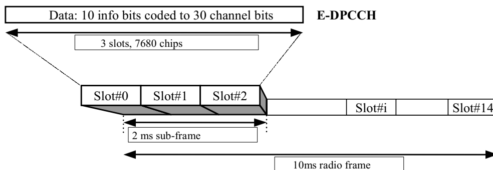
Figure 5.7 E-DPCCH frame structure.
