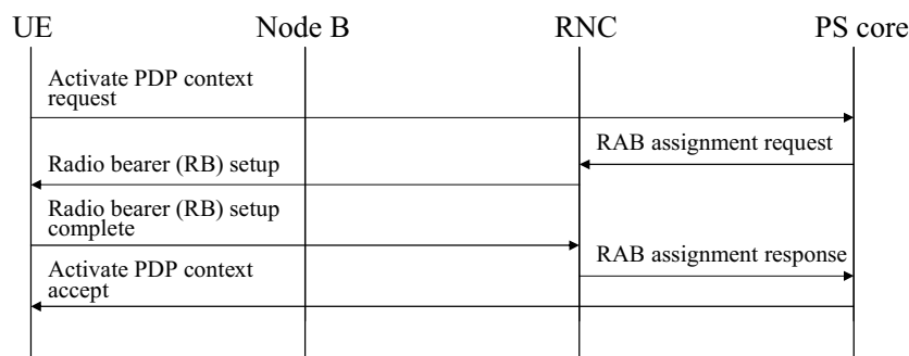
Figure 9.11 GPRS session management.
