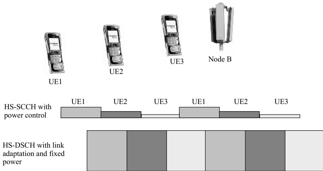
Figure 6.15 Principle behind HS-SCCH power control.
