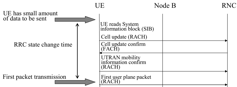
Figure 9.14 RRC state change from PCH to FACH.
