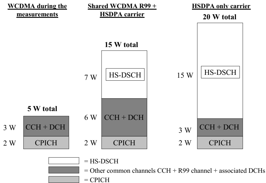
Figure 7.19 Assumed power allocations for HSDPA deployment.
