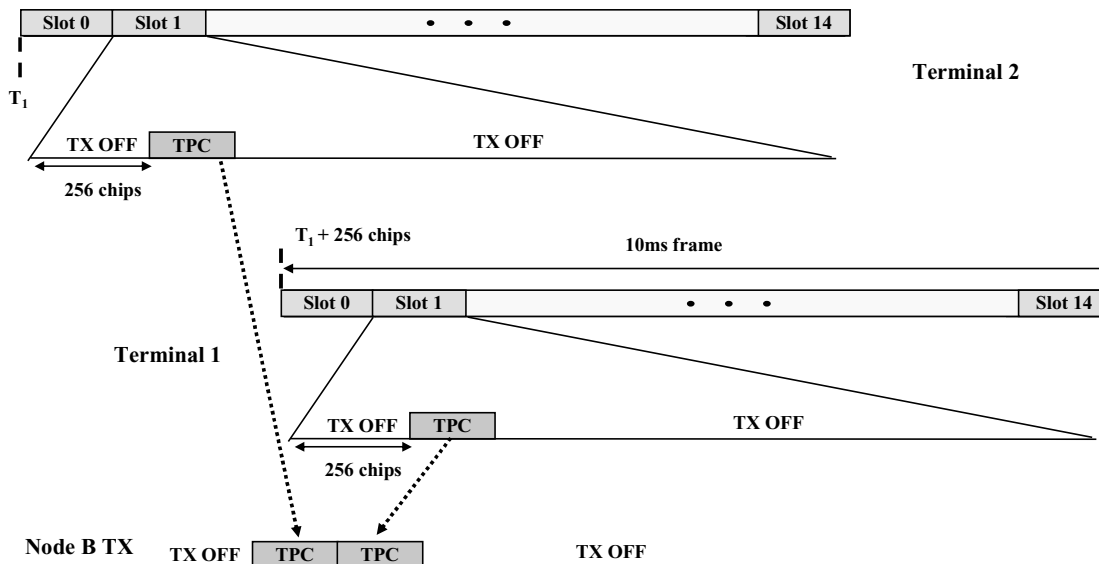
Figure 4.17 Fractional DPCH principle for Node B transmission.
