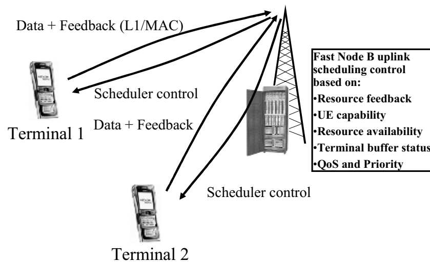
Figure 5.1 HSUPA Node B (BTS) scheduling principle.
