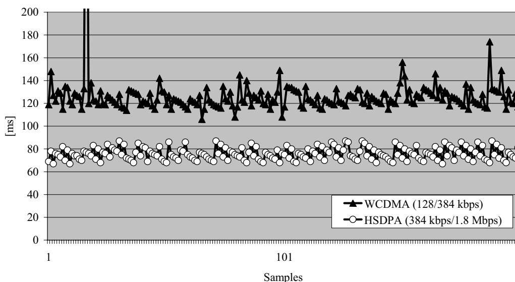
Figure 7.31 Example measured WCDMA and HSDPA RTTs.
