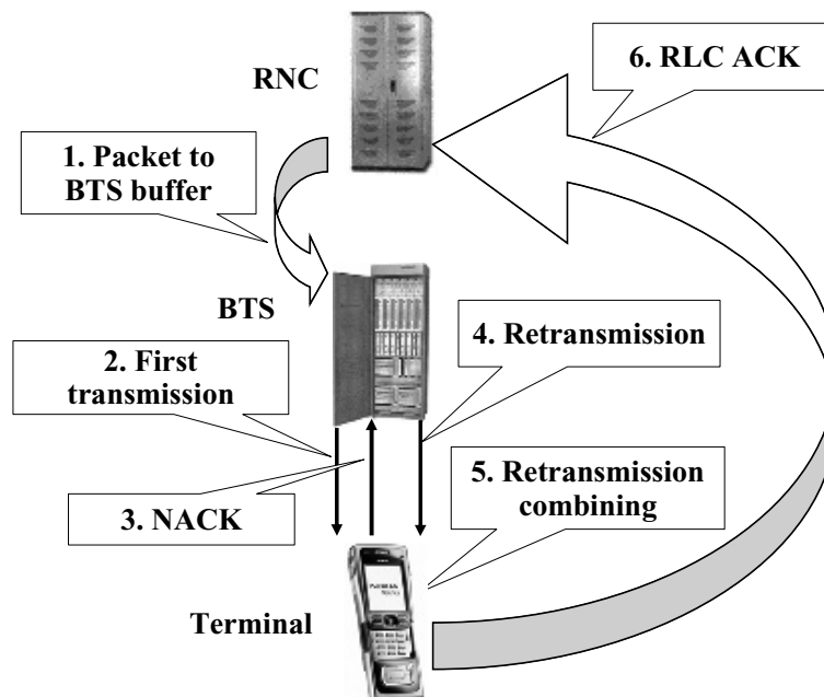
Figure 4.3 BTS retransmission handling.
