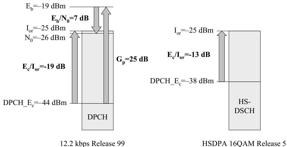
Figure 11.10 Terminal maximum input signal level test with DCH and with HSDPA 16QAM.
