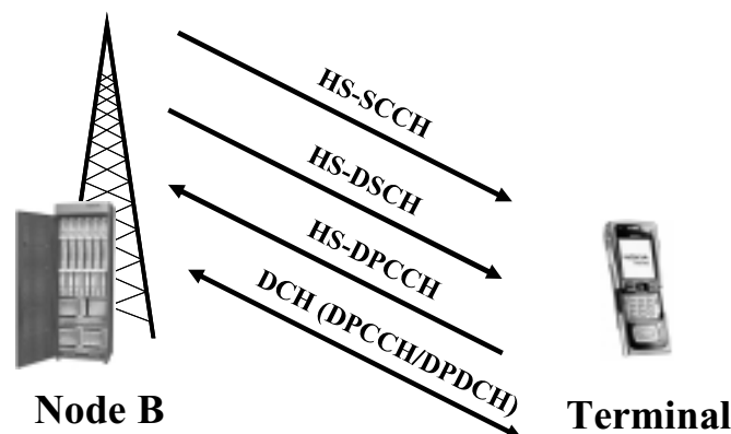
Figure 4.1 Channels needed for HSDPA operation in Release 5.
