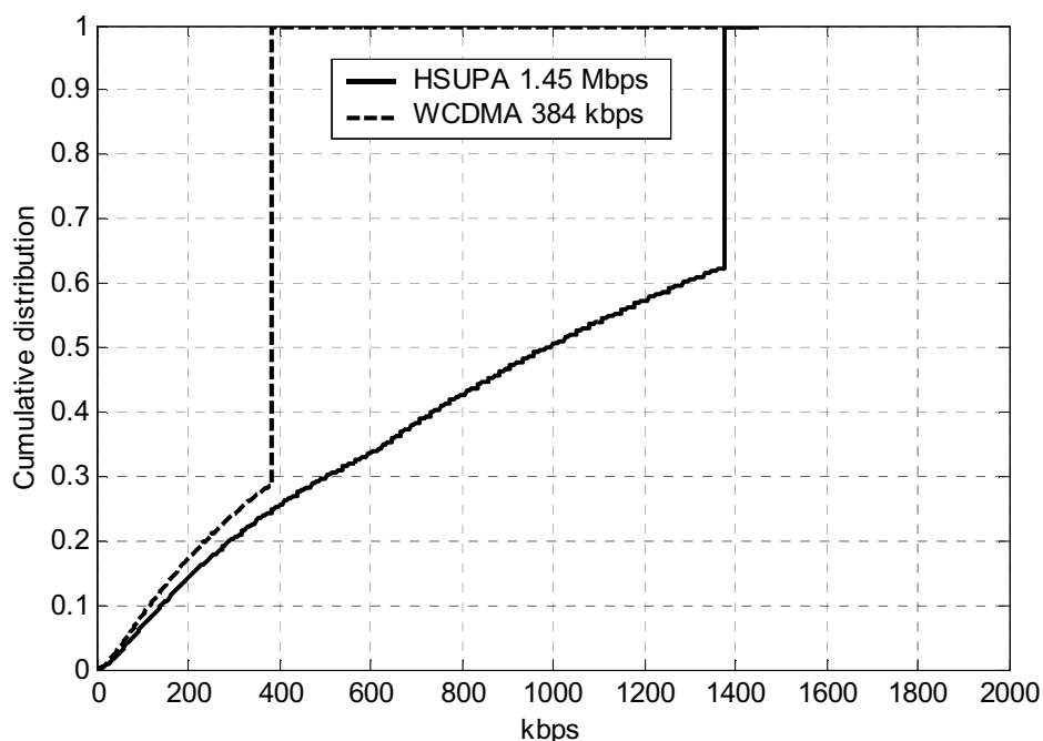
Figure 8.5 User bit rate distribution.
