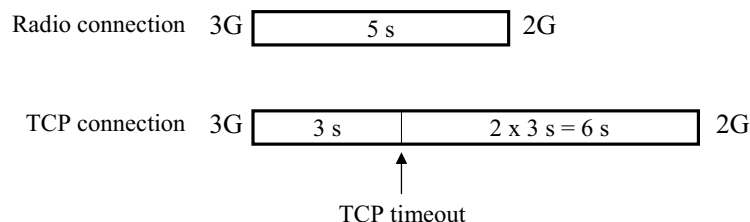
Figure 9.18 TCP timeout during inter-system cell change.
