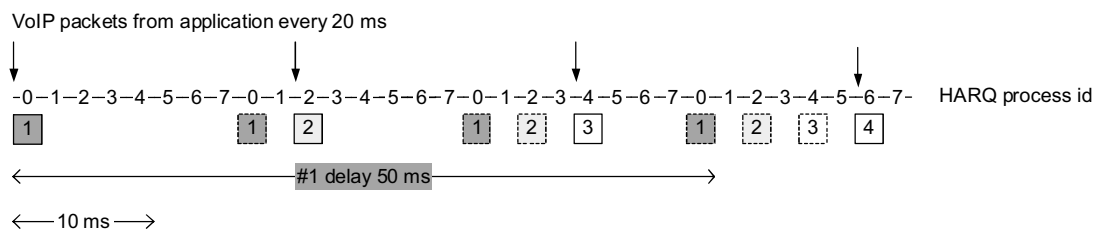
Figure 10.7 VoIP on the E-DCH with a 2-ms TTI – here, one VoIP packet is transmitted every 20 ms.
