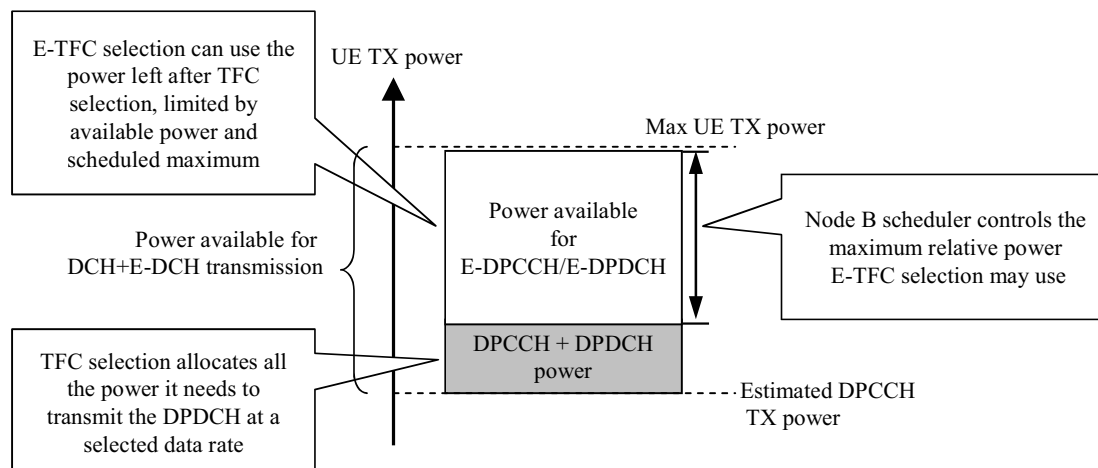
Figure 5.20 E-DCH and DCH power resource sharing.
