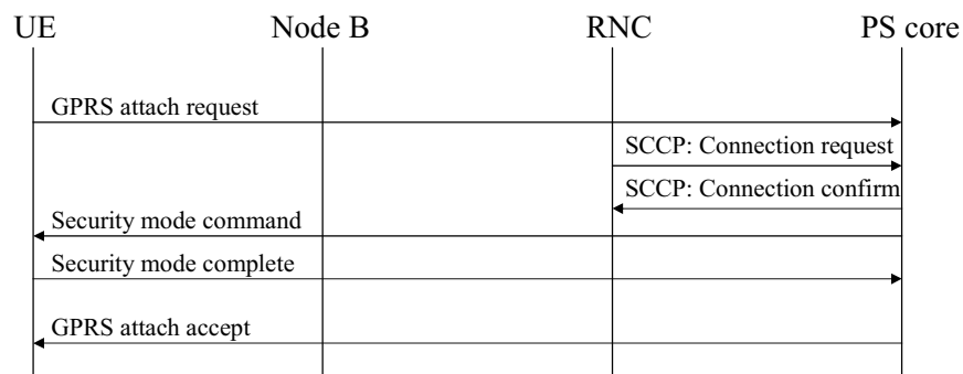
Figure 9.10 GPRS mobility management.
