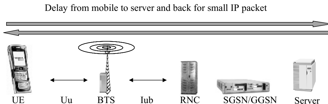
Figure 7.29 Definition of round trip time (RTT).
