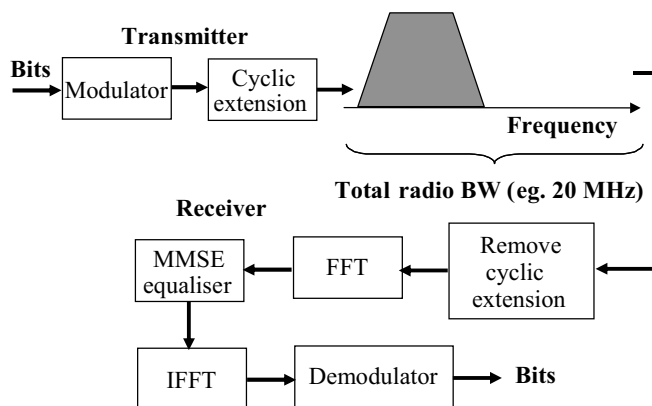
Figure 2.7 SC-FDMA principle.
