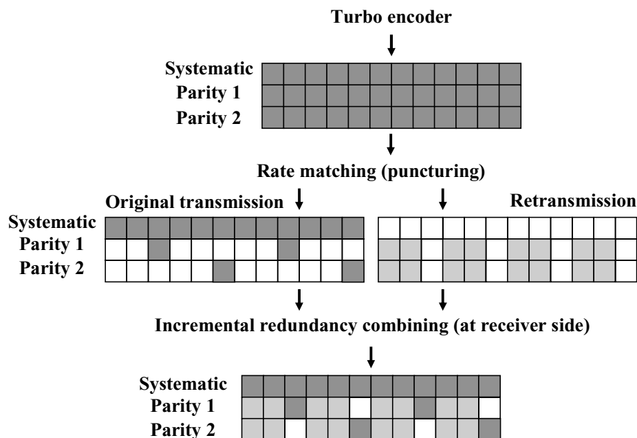
Figure 4.8 HARQ principle with non-identical retransmissions.
