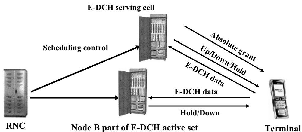
Figure 5.23 HSUPA scheduling in soft handover.
