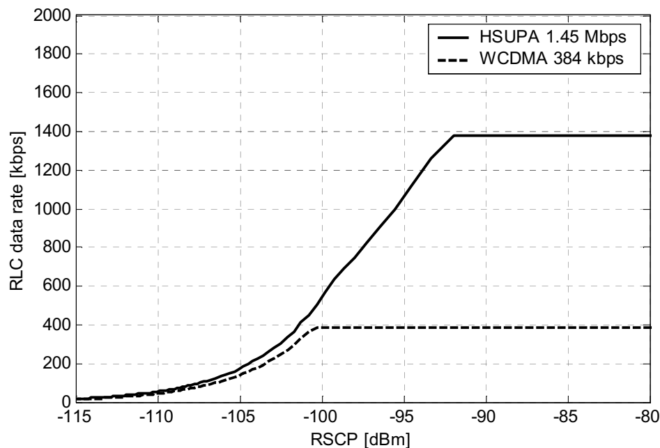
Figure 8.4 Instantaneous single-user uplink throughput vs CPICH RSCP.
