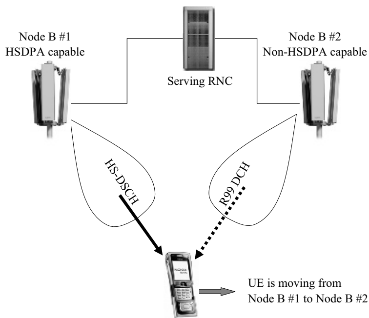
Figure 6.11 Example of HS-DSCH to DCH handover.
