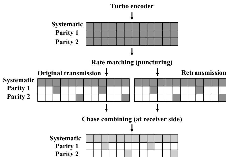
Figure 4.7 Chase (soft) combining principle with identical retransmissions.
