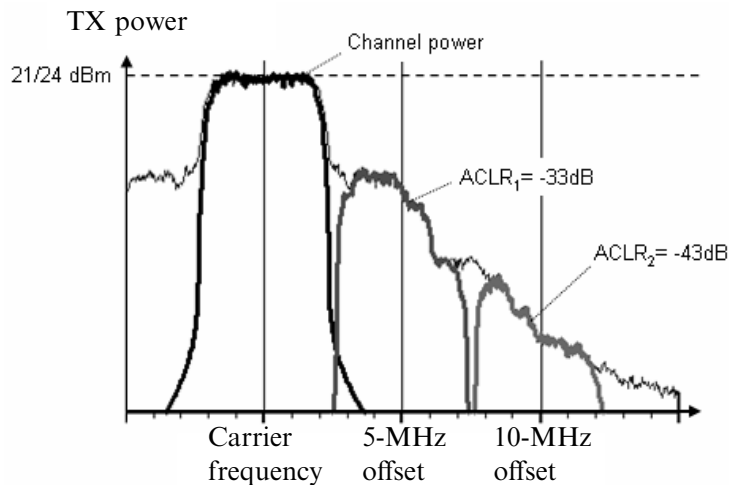
Figure 11.1 Adjacent channel leakage ratio with terminal transmission.
