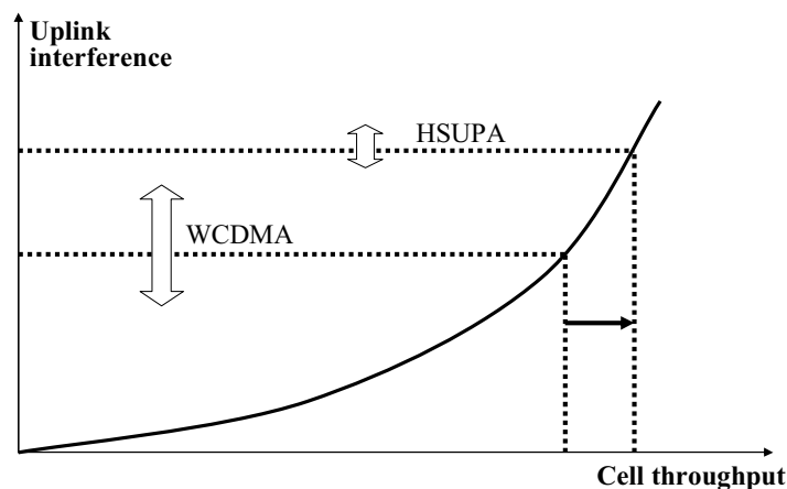
Figure 6.22 Uplink load curve and the impact of fast scheduling.
