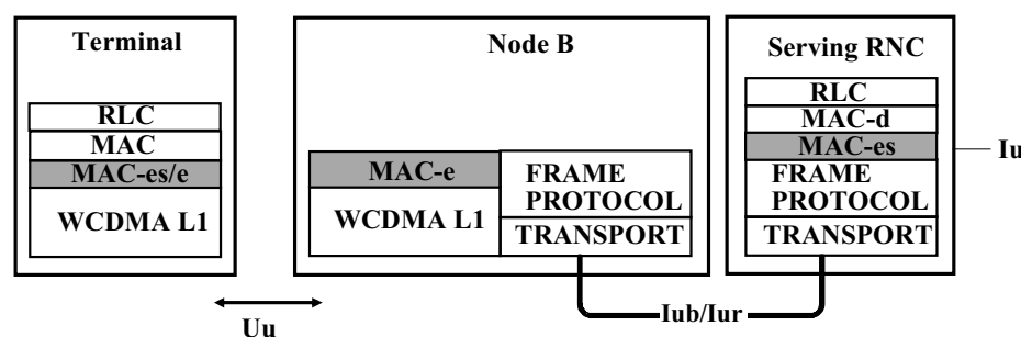
Figure 3.6 HSUPA user plane protocol architecture.
