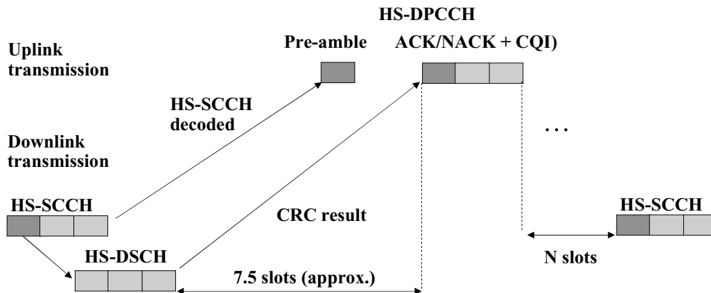
Figure 4.21 Operation with pre/post scheme of Release 6.
