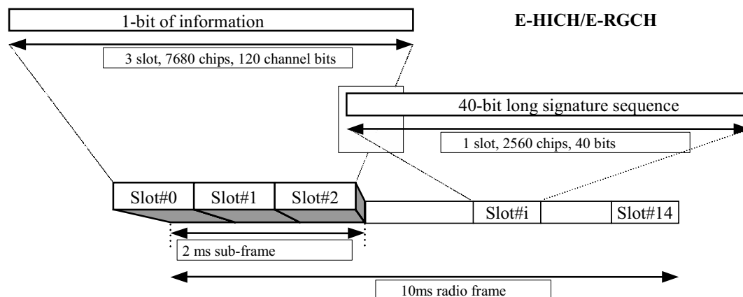
Figure 5.8 E-HICH/E-RGCH frame structure.
