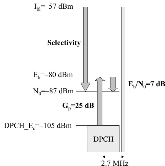
Figure 11.7 Narrowband blocking against a GSMK-modulated interferer.
