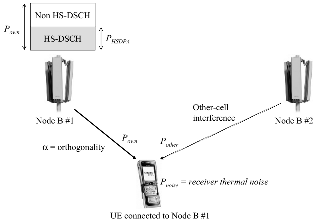
Figure 7.1 HSDPA performance factors.
