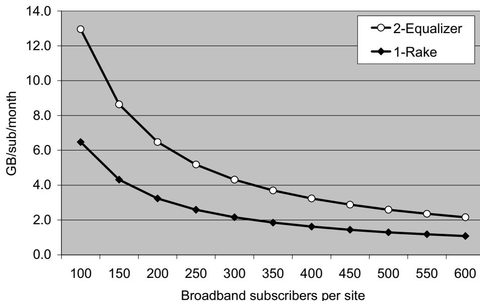
Figure 7.27 Data capacity per subscriber per month.
