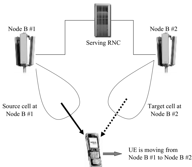
Figure 6.8 Inter Node B HS-DSCH to HS-DSCH handover.
