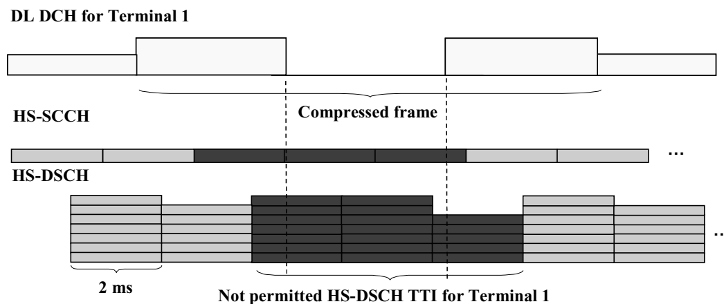
Figure 4.24 HSDPA operation with compressed mode.
