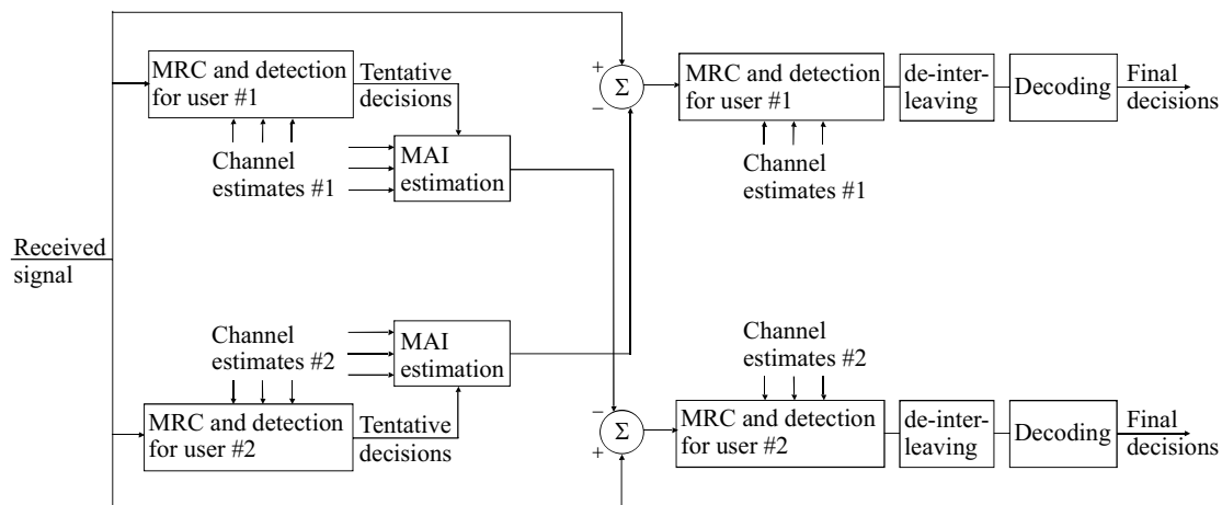
Figure 8.15 Parallel interference cancellation receiver for two users [16].
