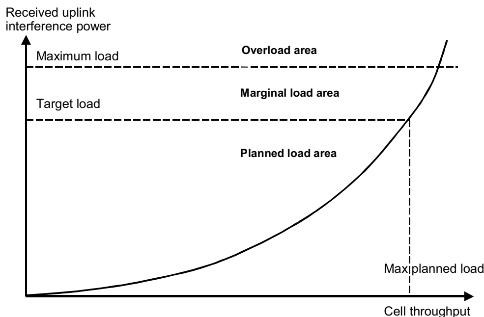
Figure 5.3 Uplink load curve.
