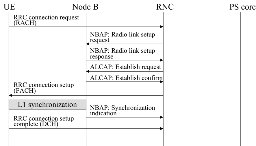
Figure 9.9 Radio resource control (RRC) connection setup.
