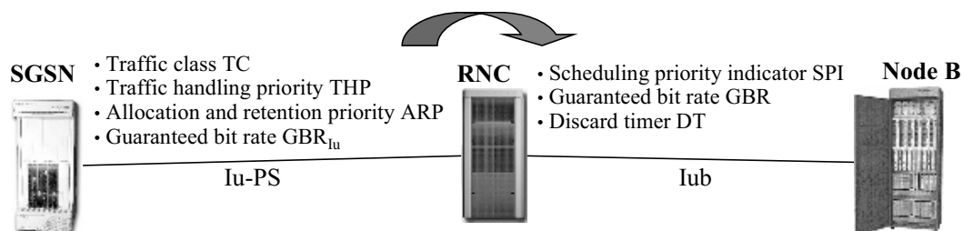
Figure 6.5 3GPP QoS parameters in the Iu-PS and Iub interfaces.
