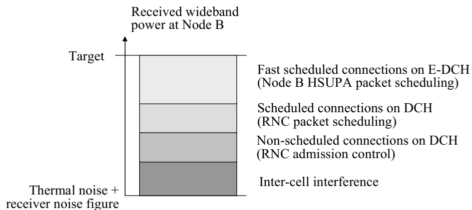
Figure 6.21 Resource allocation control with HSUPA.
