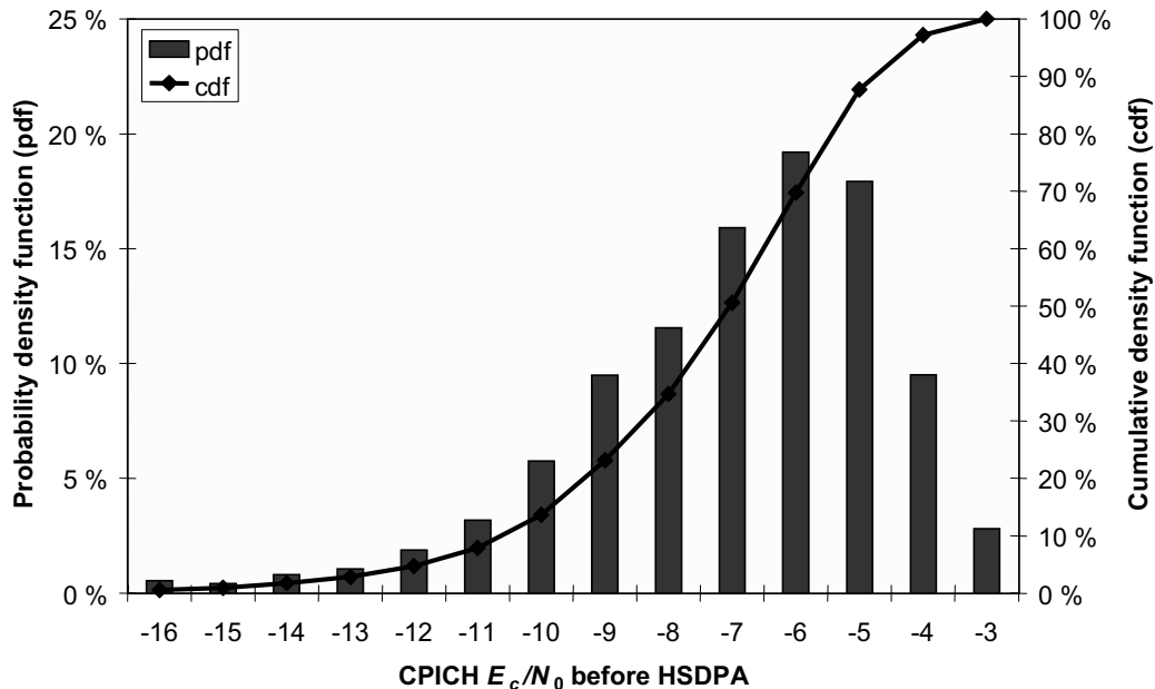
Figure 7.20 Drive test data before HSDPA.
