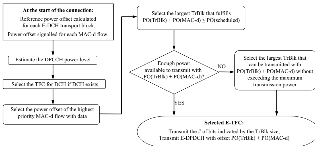
Figure 5.19 HSUPA E-TFC selection.
