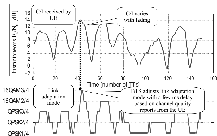
Figure 4.18 Link adaptation.
