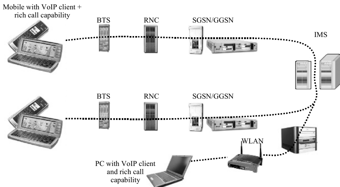
Figure 10.1 VoIP with rich call capabilities.
