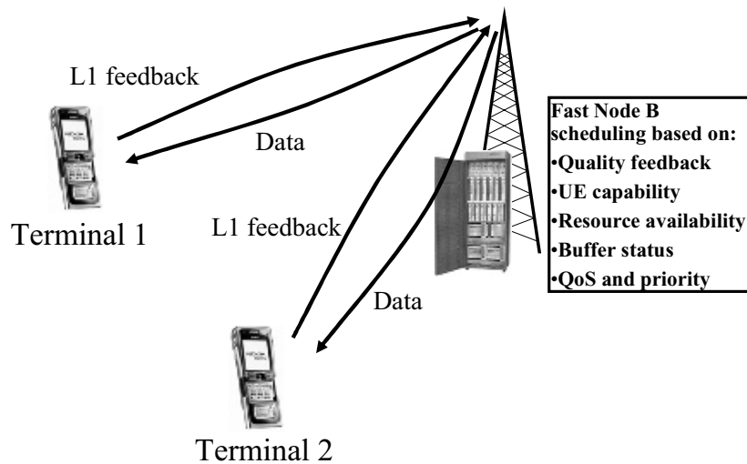
Figure 4.2 HSDPA Node B scheduling principle.
