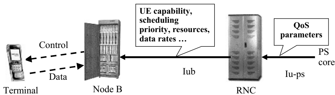
Figure 5.24 HSUPA parameters over the Iub interface.
