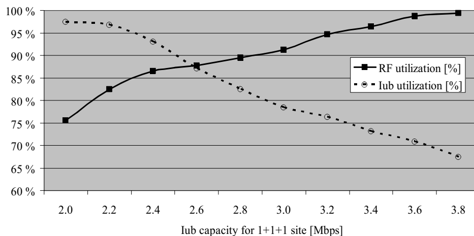
Figure 7.26 Trade-off between HSDPA RF vs Iub efficiency.
