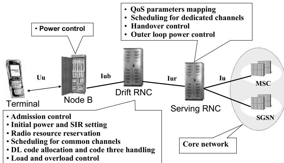
Figure 3.1 Release 99 radio resource management architecture.
