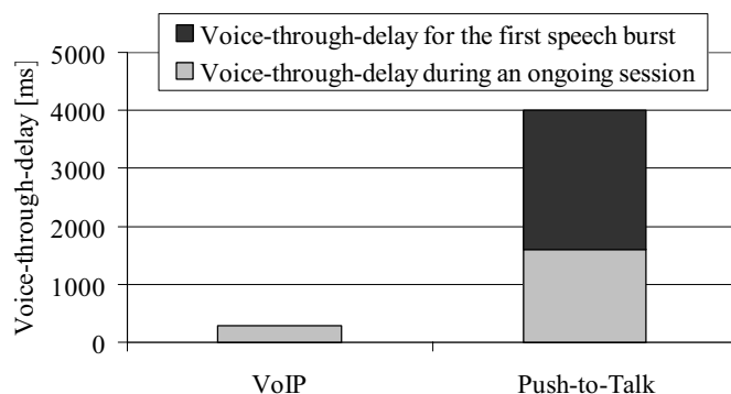
Figure 9.23 Voice-through-delay requirement for VoIP and push-to-talk.
