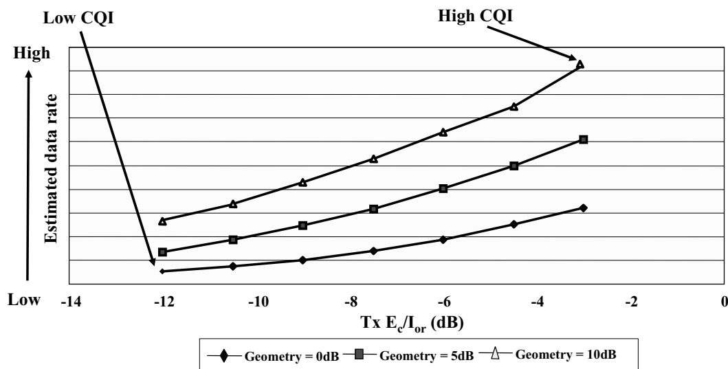
Figure 4.15 Example CQI curves for different geometry values.
