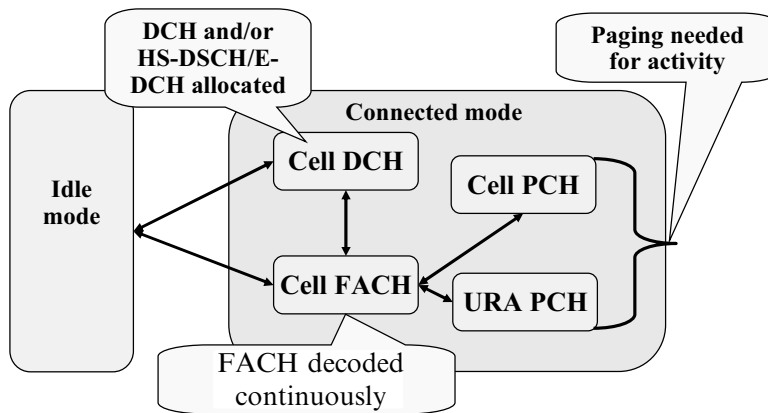
Figure 3.11 RRC states with HSDPA/HSUPA.
