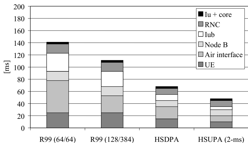
Figure 7.30 Estimated round trip time (RTT) evolution.
