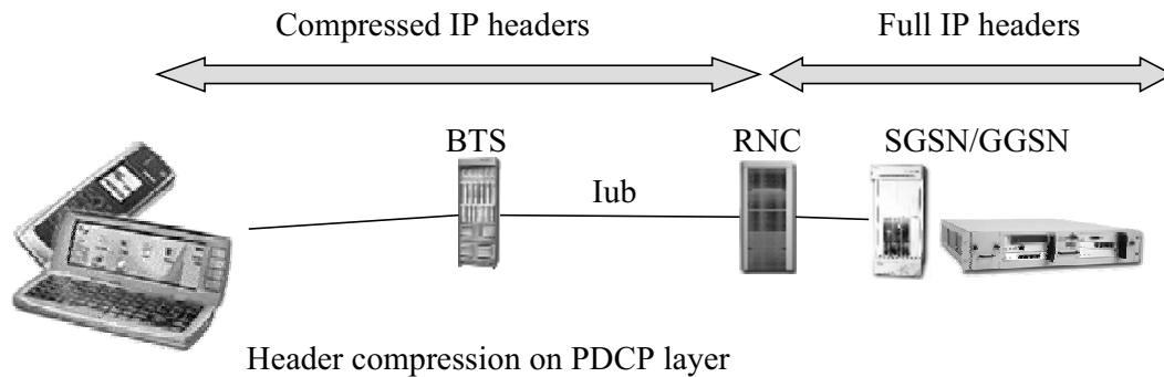
Figure 10.3 IP header compression with VoIP.
