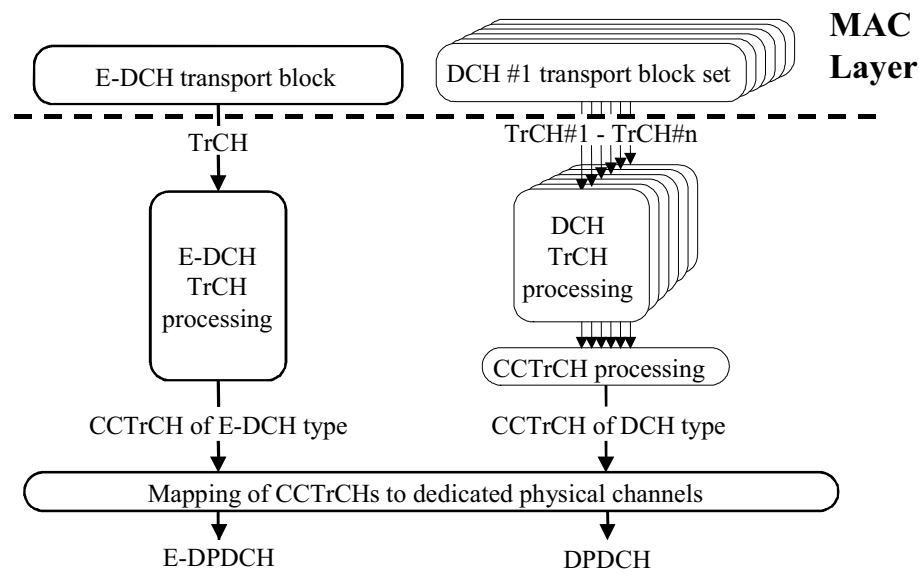
Figure 5.4 Transport channel processing.
