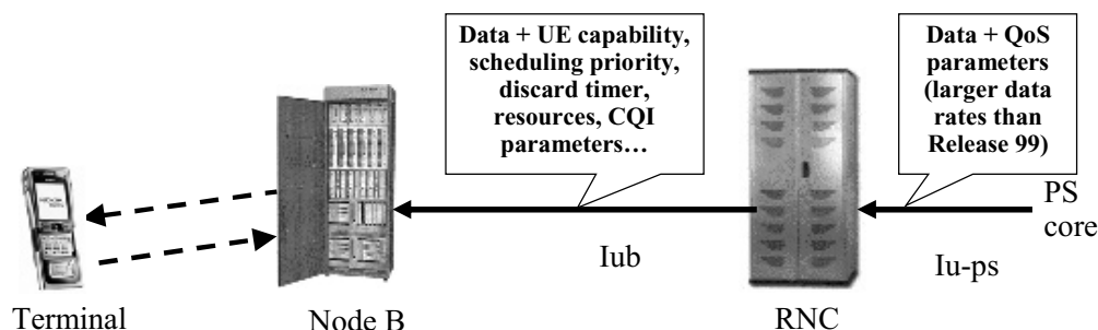
Figure 4.25 HSDPA parameters over the Iub interface.
