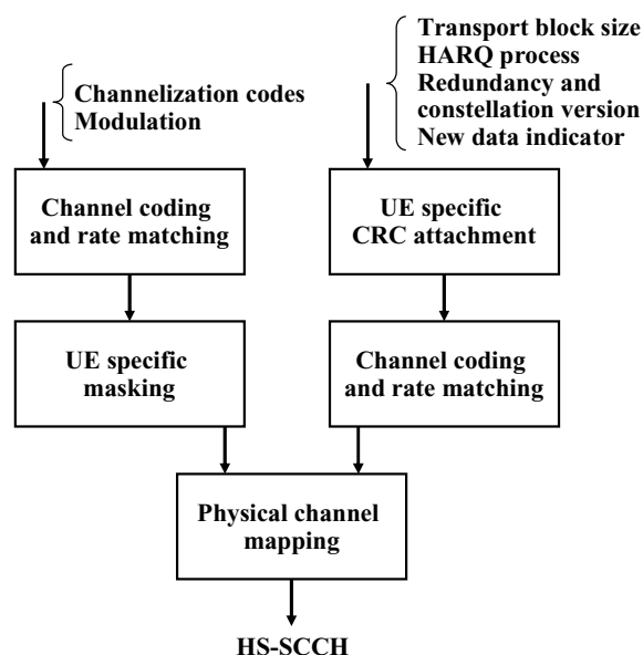
Figure 4.13 HS-SCCH channel coding and multiplexing chain.
