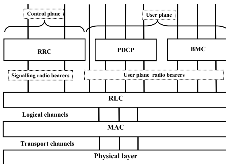
Figure 3.3 Release 99 radio interface protocol architecture.
