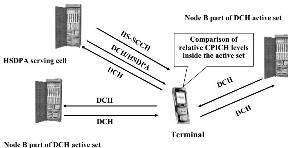
Figure 4.22 HSDPA operation with DCH active set of 3.
