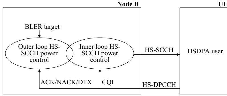
Figure 6.16 Block diagram for HS-SCCH power control algorithm.
