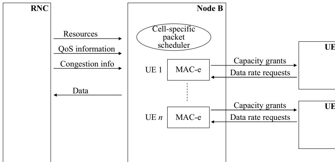
Figure 6.23 Node B based HSUPA packet scheduling environment.
