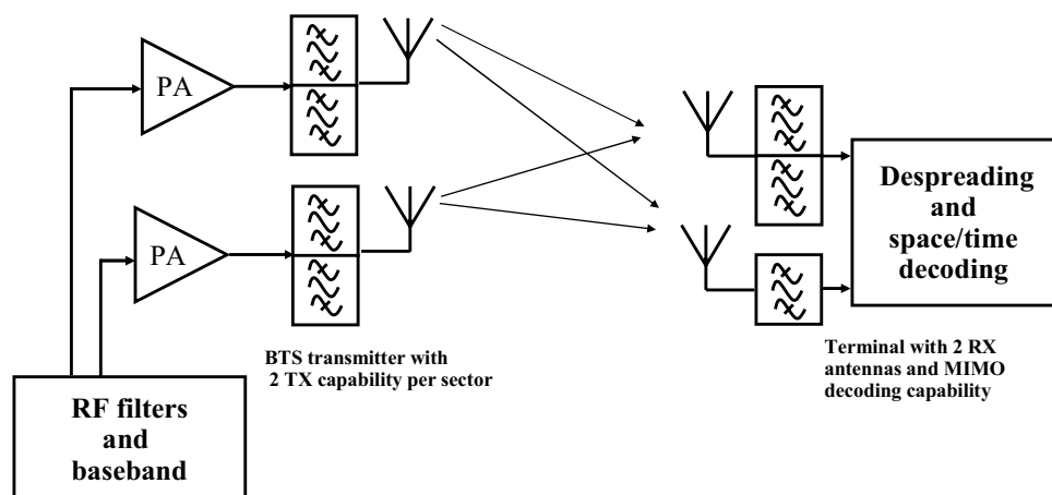
Figure 2.6 MIMO principle with 2 transmit and 2 receive antennas.
