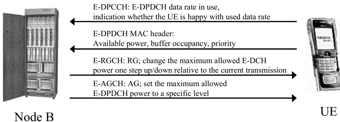
Figure 5.21 HSUPA – scheduling-related information exchanged over the air.
