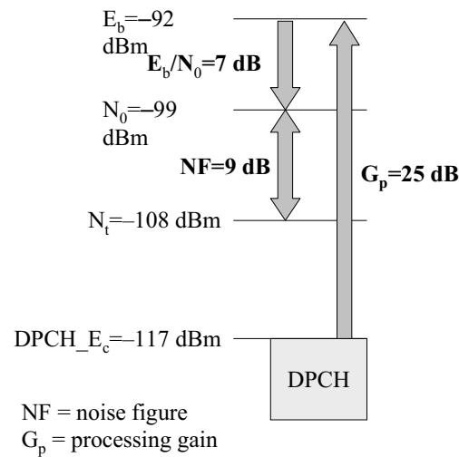
Figure 11.3 Receiver sensitivity test case.
