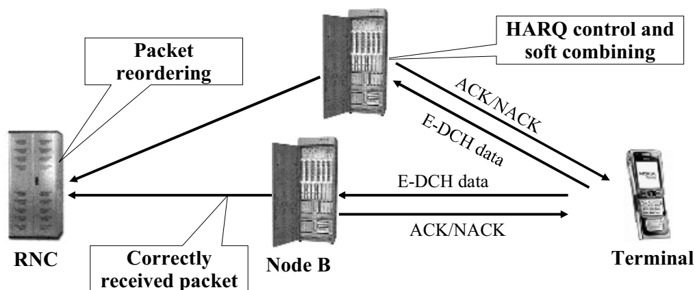
Figure 5.15 HSUPA ARQ operation in soft handover.
