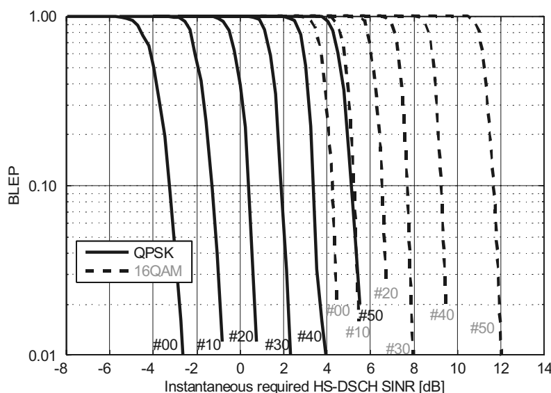
Figure 7.2 Plot of block error probability (BLEP) as a function of the instantaneous HS-DSCH SINR. The BLEP is shown for the parameters given in Table 7.1. This simulation setup is for a 1 × 1 RAKE receiver using an AWGN channel.
