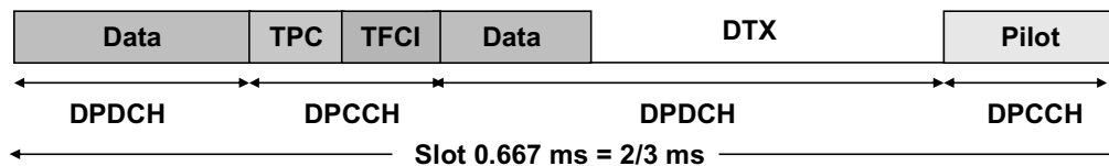
Figure 4.4 Discontinuous downlink transmission with Release 99 DCH.
