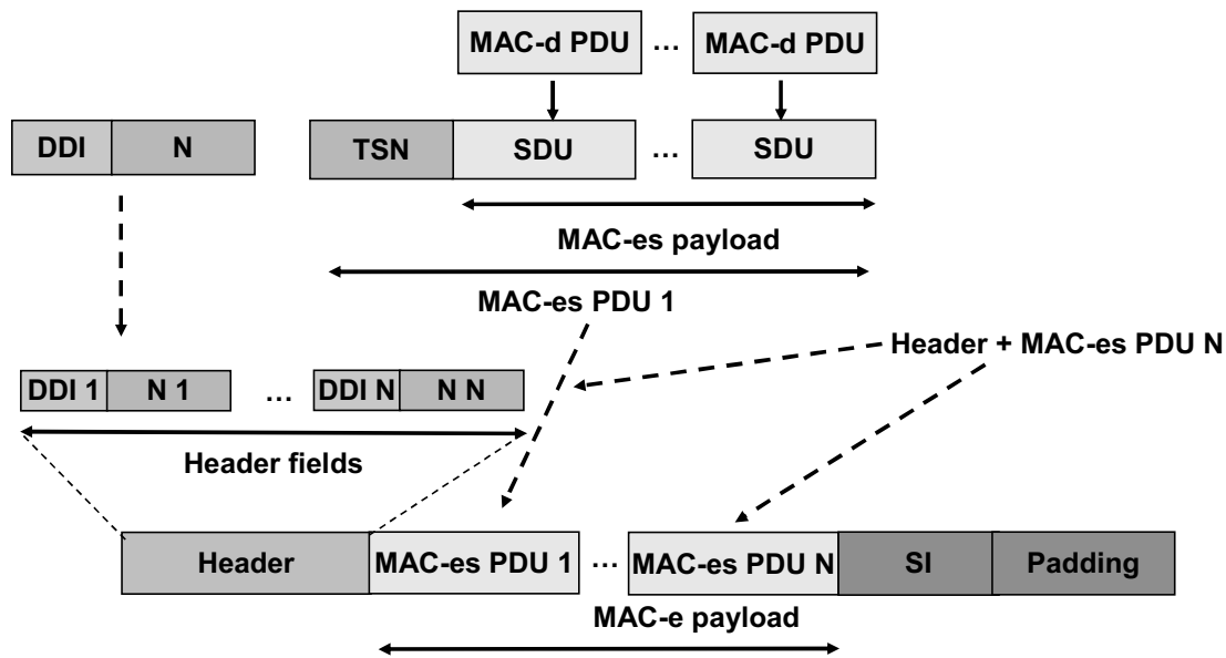
Figure 5.18 HSUPA MAC-e PDU structure.
