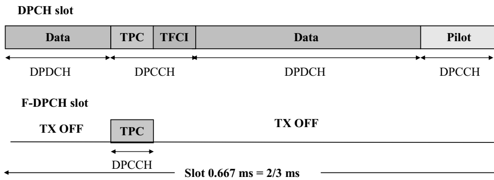
Figure 4.16 F-DPCH slot structure compared with DPCH structure.
