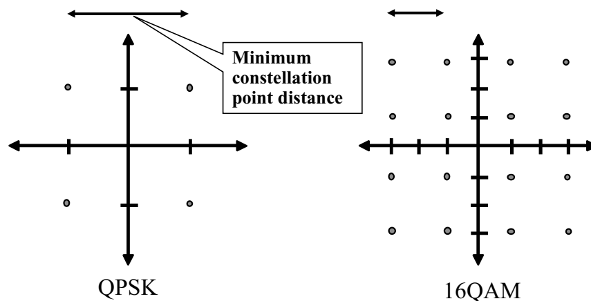
Figure 4.9 QPSK and 16QAM constellations.
