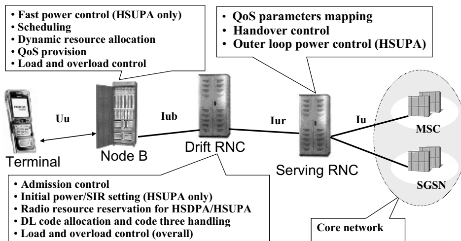
Figure 3.2 HSDPA and HSUPA RRM architecture in Release 6.
