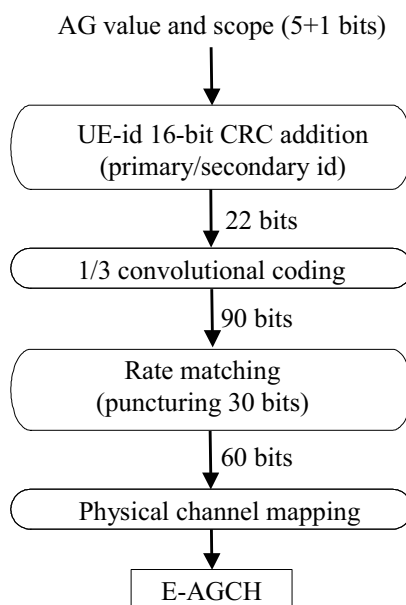
Figure 5.10 E-AGCH coding chain.
