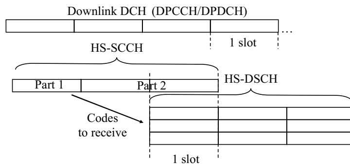
Figure 4.10 Relative timing between HS-SCCH and HS-DSCH.
