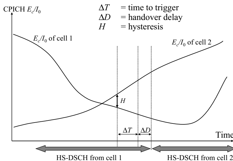
Figure 6.7 Graphical illustration of best serving HS-DSCH cell measurement from the user.
