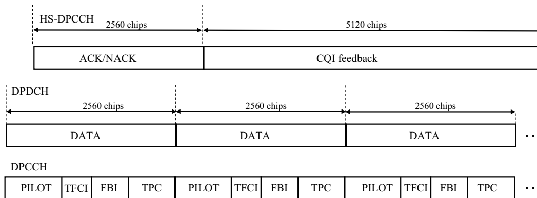
Figure 4.14 HS-DPCCH structure.
