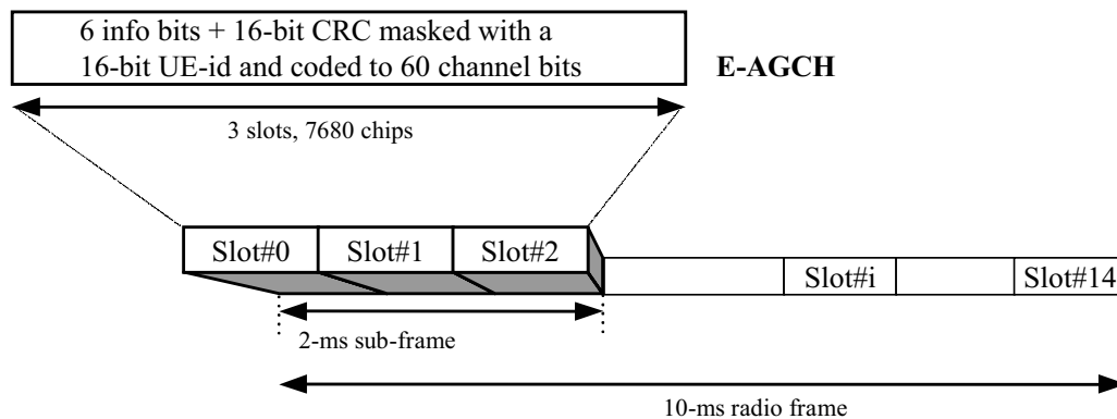
Figure 5.11 E-AGCH frame structure.
