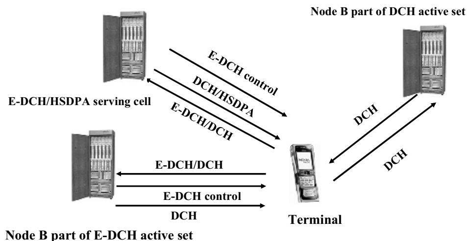
Figure 5.25 DCH and E-DCH active sets.
