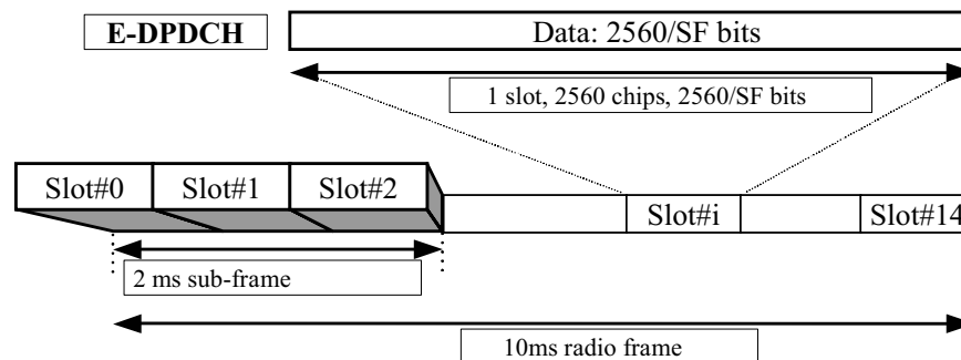
Figure 5.6 E-DPDCH frame structure.
