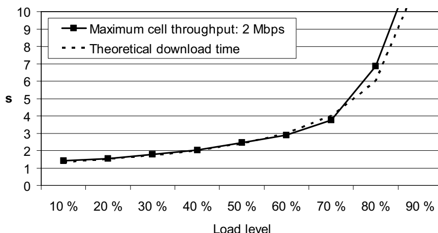
Figure 9.27 Average download time for a 300-kB Internet page as a function of load level.
