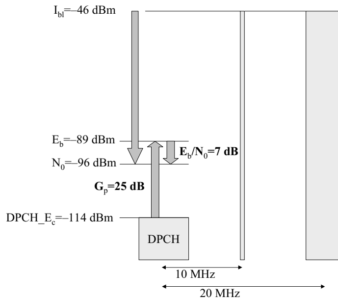
Figure 11.8 Inter-modulation test case.
