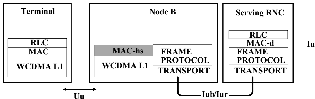
Figure 3.5 HSDPA user plane protocol architecture.
