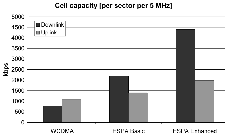
Figure 1.10 Capacity evolution with HSPA.
