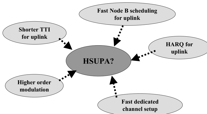
Figure 2.3 Techniques investigated for HSUPA.
