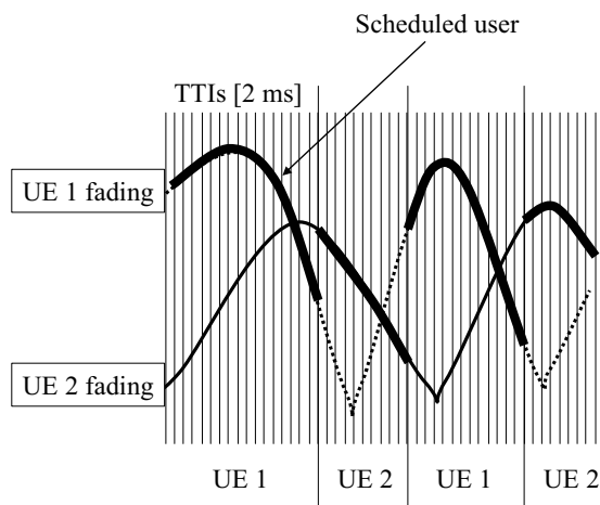
Figure 6.17 Principle underlying proportional fair scheduling with a 3-TTI delay.
