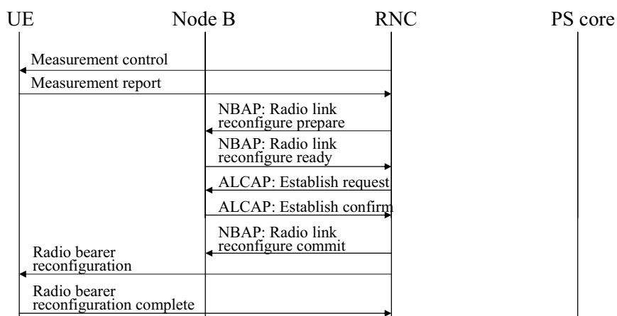
Figure 9.12 Radio bearer reconfiguration for resource allocation.
