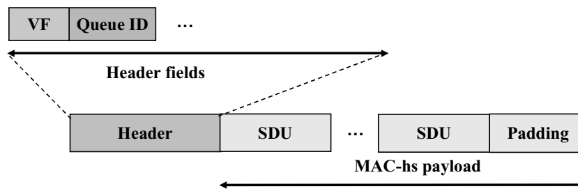
Figure 4.26 MAC-hs PDU.
