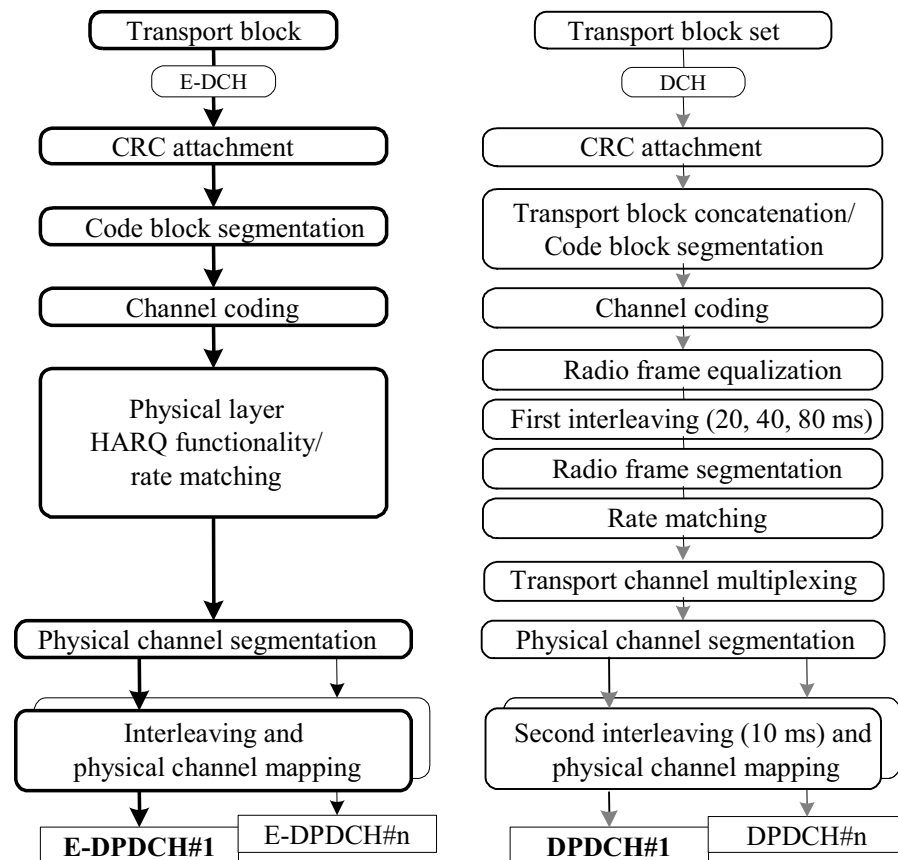
Figure 5.5 Transport channel processing details.
