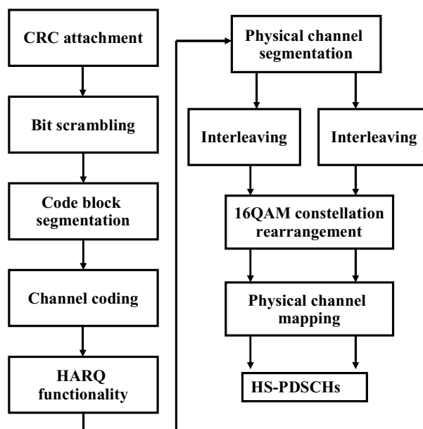
Figure 4.5 HS-DSCH channel coding chain.
