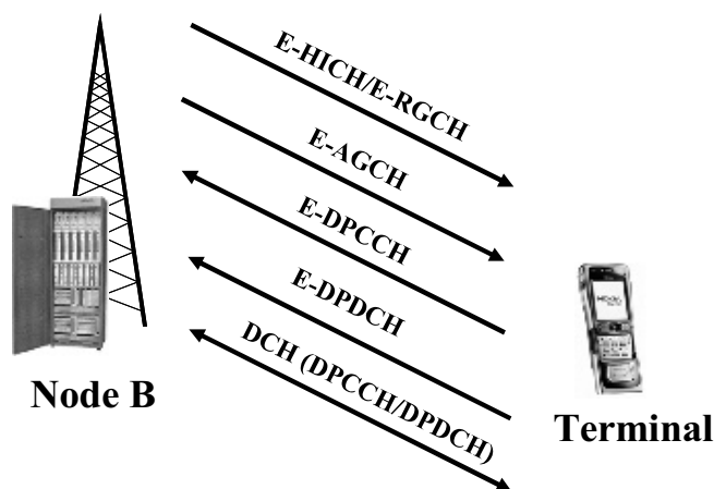
Figure 5.2 Channels needed for HSUPA operation when downlink is on the Release 99 DCH.
