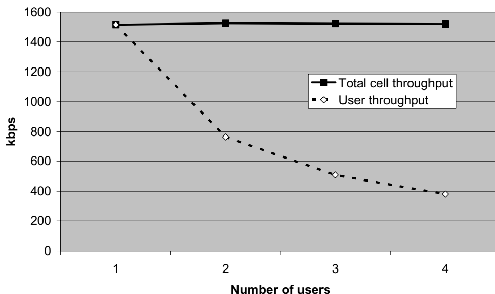
Figure 7.34 Multiuser measurements.
