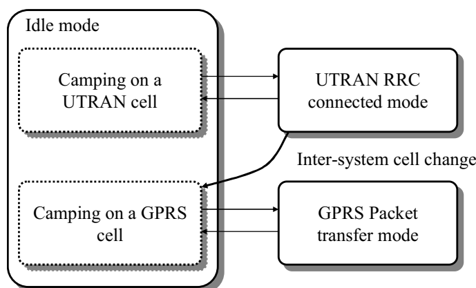
Figure 9.8 Inter-system cell change from HSPA to GPRS.
