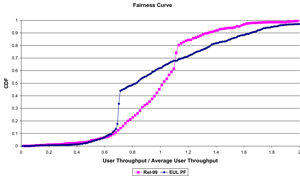
Figure 9.6.1.2.4: Fairness curves for EUL and Rel-99
