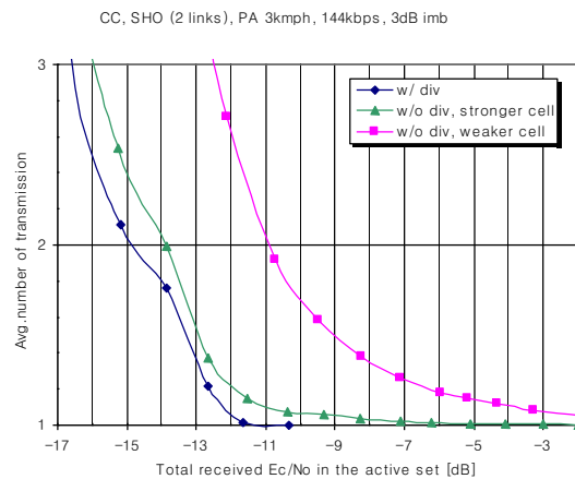
Figure 9.2.11. Average number of transmissions in soft handover with 3dB link imbalance in PA 3kmph
