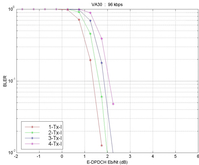
Figure A.2.2.1.4: 96 kbps – VA30
