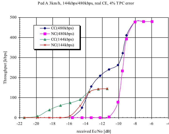
Figure 9.2.1. Throughput in Pedestrian A 3 km/h with power control
