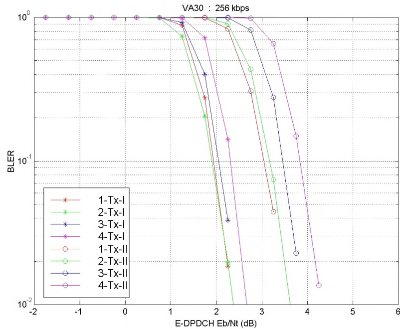
Figure A.2.2.1.6: 256 kbps – VA30
