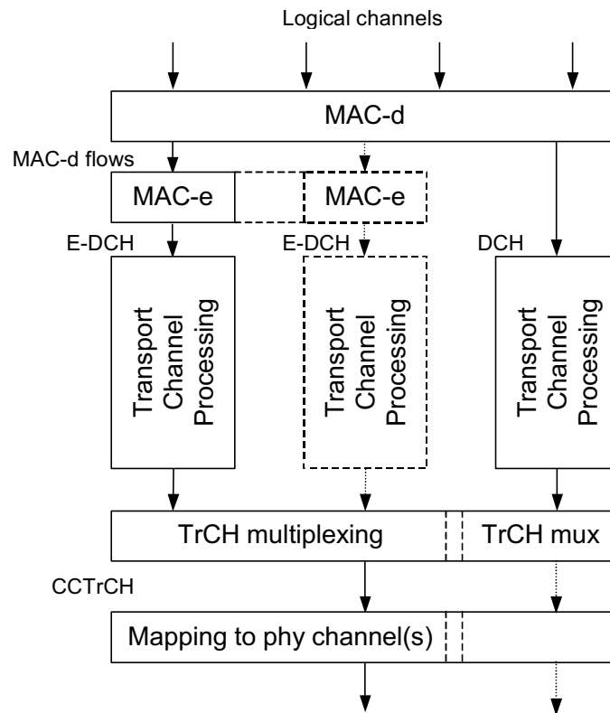
Figure 8.1.1: Simplified illustration of possible transport channel structures.
