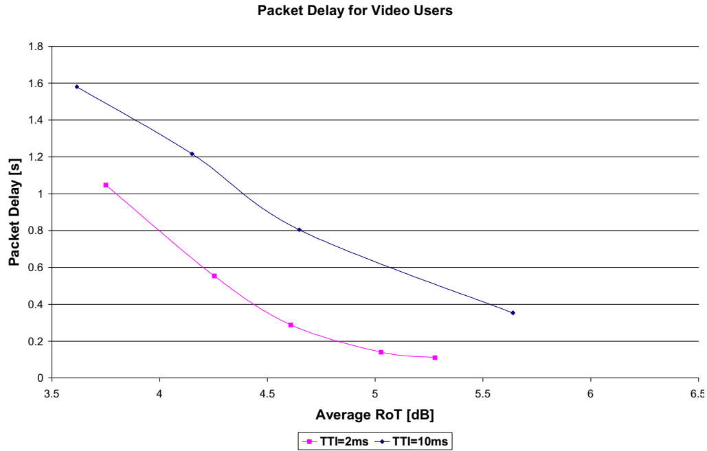
Figure 9.4.1.2.7: Average packet delay for Video users
