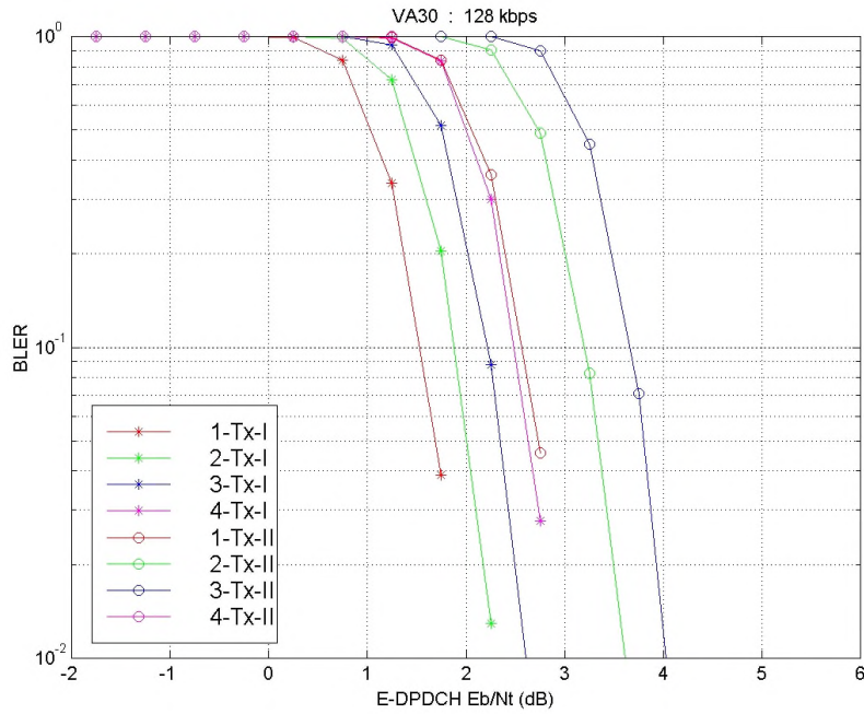
Figure A.2.2.1.5: 128 kbps – VA30
