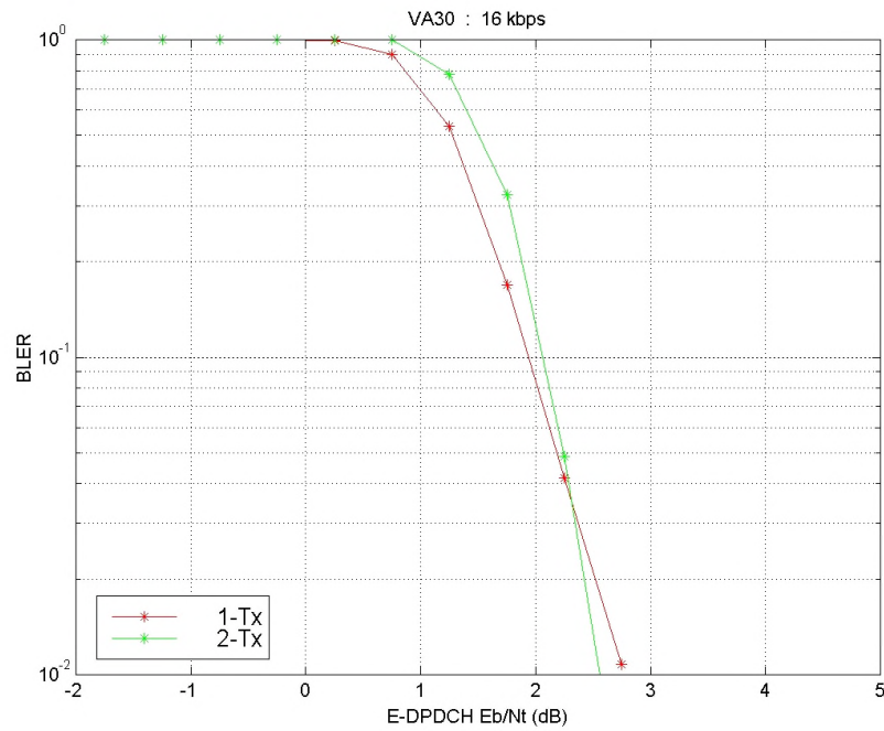
Figure A.2.2.2.1: 16 kbps – VA30
