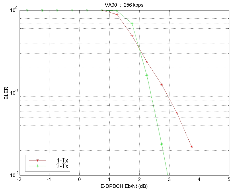
Figure A.2.2.2.5: 256 kbps – VA30
