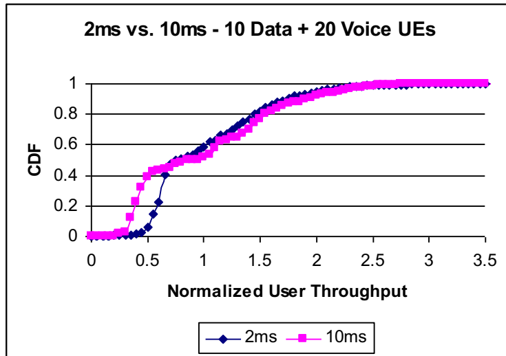
Figure 9.4.1.3.4: Fairness curves - mixed channel
