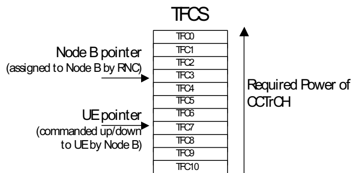
Figure 7.1.1: Depiction of the TFC pointers
