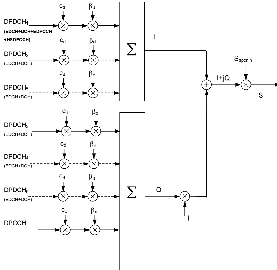
Figure 8.4.11. Case 3: Structure for Enhanced Uplink
