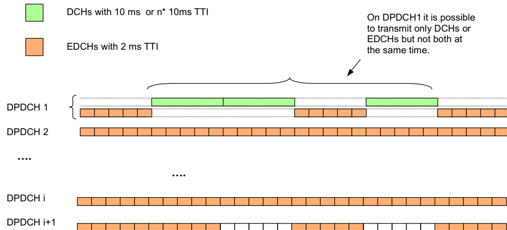
Figure 8.4.5. An example showing code multiplexing with UE capability defined in a combined fashion for E-DCH and DCH, with minimum TTI=2ms for E-DCH.
