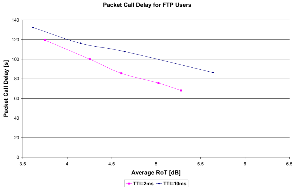
Figure 9.4.1.2.4: Average packet call delay for FTP users
