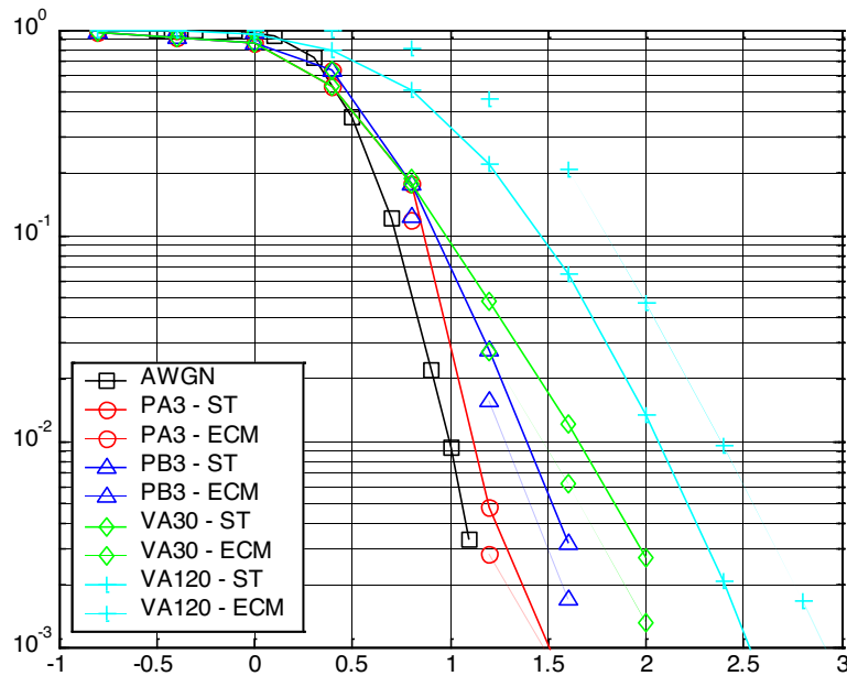
Figure A.1.4.3; Comparison of actual short-term and ECM generated curves – 192 kbps, R=0.4 , BPSK, TTI=10\text{ms} , SF=8 , ideal channel estimation, Q=1.0 for PA3, PB3, Q=2.0 for VA30, VA120.
