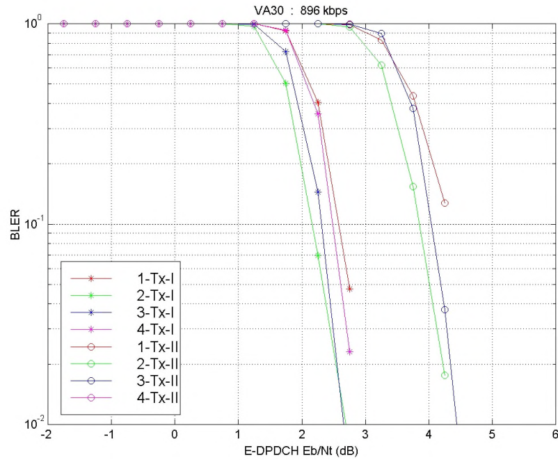
Figure A.2.2.1.11: 896 kbps – VA30
