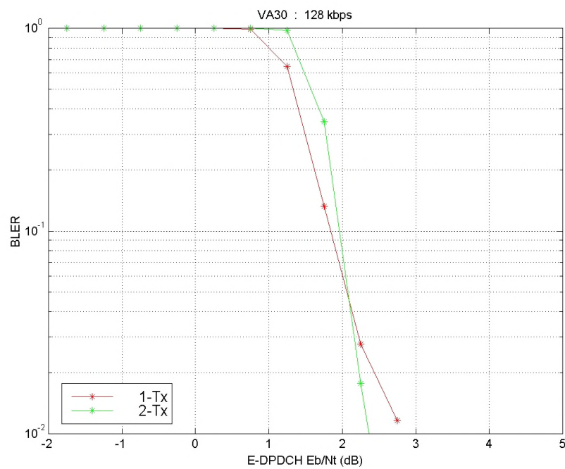
Figure A.2.2.2.4: 128 kbps – VA30
