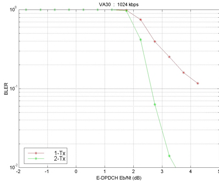
Figure A.2.2.2.7: 1024 kbps – VA30
