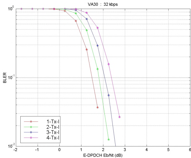
Figure A.2.2.1.2: 32 kbps – VA30
