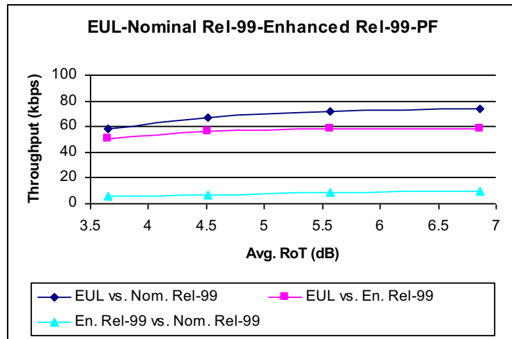
Figure 9.6.1.1.10: Throughput gain between EUL and Rel-99 - PF
