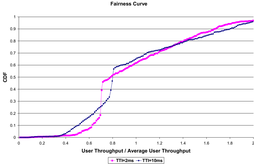
Figure 9.4.1.2.3: Fairness curves
