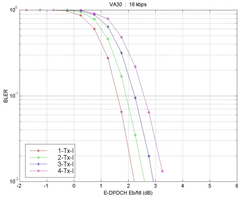
Figure A.2.2.1.1: 16 kbps – VA30
