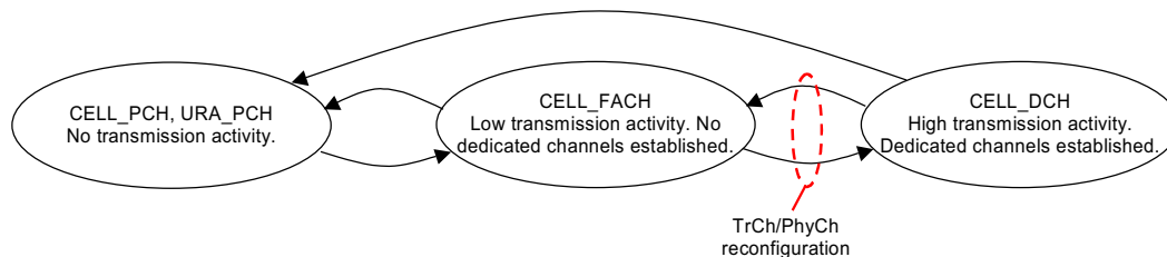
Figure 6.1.1: Connection states.
