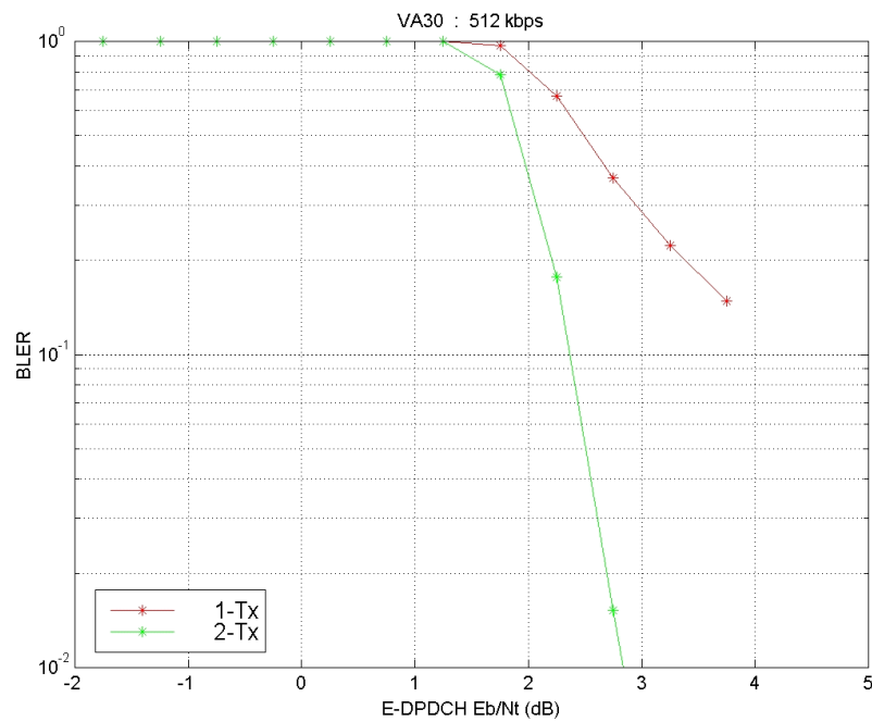
Figure A.2.2.2.6: 512 kbps – VA30
