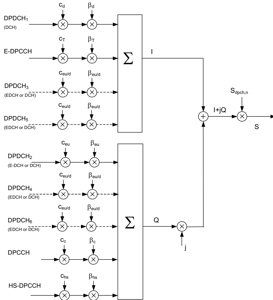
Figure 8.4.9. Case 1: Structure for Enhanced Uplink
