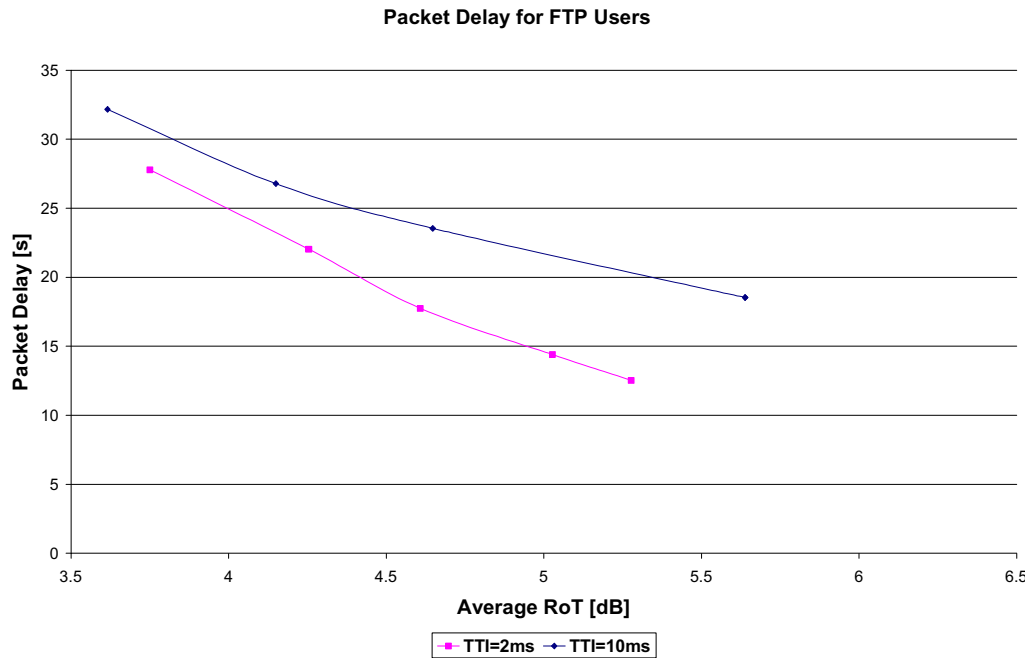
Figure 9.4.1.2.6: Average packet delay for FTP users
