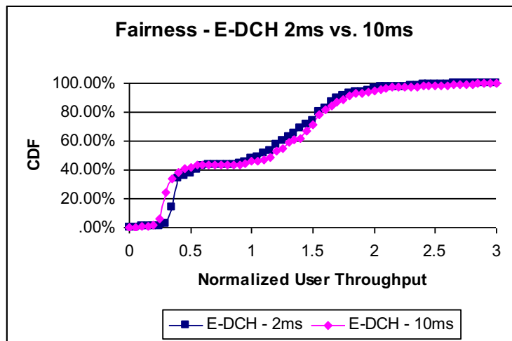
Figure 9.4.1.1.3: Fairness curves - mixed channel
