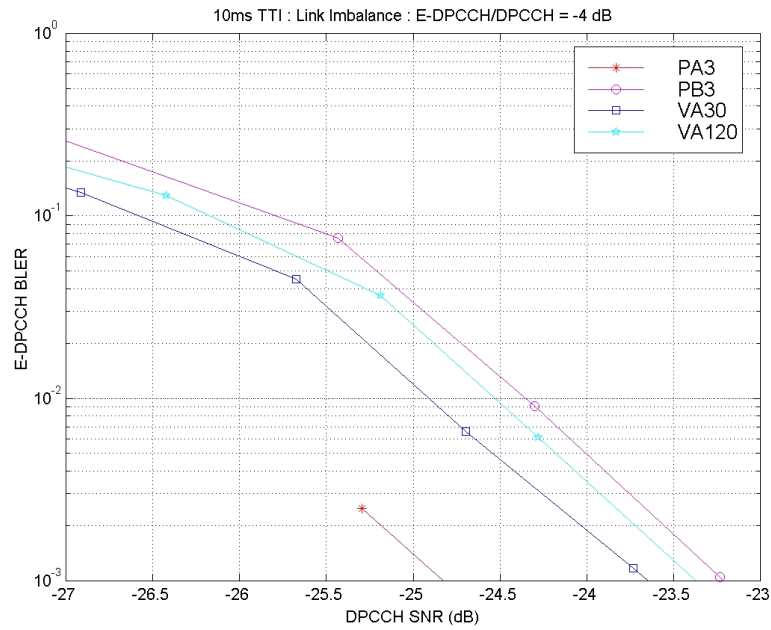
Figure 9.2.4.2: E-DPCCH/DPCCH = -4 dB
