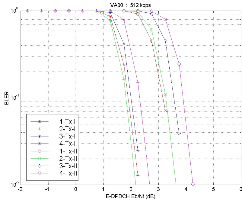
Figure A.2.2.1.8: 512 kbps – VA30
