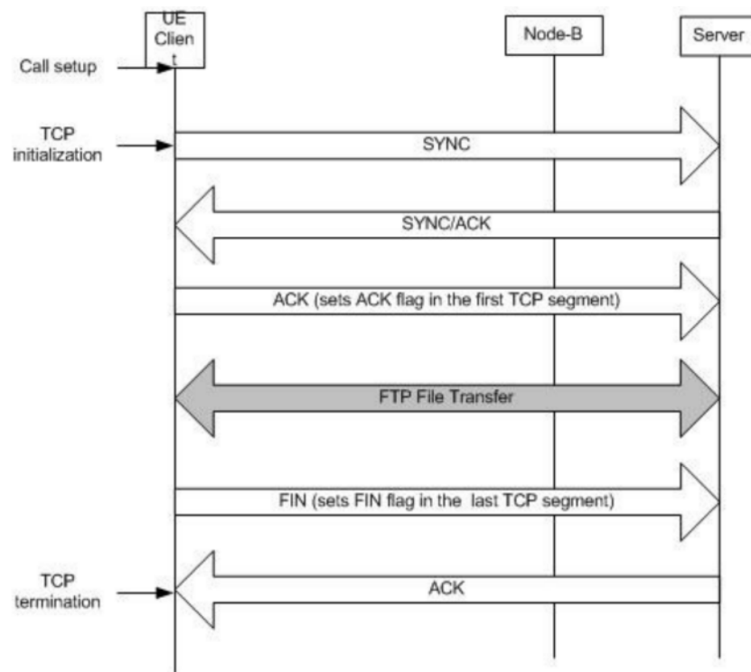
Figure A-7: Modeling of TCP three-way handshake
