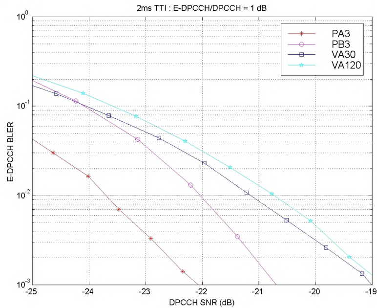
Figure 9.2.4.5: E-DPCCH/DPCCH = 1 dB
