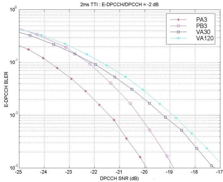
Figure 9.2.4.4: E-DPCCH/DPCCH = -2 dB
