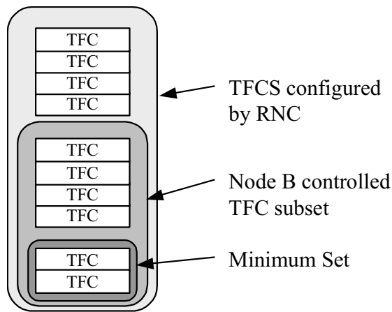
Figure 7.1 : Illustration of different sets of TFCs.
