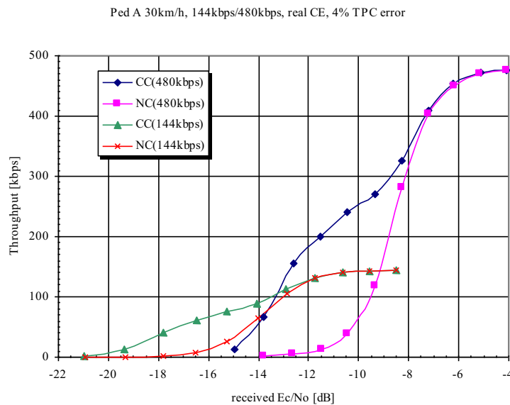
Figure 9.2.2. Throughput in Pedestrian A 30 km/h with power control
