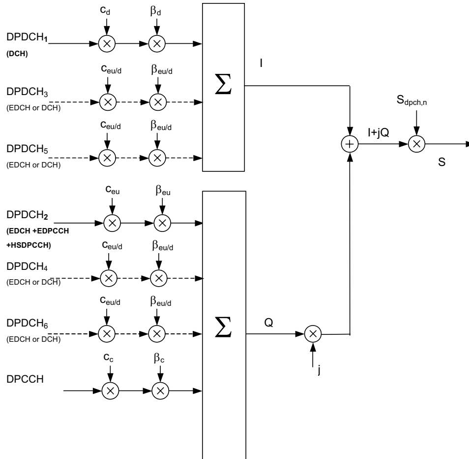
Figure 8.4.12. Case 4: Structure for Enhanced Uplink
