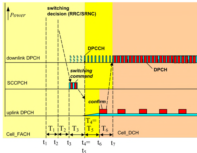
Figure 7.3.1: Enhanced procedure for DCH establishment.
