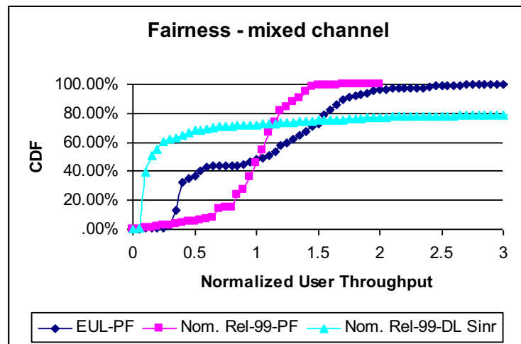
Figure 9.6.1.1.3: Fairness curves - mixed channel
