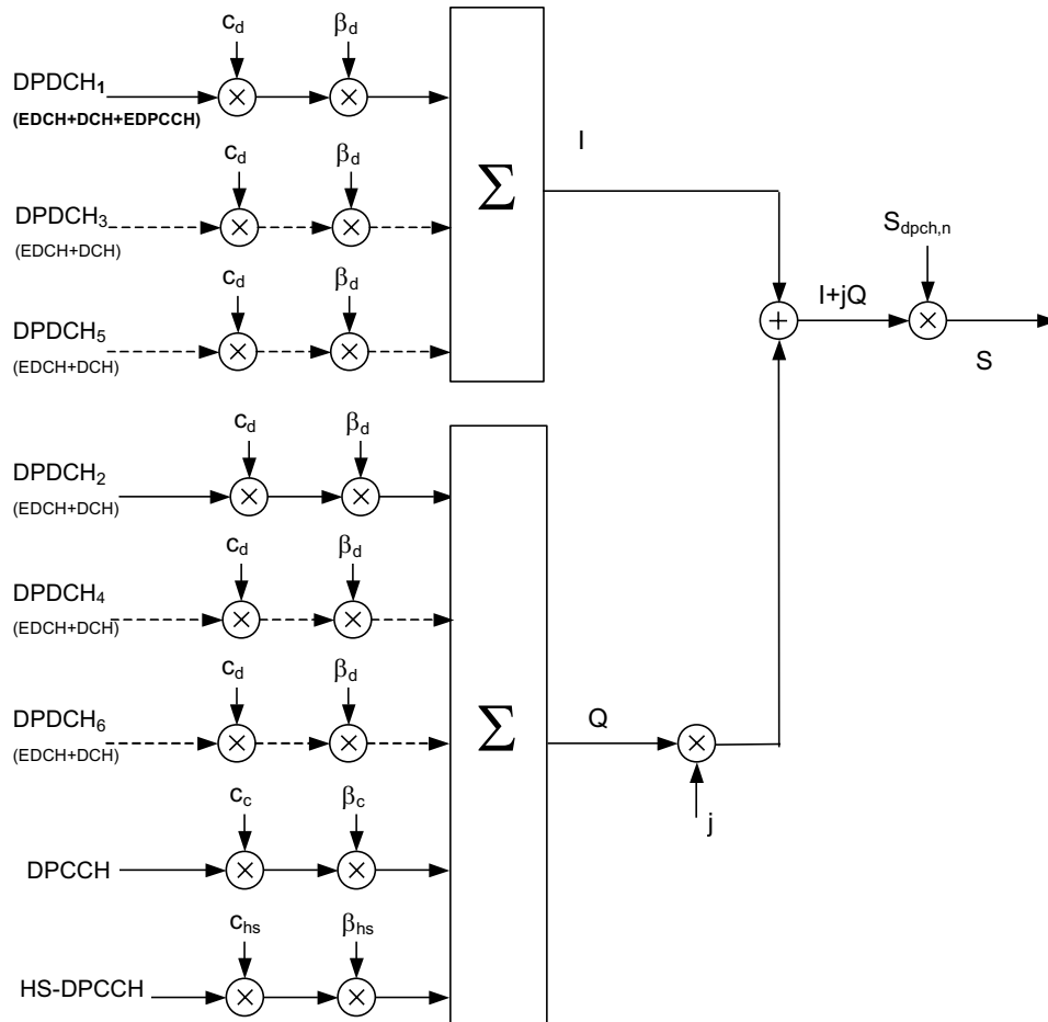
Figure 8.4.10. Case 2: Structure for Enhanced Uplink
