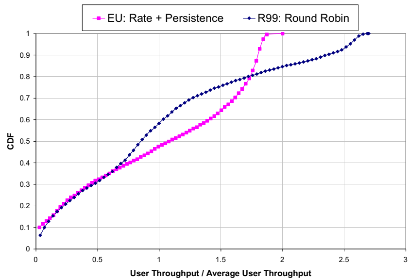
Figure 9.6.2.5 Gaming Traffic Fairness curves for PB3
