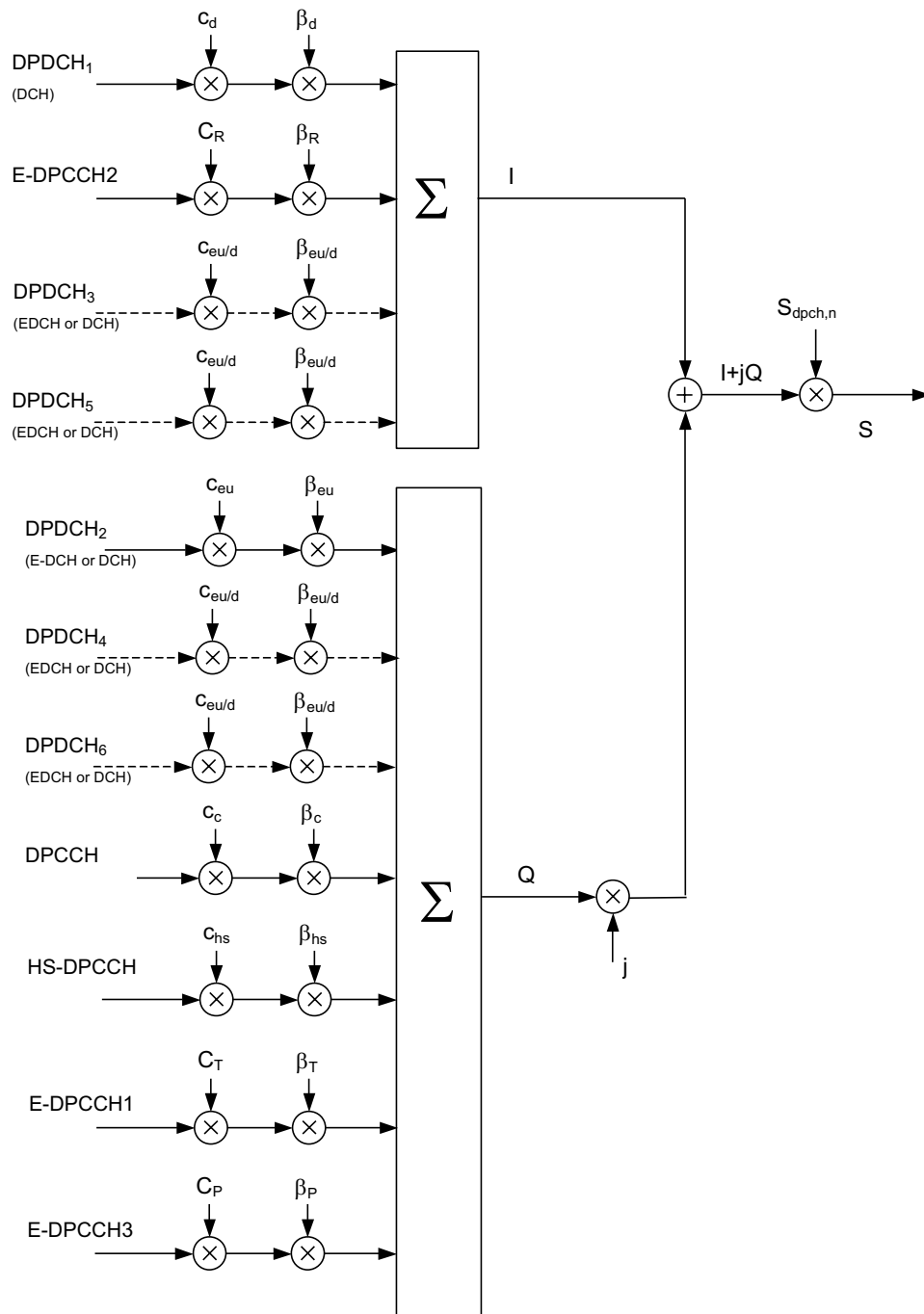
Figure 8.4.13 Case 8: Structure for Enhanced Uplink
