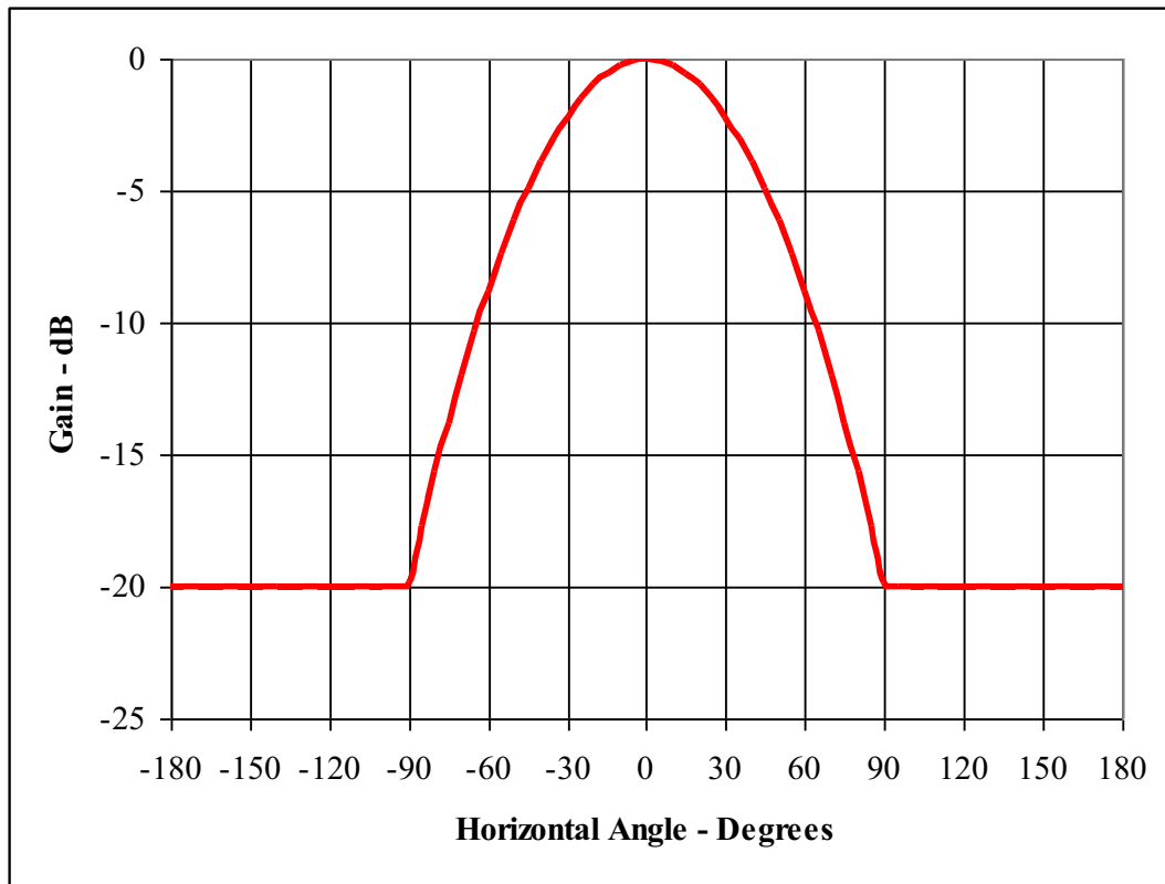
Figure A - 1 - Antenna Pattern for 3-Sector Cells
