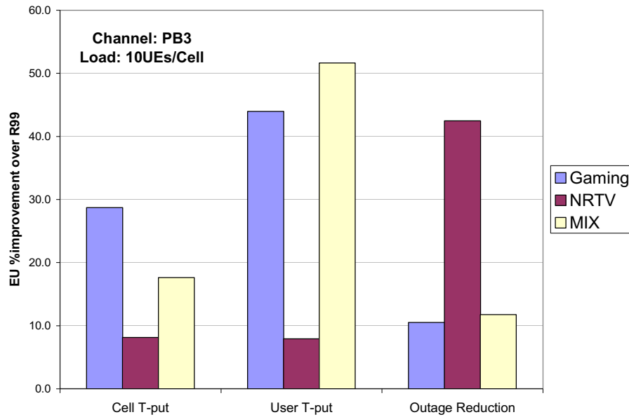
Figure 9.6.2.3: E-DCH improvement over DCH for similar RoT
