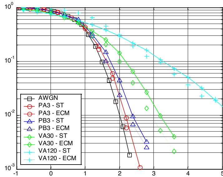
Figure A.1.4.2; Comparison of actual short-term and ECM generated curves – 480 kbps, R=0.5 , BPSK, TTI=2\text{ms} , SF=4 , ideal channel estimation, Q=1.0 for PA3, PB3, Q=2.0 for VA30, VA120.
