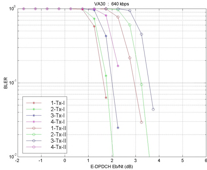
Figure A.2.2.1.9: 640 kbps – VA30
