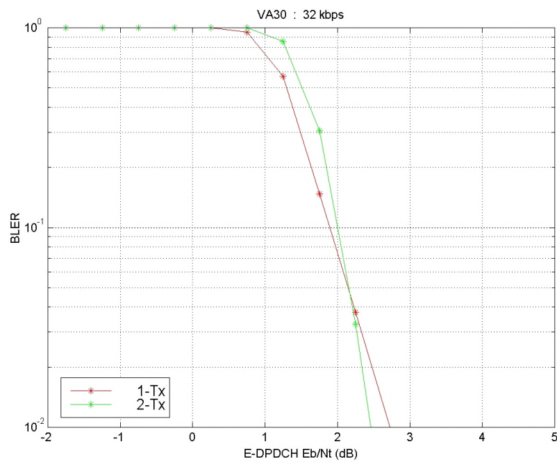
Figure A.2.2.2.2: 32 kbps – VA30
