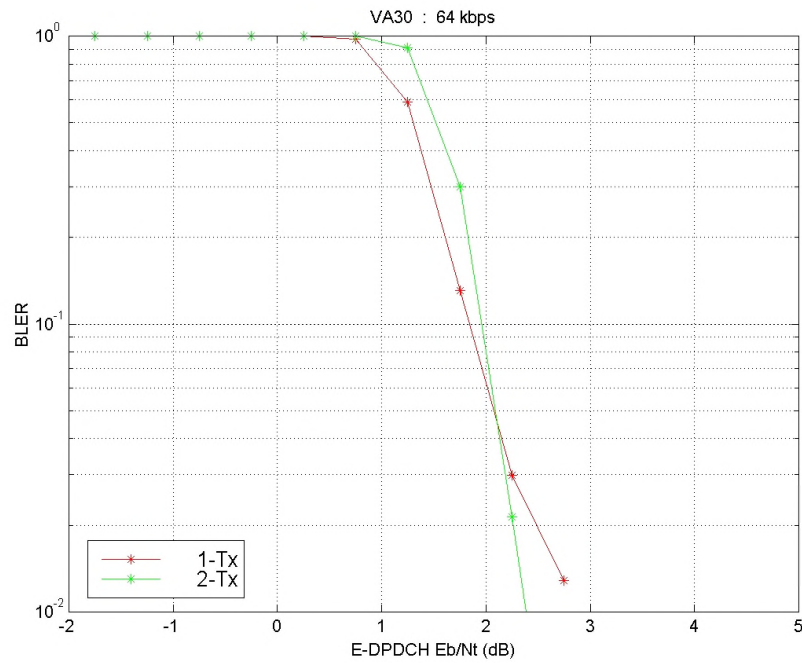
Figure A.2.2.2.3: 64 kbps – VA30
