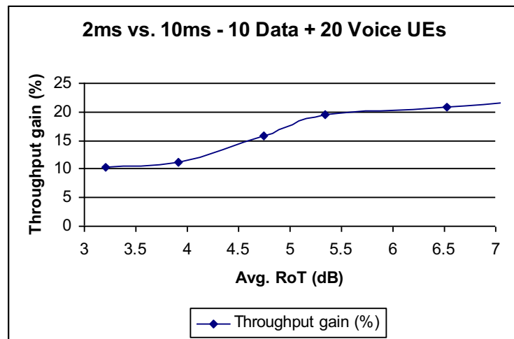
Figure 9.4.1.3.2: Throughput gain between 2ms and 10ms
