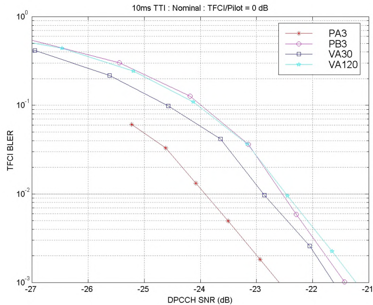
Figure 9.2.4.3: TFCI/DPCCH = 0 dB
