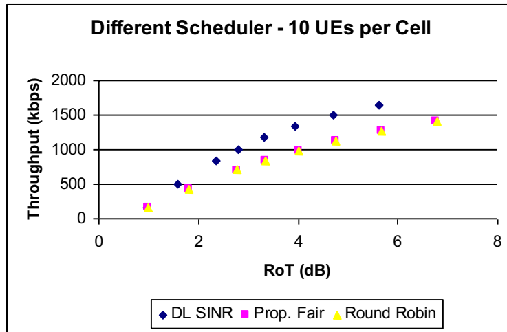
Figure A.4.1.1.3.3 Average cell throughput as a function of RoT -- 10 UEs per cell
