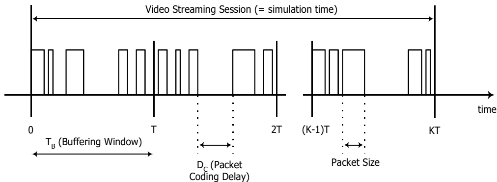
Figure A - 5 - Video Streaming Traffic Model
