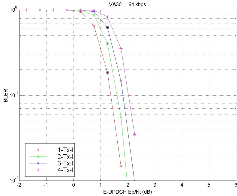
Figure A.2.2.1.3: 64 kbps – VA30
