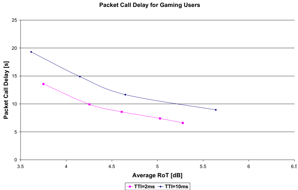
Figure 9.4.1.2.5: Average packet call delay for Gaming users
