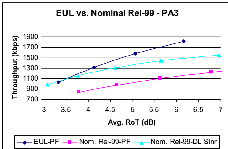
Figure 9.6.1.1.5 Average cell throughput as a function of average RoT – PA3
