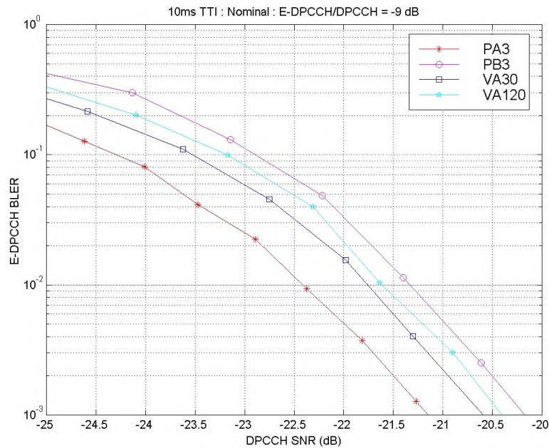
Figure 9.2.4.1 E-DPCH/DPCH = -9 dB
