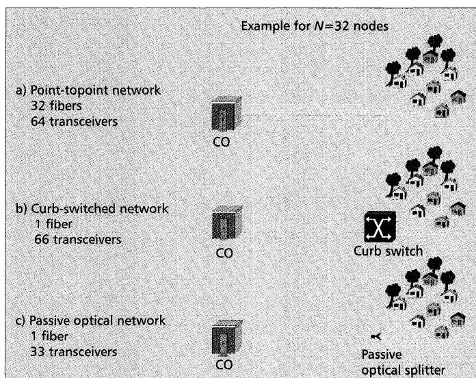
■ Figure 2. Fiber to the home (FTTH) deployment scenarios.
