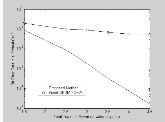
Figure 4: Performance comparison between proposed method and fixed OFDM-FDMA scheme
