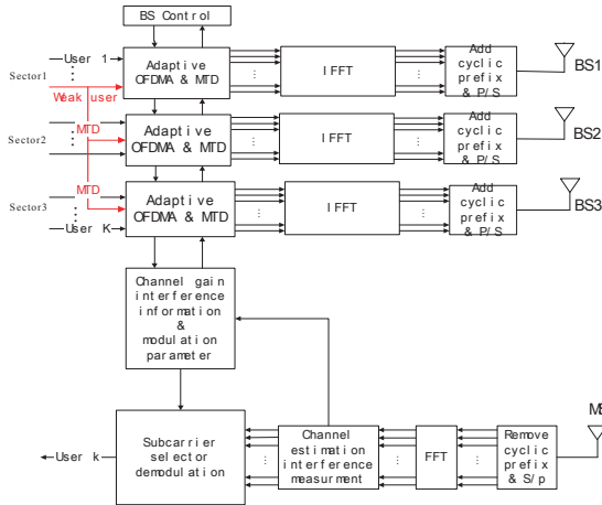
Figure 3: Adaptive resource allocation OFDMA with Macro Transmit Diversity in a “virtual cell”
