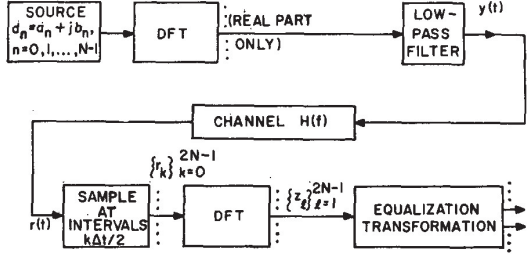
Fig. 4. Fourier transform communication system including linear channel distortion and final equalization.
