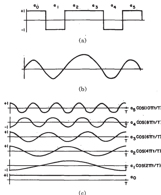
Fig. 1. Comparison of waveforms in serial and parallel data transmission systems. (a) Serial stream of six binary digits. (b) Typical appearance of baseband serial transmission. (c) Typical appearance of waveforms that are summed to create parallel data signals.
