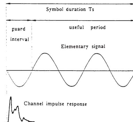
Figure 3 Use of a guard interval to suppress the intersymbol interference
