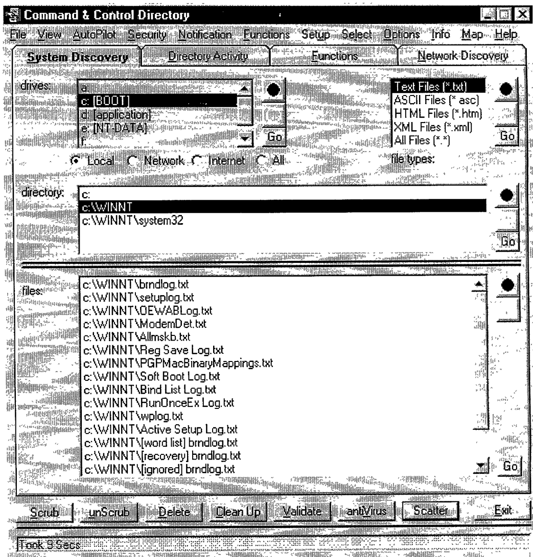
Figure 28. Command and Control local disk management in process.
