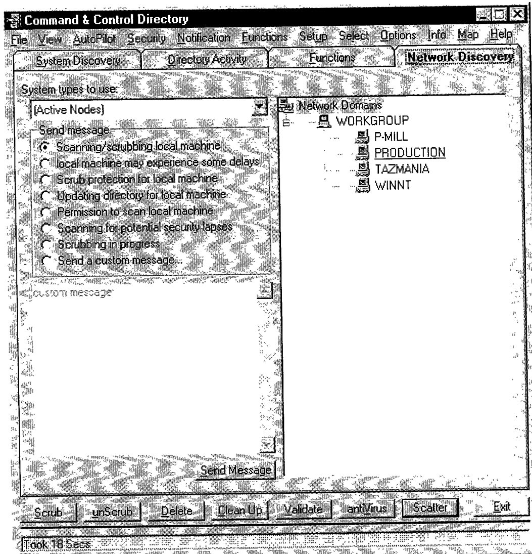
Figure 10. Network resources management.
