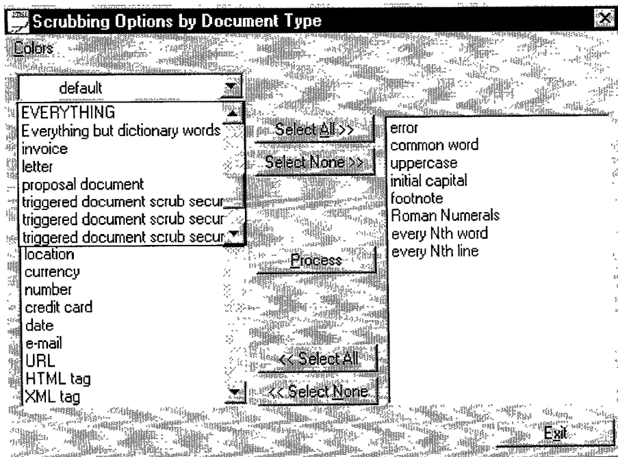
Figure 12. Selection of categories for document type scrubbing.
