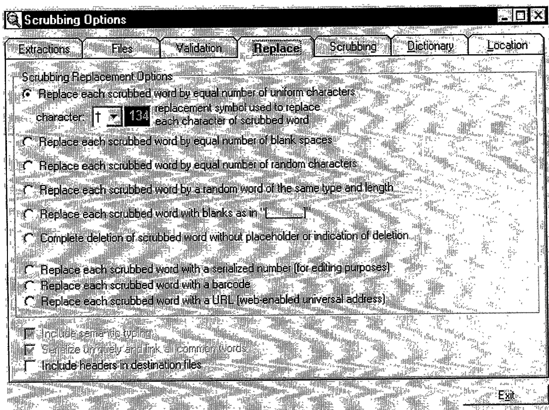
Figure 20. Output extraction display options.
