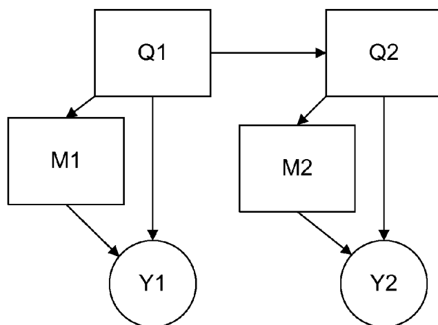
HMM with mixture of Gaussians output
