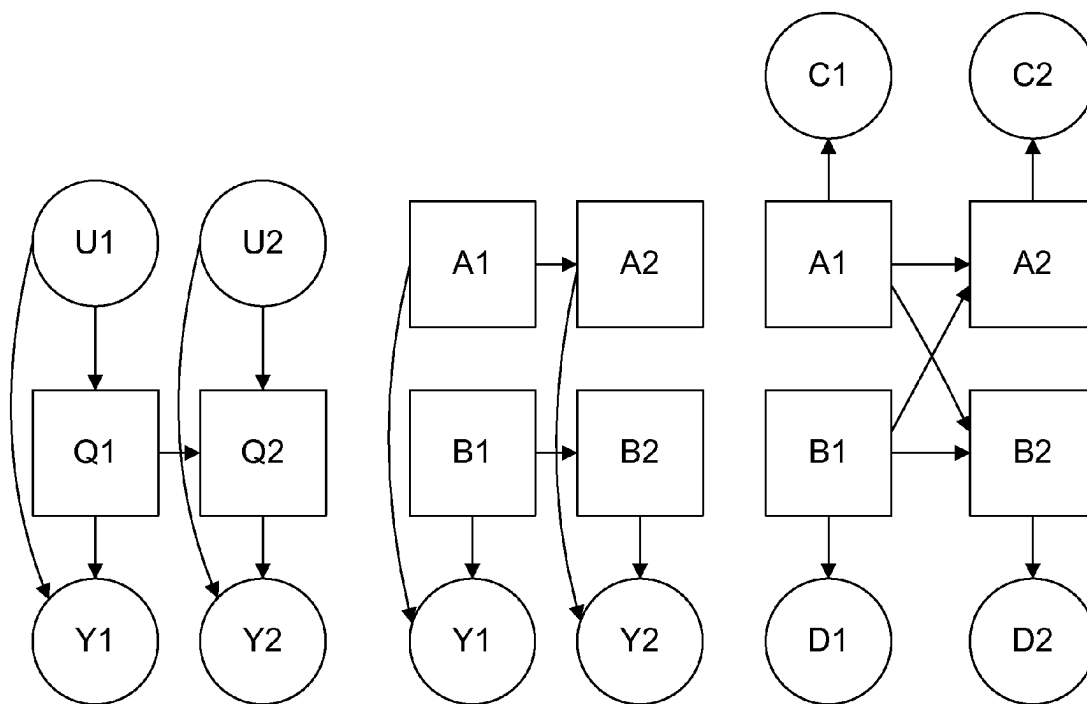
Input-output HMM Fig. 4A
