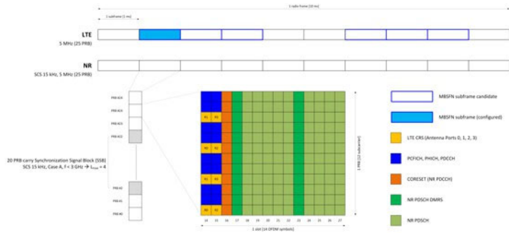
Figure 1 NR signal configuration within the MBSFN subframe.
