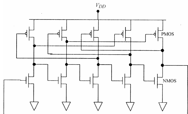
Fig. 2 — Five stages negative skewed delay ring oscillator
