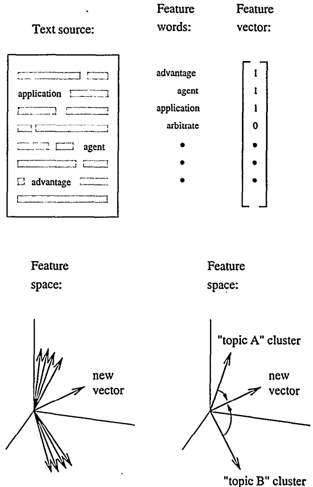
Figure 1: Nearest Neighbor Approach. In one common Information Retrieval approach, feature words are chosen and counted to produce a feature vector. The feature vectors of similar documents may be clustered to produce a prototype or category vector. Given query or a new document to classify, the system chooses the category nearest to the query vector. The dimension of the vector space is equal to the number of feature words, often in the thousands.
