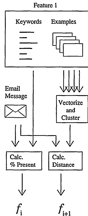
Figure 4: Feature Extraction. Features may contain keywords and/or example emails. To determine the feature vector on which the learner will operate, the mail is vectorized. If the feature uses keywords, the percentage of keywords present in the email is calculated and output. If there are example emails, they are vectorized and clustered; the distance between the email and the cluster center is then calculated and output. These two outputs are used as elements of the feature vector.
