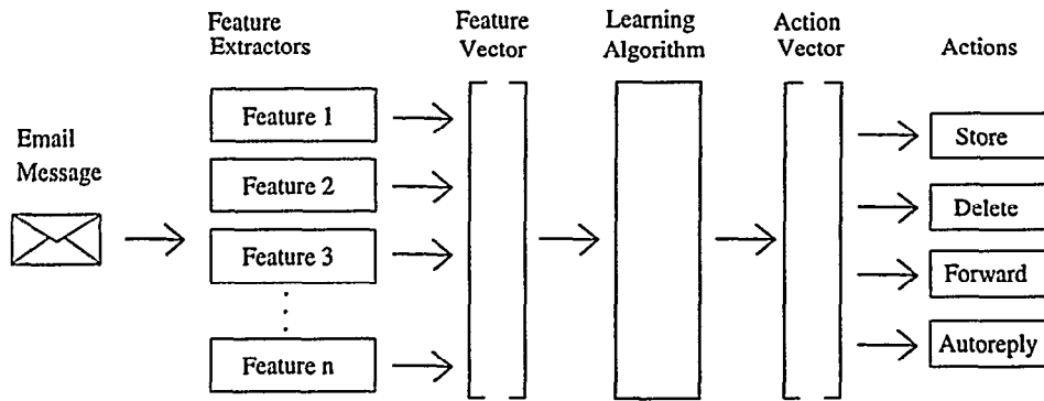
Figure 3: Agent Architecture. Our system extracts features from the email that can be used by a learner to determine output actions. Note that learning occurs in two places. The agent first learns what features to extract from email. It then uses the extracted features to learn what to do with the mail.
