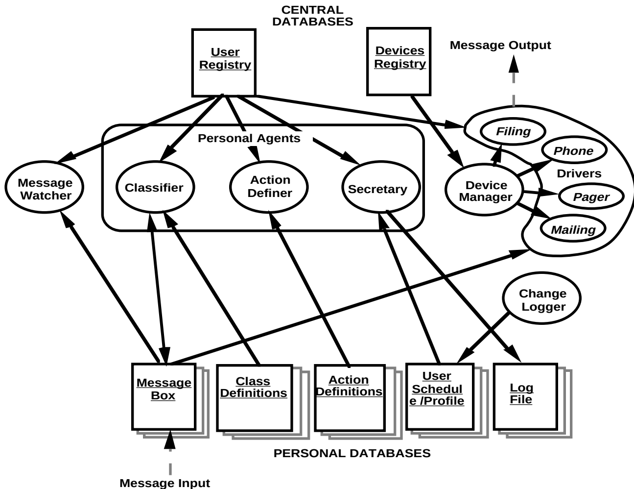
Figure 3. Processes and the Lotus Notes Databases.
