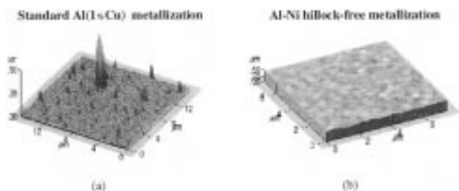
Fig. 4. Comparison of AFM pictures of (a) an Al film and (b) an Al — Ni film after both films were heated at 500 °C. It is clear that the Al-Ni film resists the formation of hillocks.
