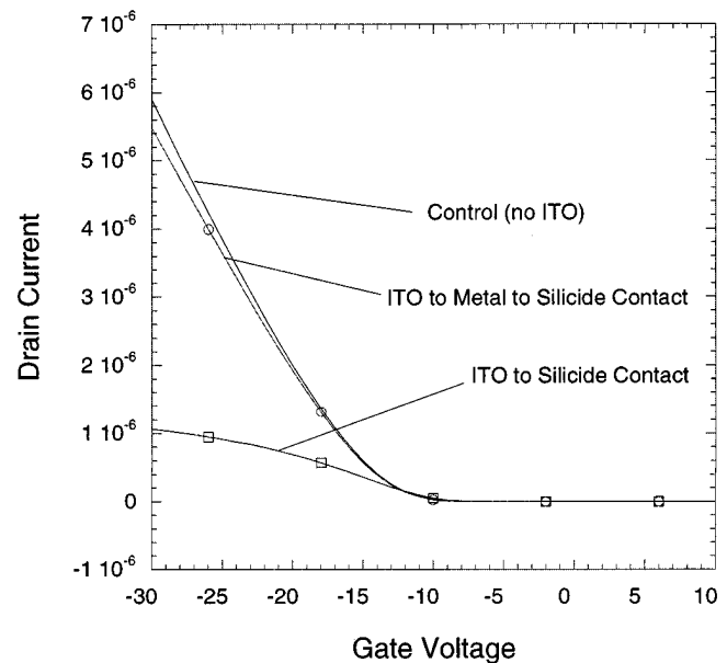
Fig. 8. TFT transfer characteristics comparing a TFT using an ITO-metal-silicide contact scheme with a TFT using an ITO-silicide contact scheme.
