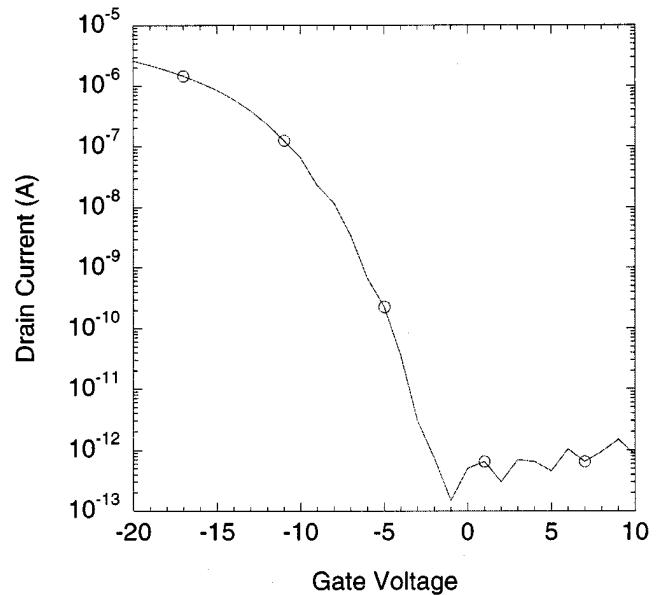
Fig. 11. P-channel pixel TFT transfer characteristics. W/L = 4 \mu\text{m}/8 \mu\text{m} , V_{DS} = -1 V.
