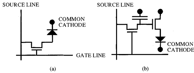
Fig. 1. Pixel design schematics showing (a) the single TFT per pixel design, and (b) the two TFT per pixel design.
