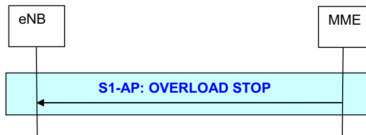
Figure 19.2.2.12.2-1: Overload Stop procedure
