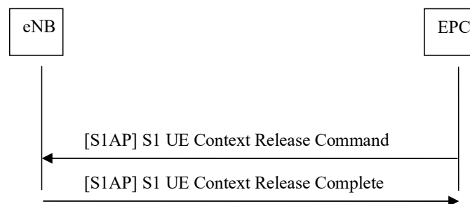
Figure 19.2.2.2.1-1: S1 UE Context Release procedure (EPC triggered)
