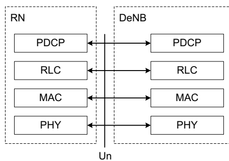
Figure 4.7.5-2: User plane protocol stack for supporting RNs
