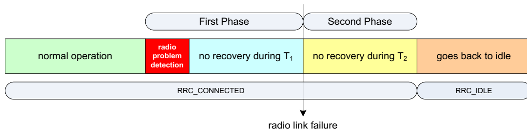
Figure 10.1.6-1: Radio Link Failure
