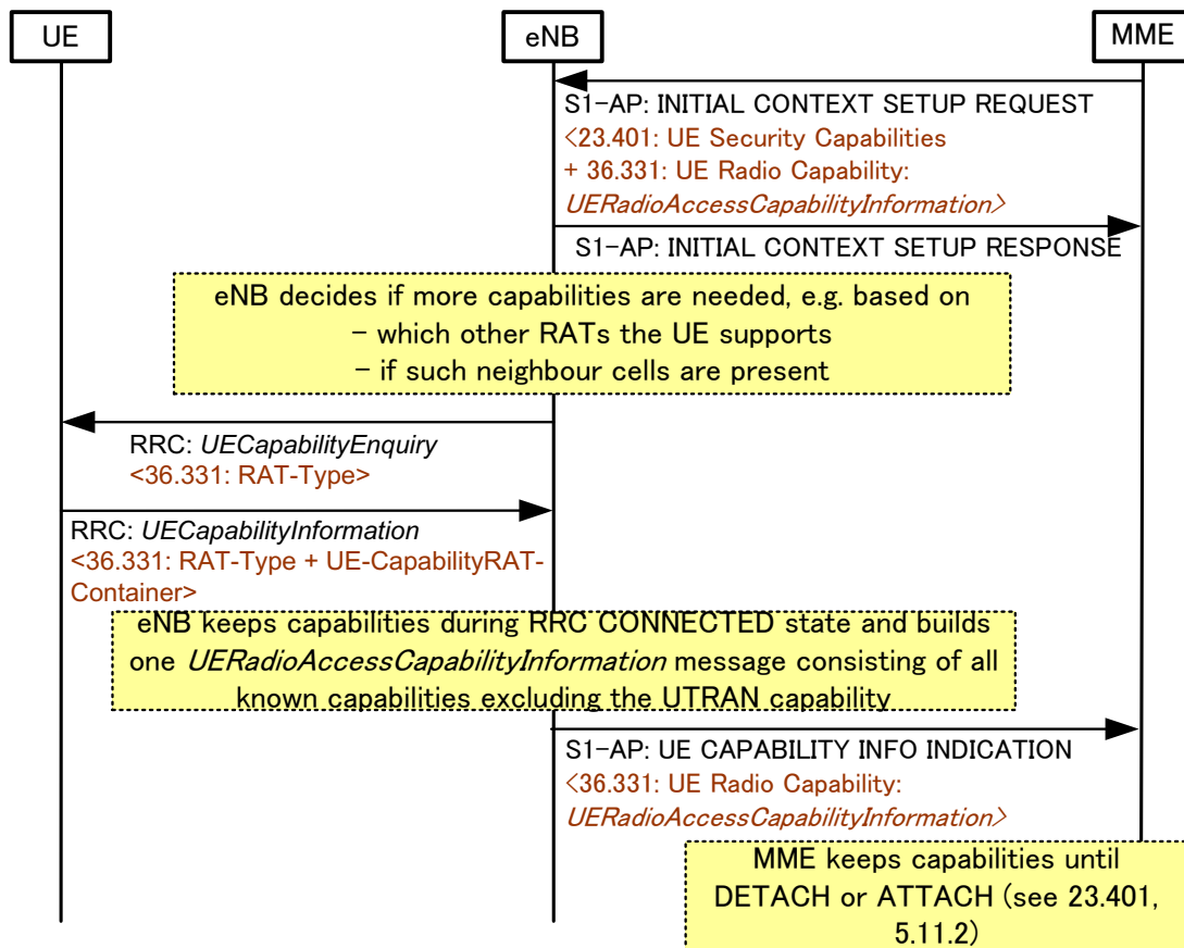
Figure 18-1: Initial UE Capability Handling
