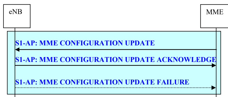
Figure 19.2.2.10-1: MME Configuration Update procedure
