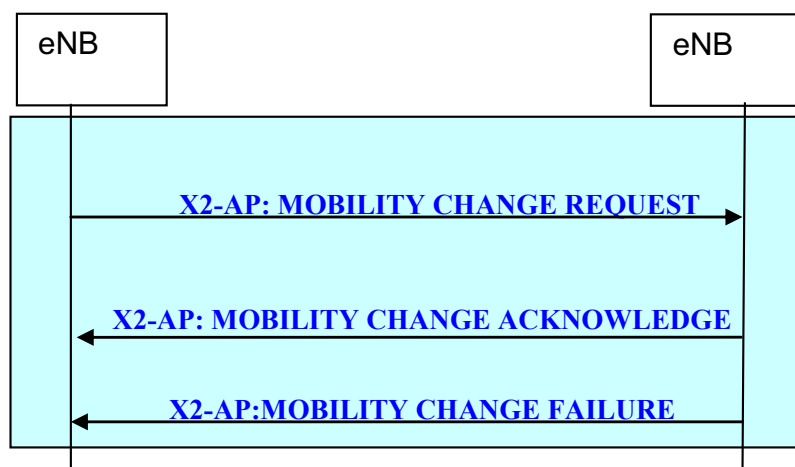
Figure 20.2.2.14-1: Mobility Settings Change procedure
