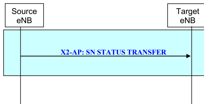
Figure 20.2.2.4-1: SN Status Transfer procedure
