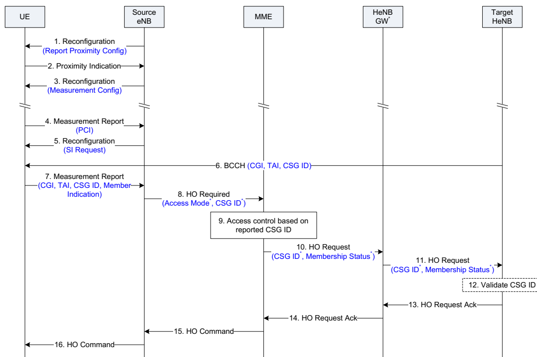
Figure 10.5.1.2-1: Mobility to HeNB's CSG and hybrid cells.
