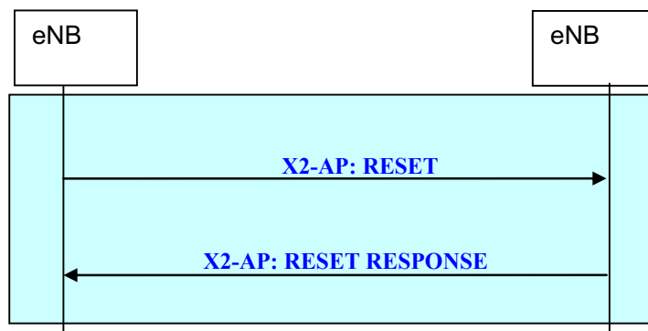
Figure 20.2.2.9-1: Reset procedure
