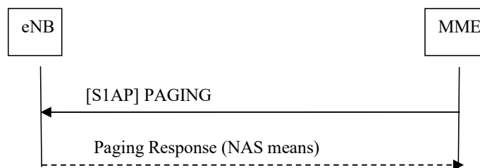
Figure 19.2.2.1-1: Paging procedure
