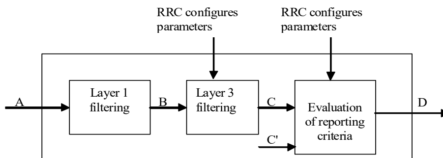
Figure 10.6-1: Measurement model
