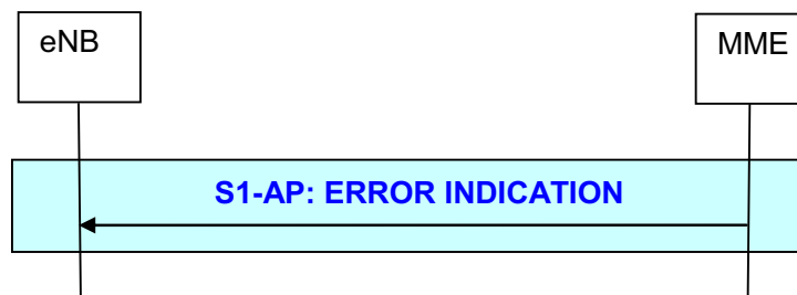
Figure 19.2.2.7.2b-1: MME initiated Error Indication procedure
