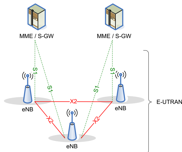
Figure 4-1: Overall Architecture
