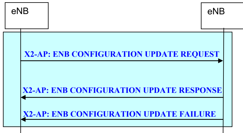
Figure 20.2.2.8-1: eNB Configuration Update procedure
