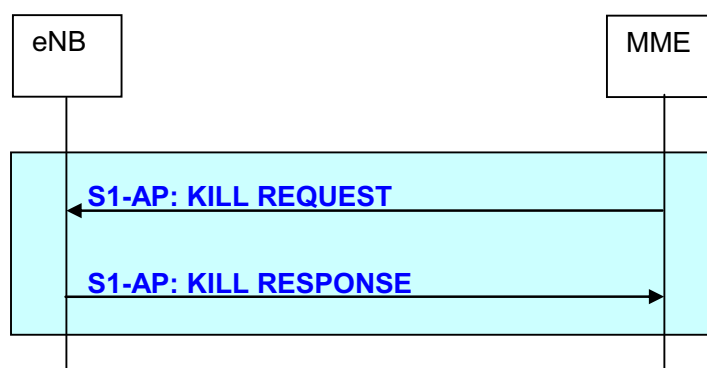
Figure 19.2.2.17-1: Kill procedure
