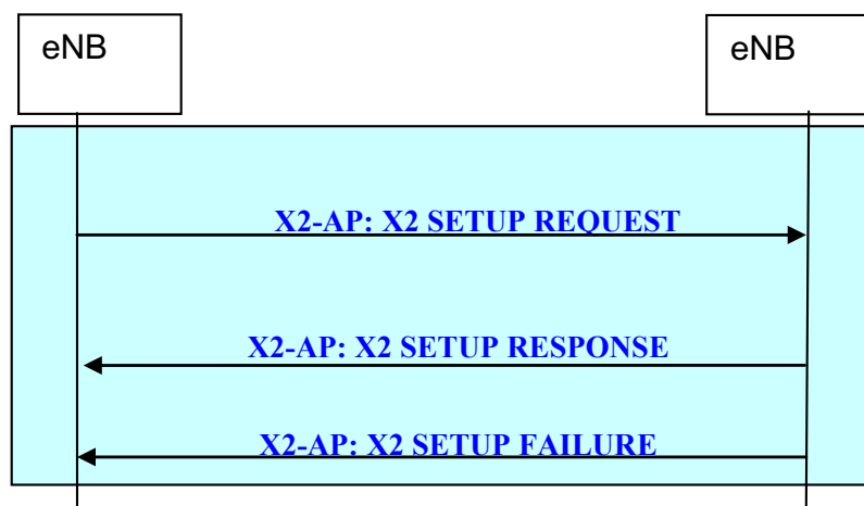
Figure 20.2.2.7-1: X2 Setup procedure
