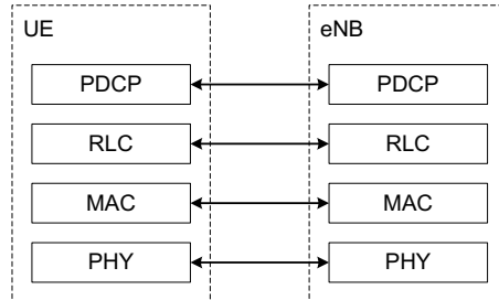
Figure 4.3.1-1: User-plane protocol stack
