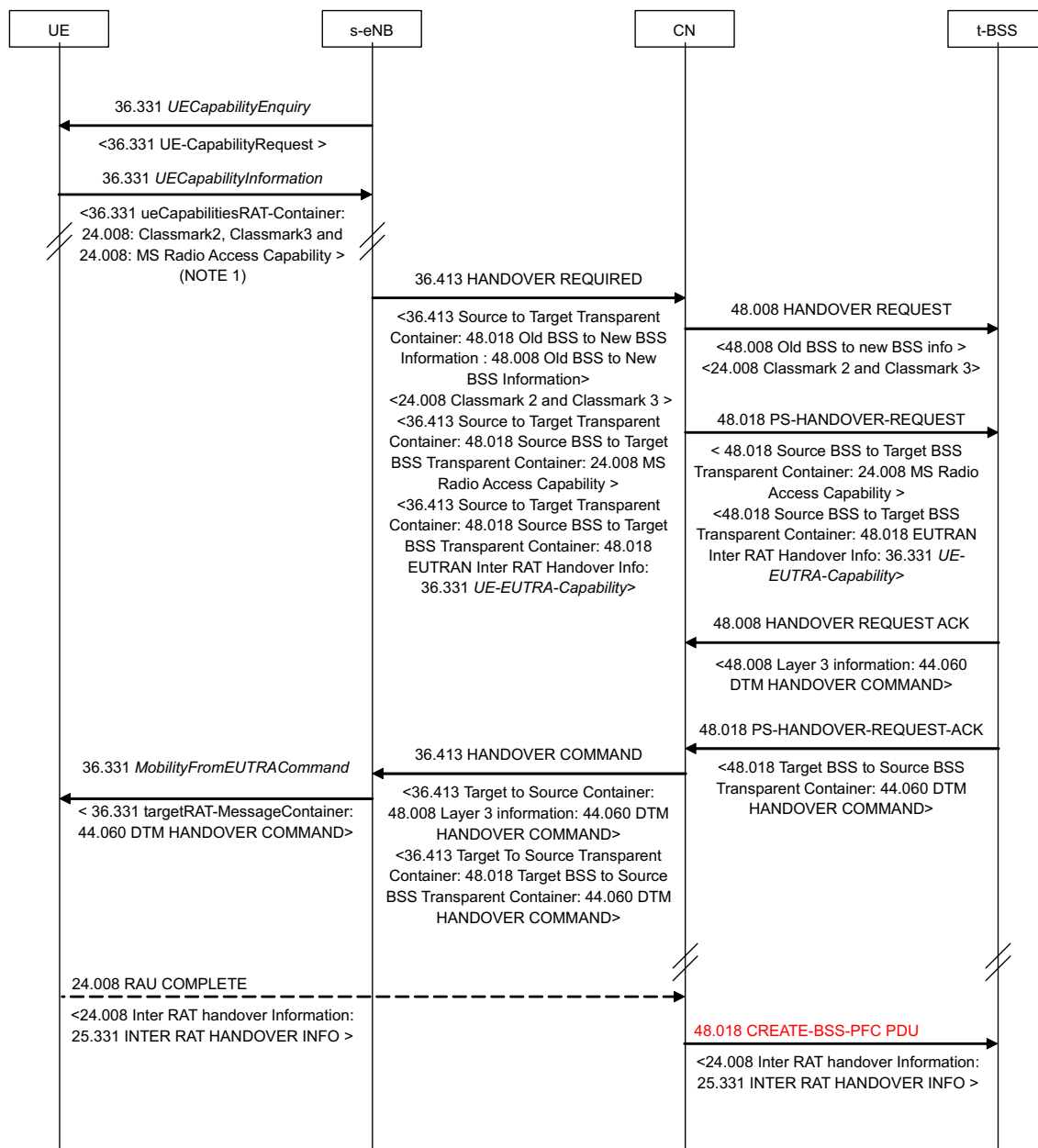
Figure 19.2.2.5.6-5: Handover of CS and PS domain services from EUTRAN to GERAN A/Gb mode, normal flow
