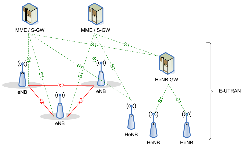
Figure 4.6.1-2: Overall E-UTRAN Architecture with deployed HeNB GW.
