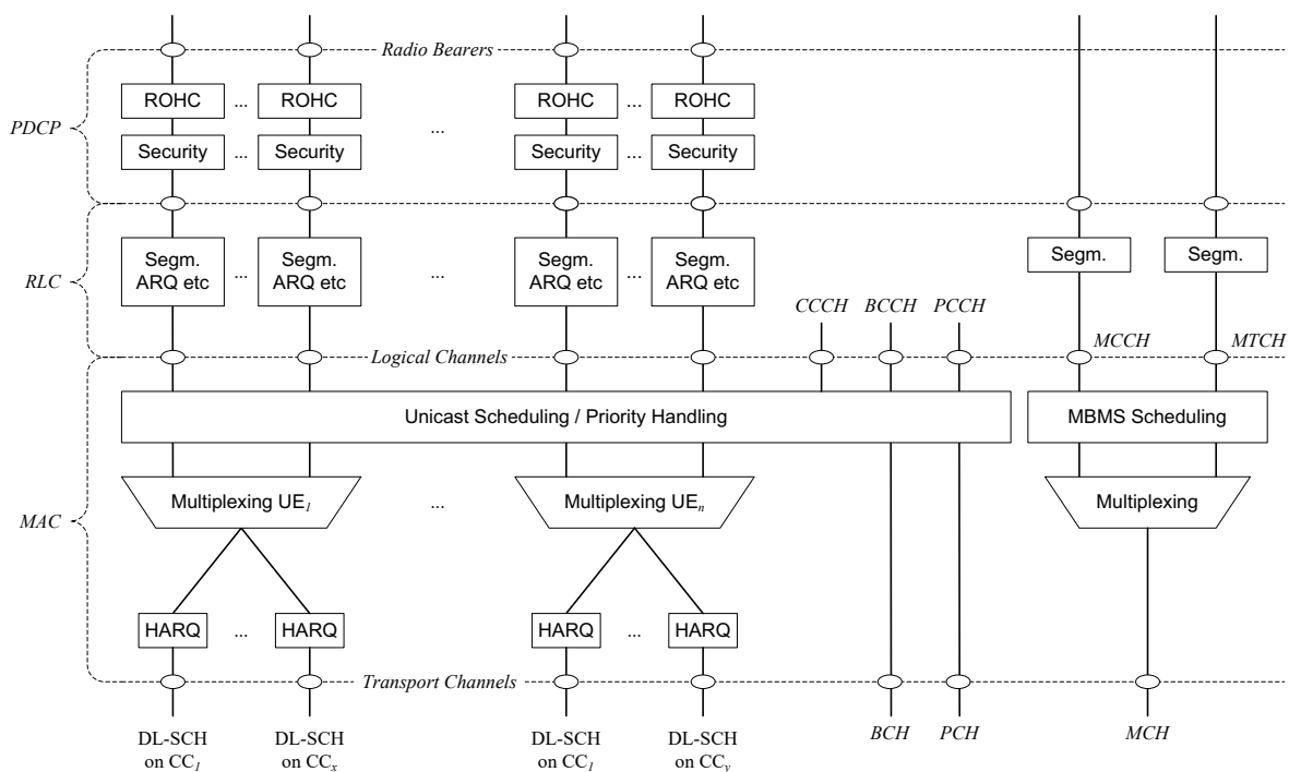
Figure 6.4-1: Layer 2 Structure for DL with CA configured
