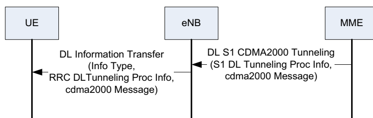
Figure 10.3.2.1-1: Downlink Direct Transfer
