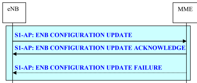
Figure 19.2.2.9-1: eNB Configuration Update procedure
