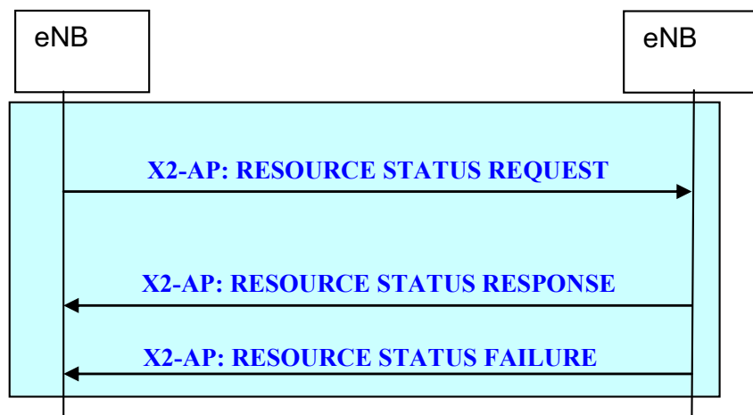
Figure 20.2.2.10-1: Resource Status Reporting Initiation procedure
