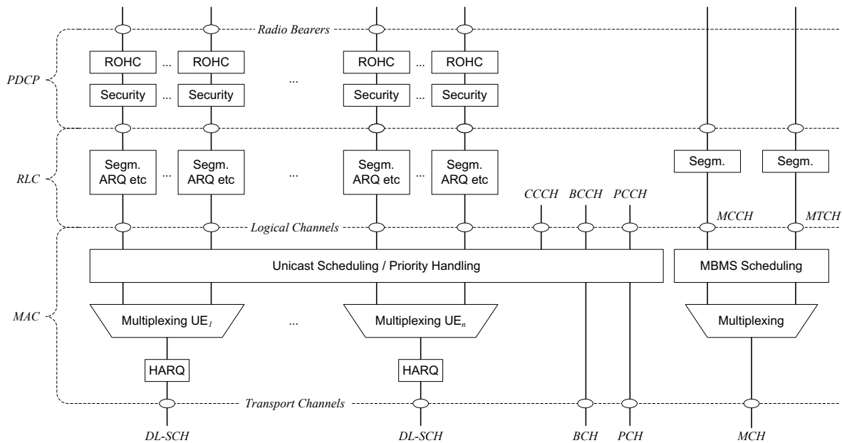
Figure 6-1: Layer 2 Structure for DL
