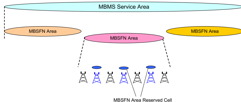
Figure 15-1: MBMS Definitions
