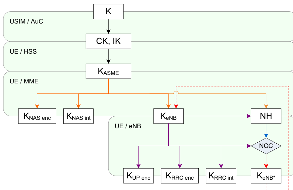
Figure 14.1-1: Key Derivation
