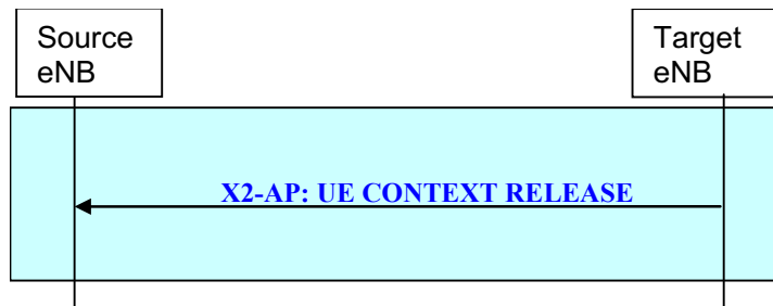
Figure 20.2.2.3-1: UE Context Release procedure
