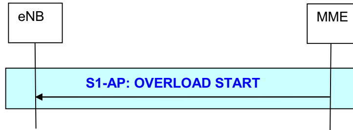
Figure 19.2.2.12.1-1 Overload Start procedure
