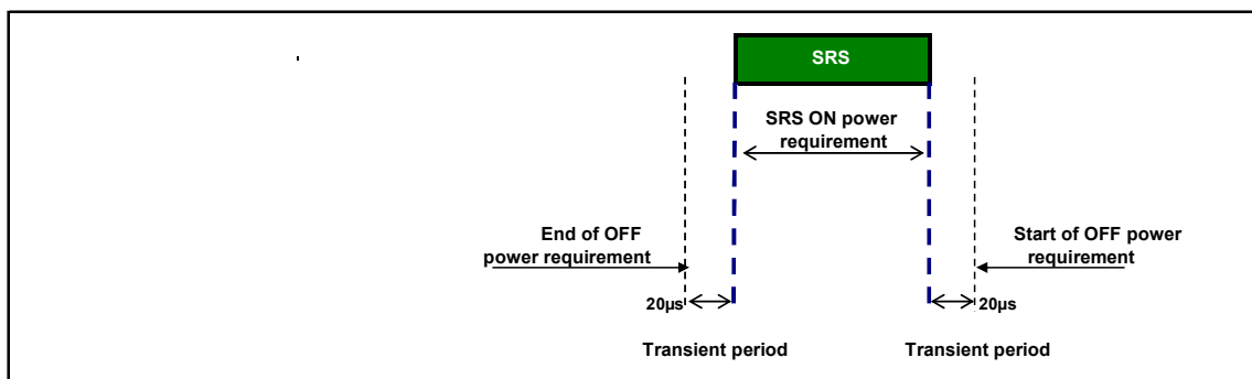
Figure 6.3.4.2.2-1: Single SRS time mask
