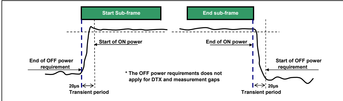
Figure 6.3.4.1-1: General ON/OFF time mask
