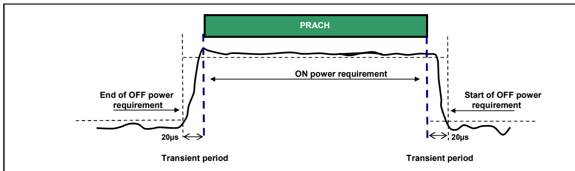
Figure 6.3.4.2-1: PRACH ON/OFF time mask
