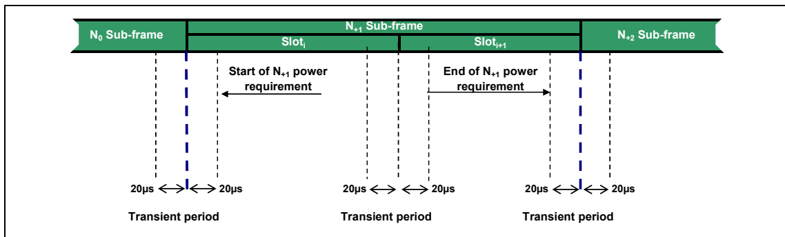
Figure 6.3.4.3-1: Transmission power template
