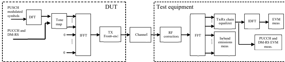
Figure F.1-1: EVM measurement points
