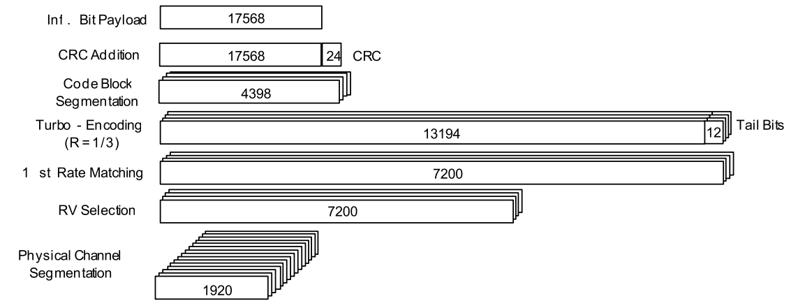
Figure A.27: Coding rate for Fixed Reference Channel H-Set 11 Secondary Transport Block
