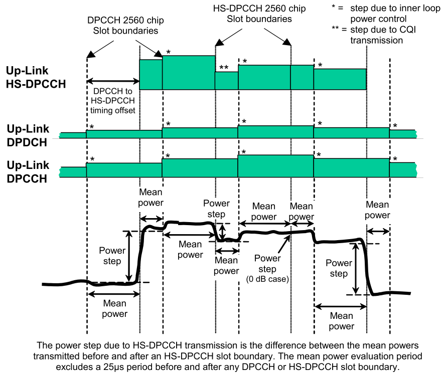
Figure 6.6: Transmit power template during HS-DPCCH transmission
