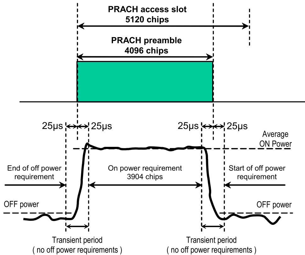
Figure 6.2: Transmit ON/OFF template for PRACH preambles
