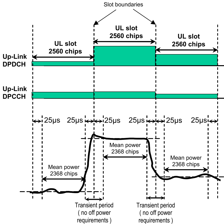
Figure 6.4: Transmit template during TFC change
