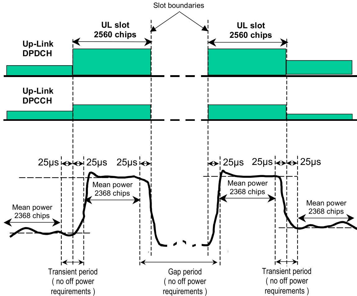
Figure 6.5: Transmit template during compressed mode
